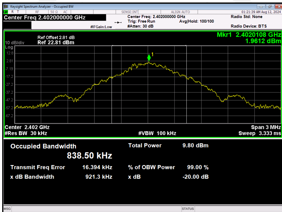
99%_Occupied_Bandwidth_NVNT_ANT1_1-DH1_2402_00
