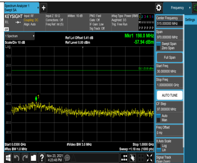
Band7-5MHz-16QAM-21100-25RB#0-Range1:30~1000MHz
