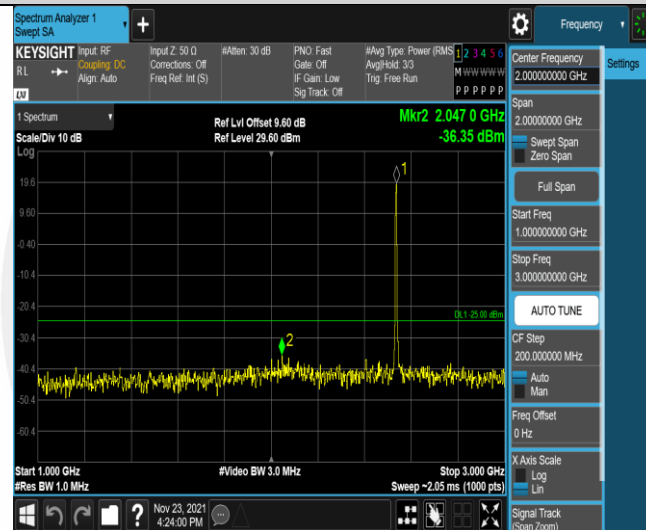
Band7-5MHz-16QAM-21100-25RB#0-Range2:1000~3000MHz
