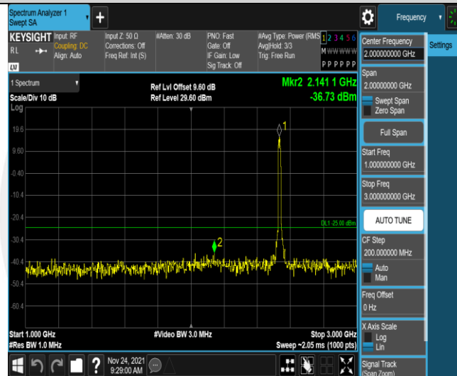
Band7-15MHz-QPSK-21100-75RB#0-Range2:1000~3000MHz
