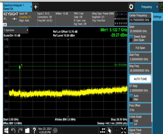
Band7-5MHz-16QAM-21425-25RB#0-Range3:3000~26500MHz
