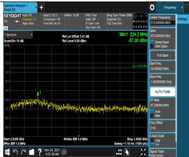
Band7-15MHz-QPSK-20825-75RB#0-Range1:30~1000MHz
