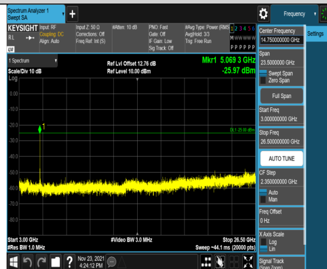
Band7-5MHz-16QAM-21100-25RB#0-Range3:3000~26500MHz
