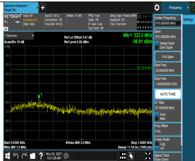
Band7-10MHz-16QAM-20800-50RB#0-Range1:30~1000MHz
