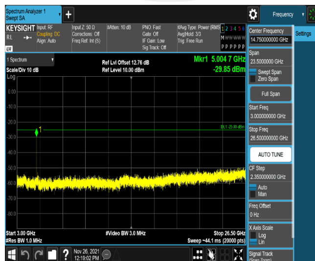
Band7-10MHz-16QAM-21100-50RB#0-Range3:3000~26500MHz
