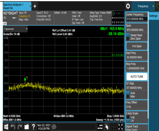
Band7-5MHz-QPSK-21425-25RB#0-Range1:30~1000MHz
