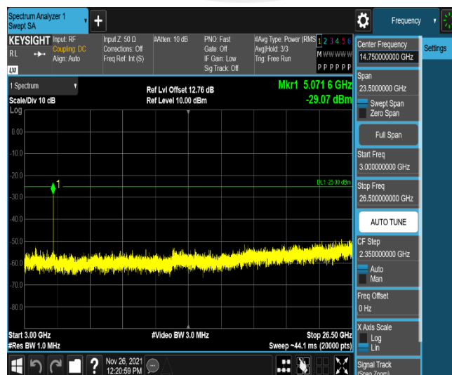
Band7-10MHz-16QAM-21400-50RB#0-Range3:3000~26500MHz
