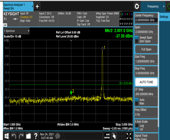
Band7-15MHz-QPSK-20825-75RB#0-Range2:1000~3000MHz
