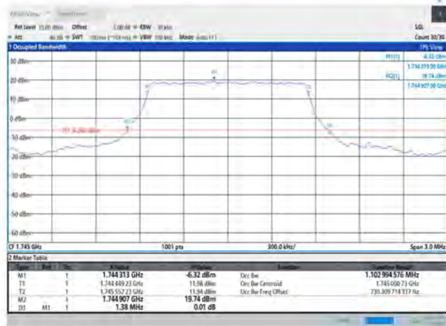
Band66-1.4MHz-QPSK-132322-6RB#0
