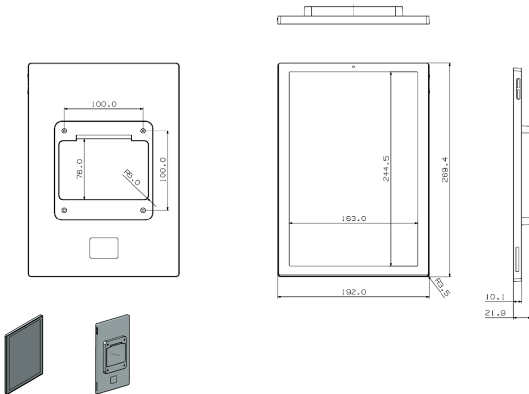
Figure 10 11.6" Mechanical Dimension
