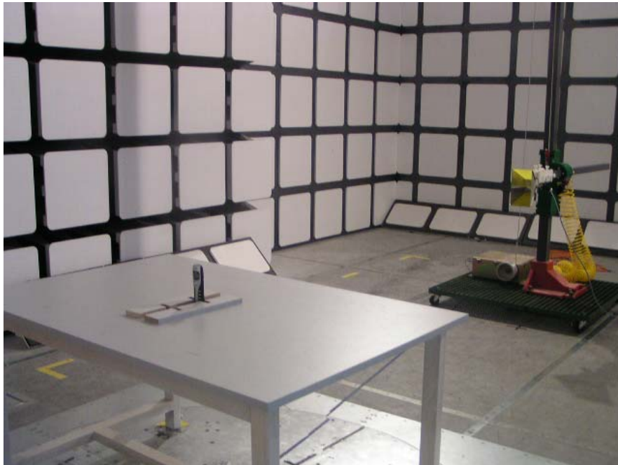
Handset: Radiated Emission - Front View (Above 1 GHz)
