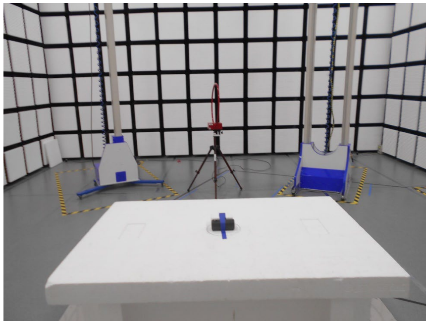
RADIATED BELOW 30MHz 90 DEG
