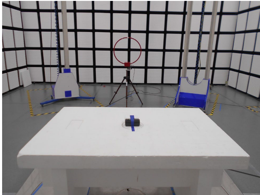
RADIATED BELOW 30MHz 0 DEG
