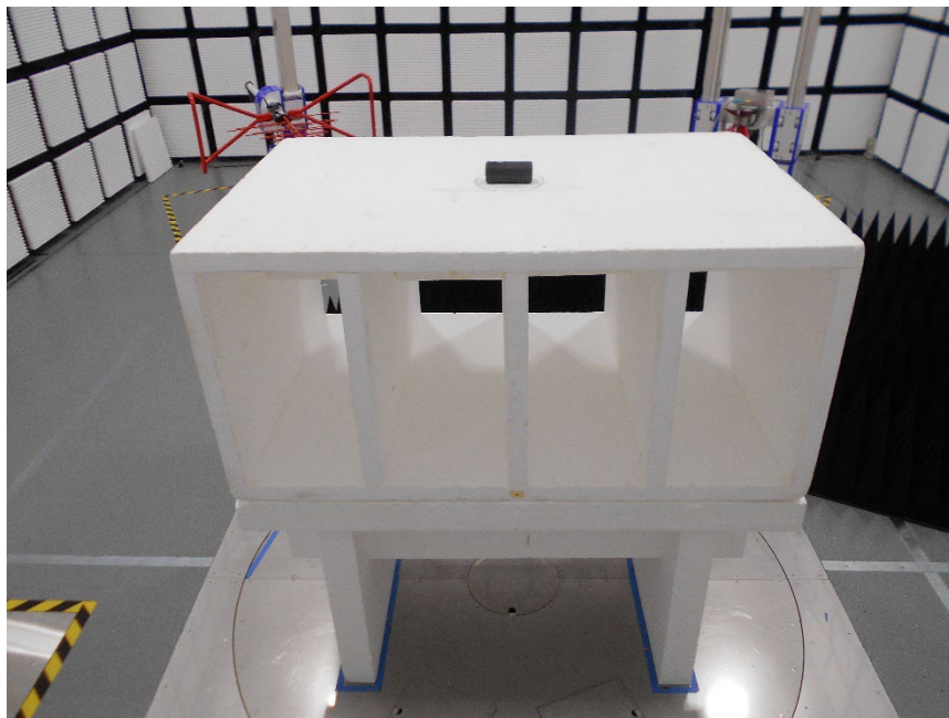
RADIATED ABOVE 1GHz BACK
