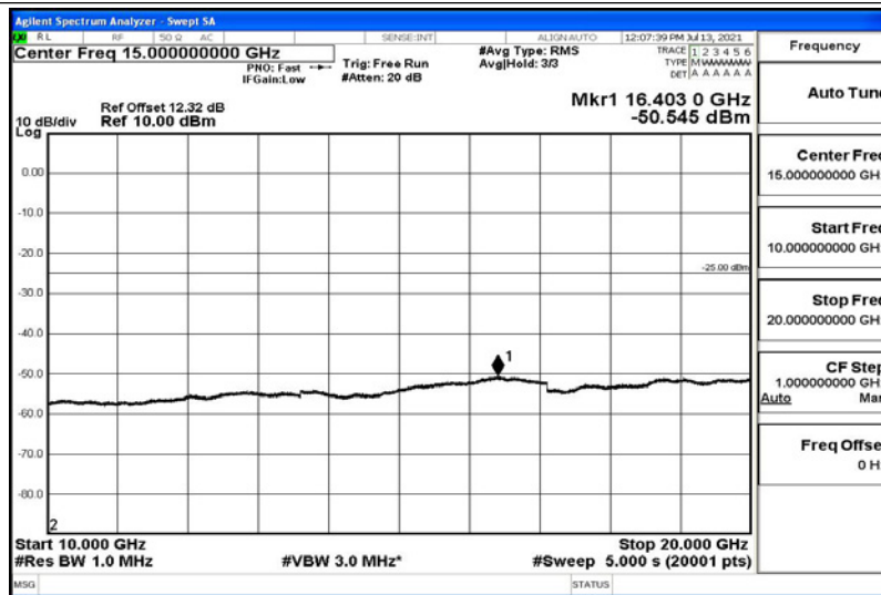
Band7-5MHz-QPSK-21425-1RB#0-Range6:20000~26500MHz
