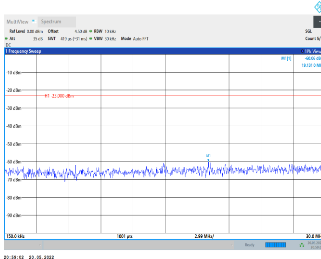
Band26-15MHz-QPSK-26865-1RB#0-Range2:0.15~30MHz
