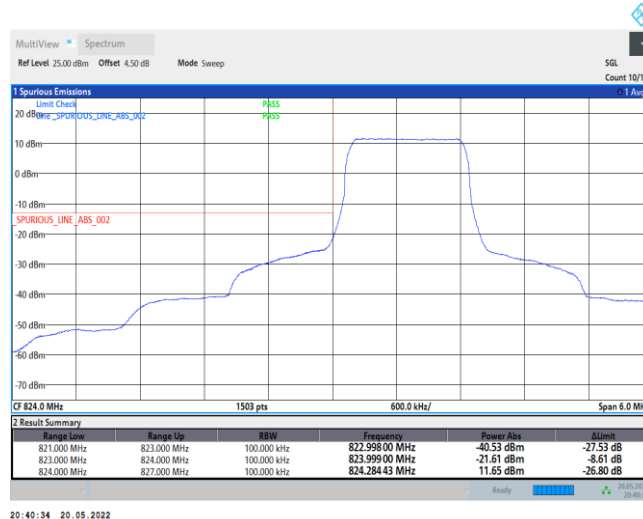
Band26-1.4MHz-QPSK-26797-6RB#0
