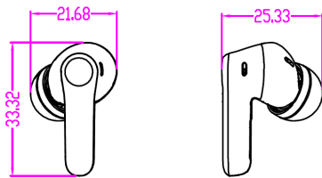
Bluetooth headset
