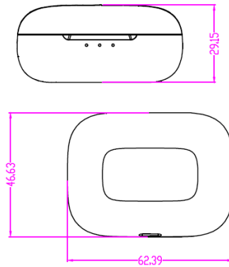
Charging box
