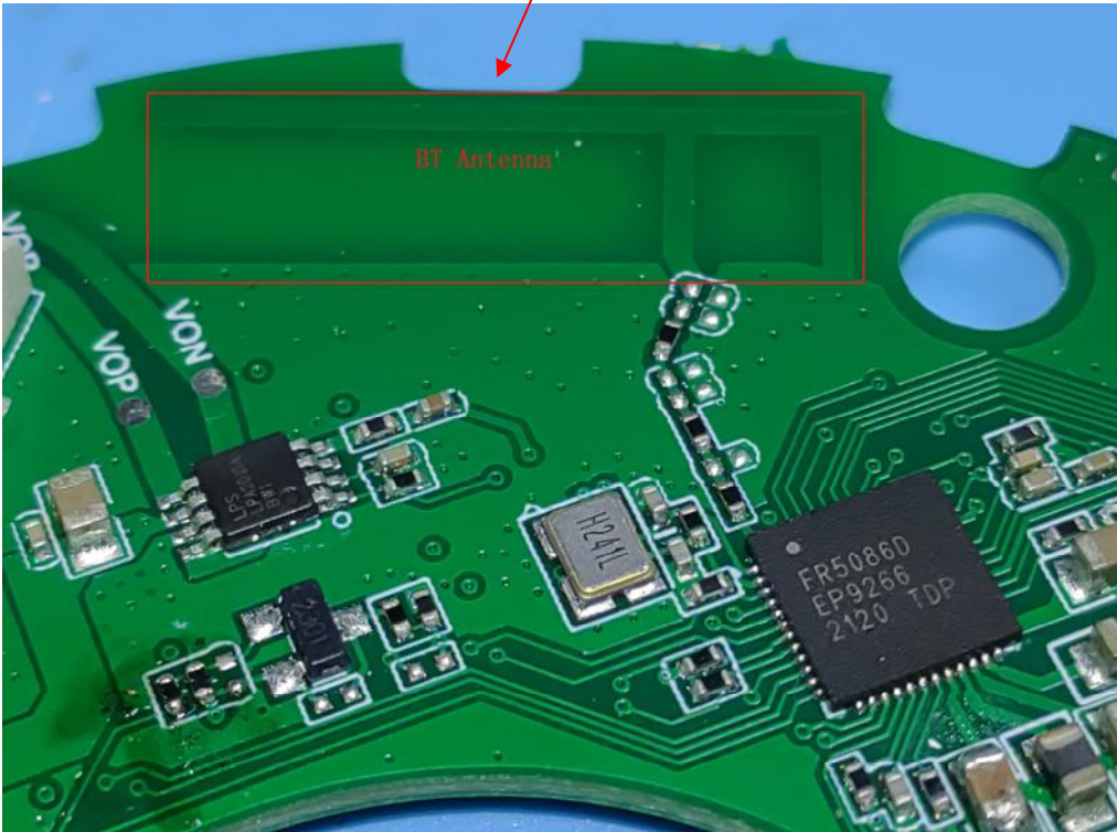
BT/BLE Antenna
