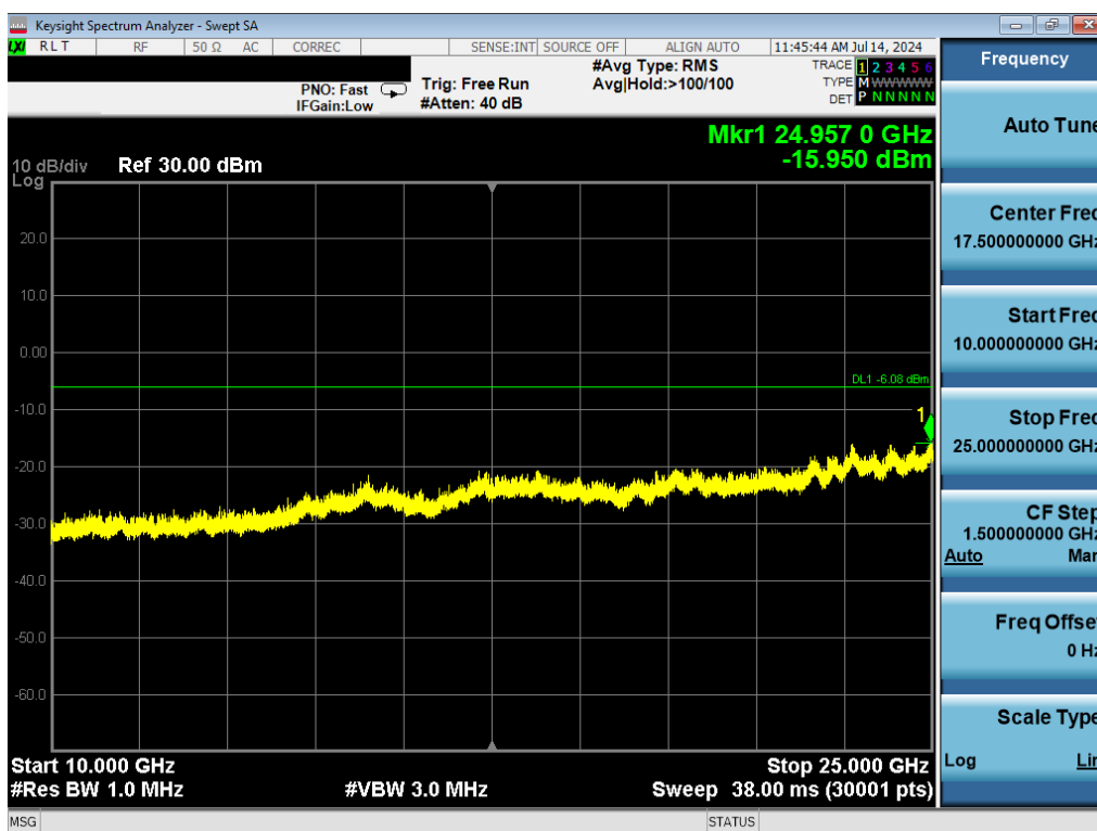
Plot 7-28. Conducted Spurious Plot (Bluetooth (HDR4), ePA – Ch. 73)
