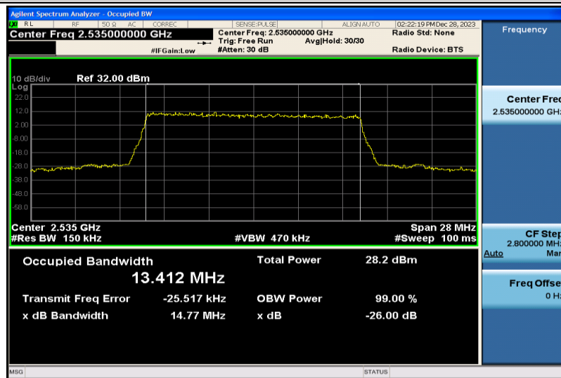
Band7-15MHz-QPSK-21100-75RB#0-13.412
