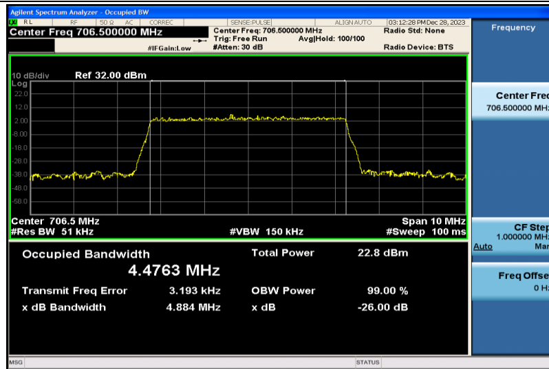
Band17-5MHz-16QAM-23755-25RB#0-4.4763
