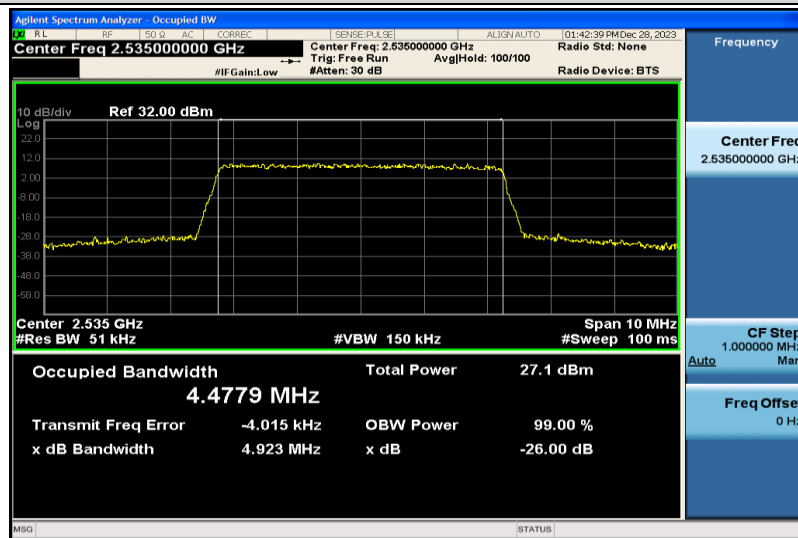
Band7-5MHz-16QAM-21100-25RB#0-4.4779
