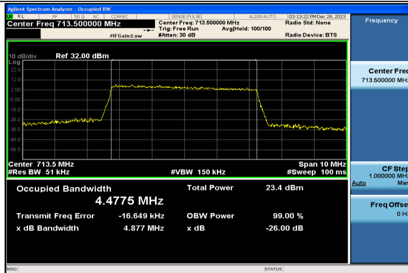
Band17-5MHz-QPSK-23825-25RB#0-4.4775
