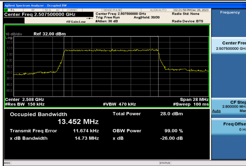
Band7-15MHz-QPSK-20825-75RB#0-13.452
