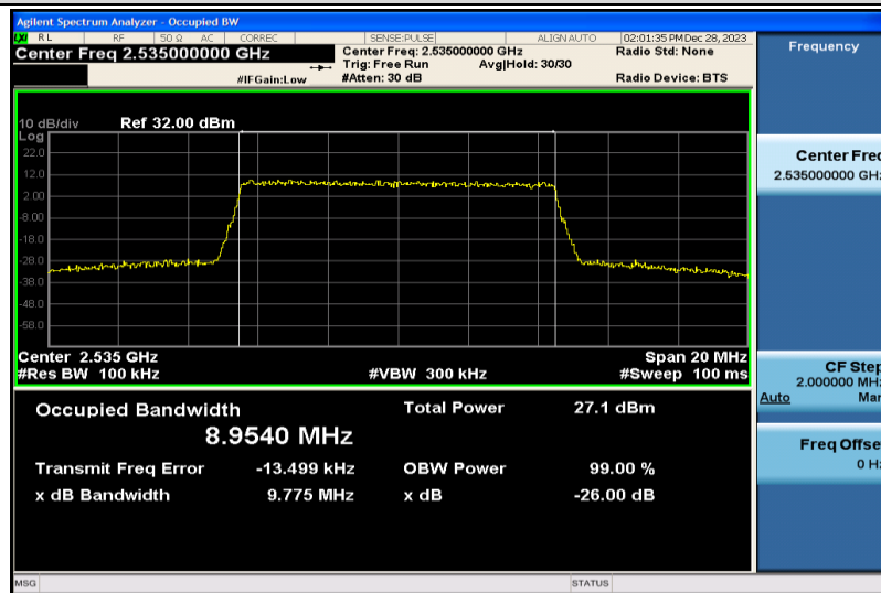
Band7-10MHz-16QAM-21100-50RB#0-8.9540
