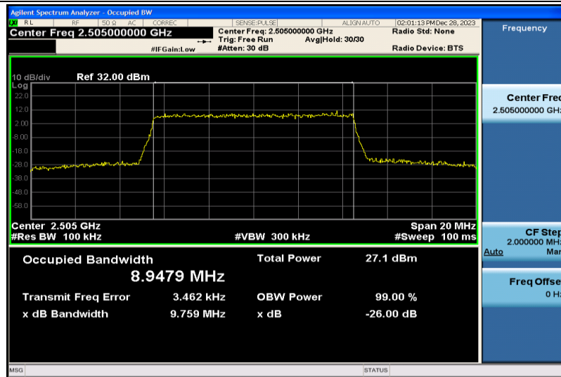
Band7-10MHz-16QAM-20800-50RB#0-8.9479
