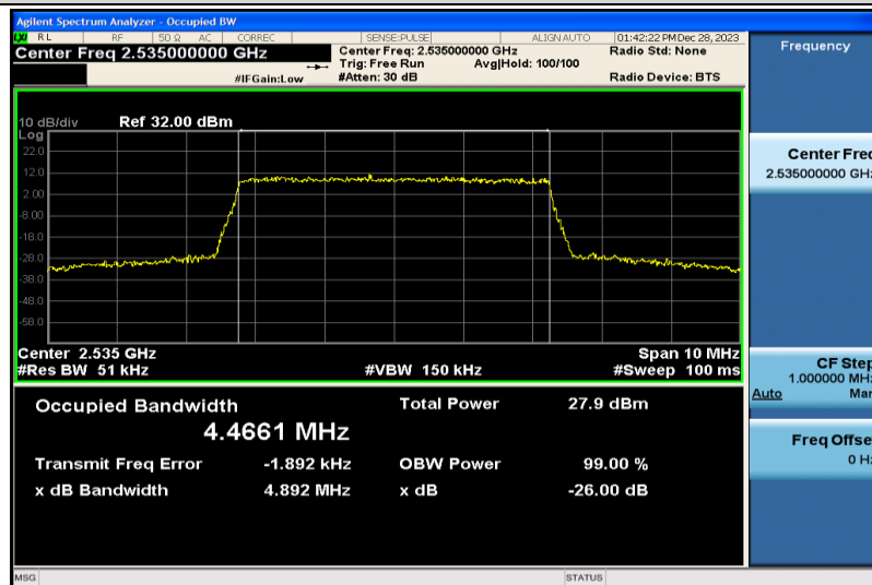
Band7-5MHz-QPSK-21100-25RB#0-4.4661
