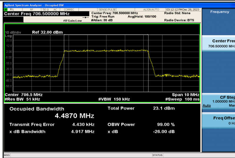
Band17-5MHz-QPSK-23755-25RB#0-4.4870
