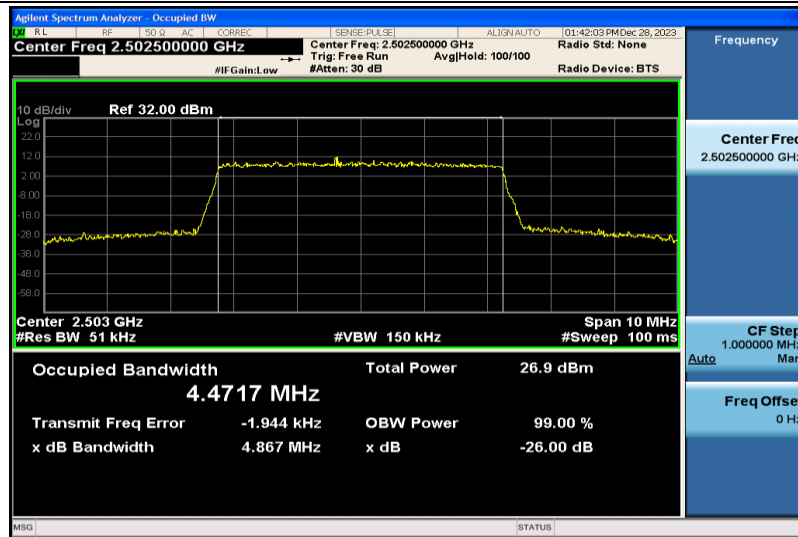
Band7-5MHz-16QAM-20775-25RB#0-4.4717
