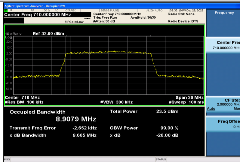
Band17-10MHz-16QAM-23790-50RB#0-8.9079
