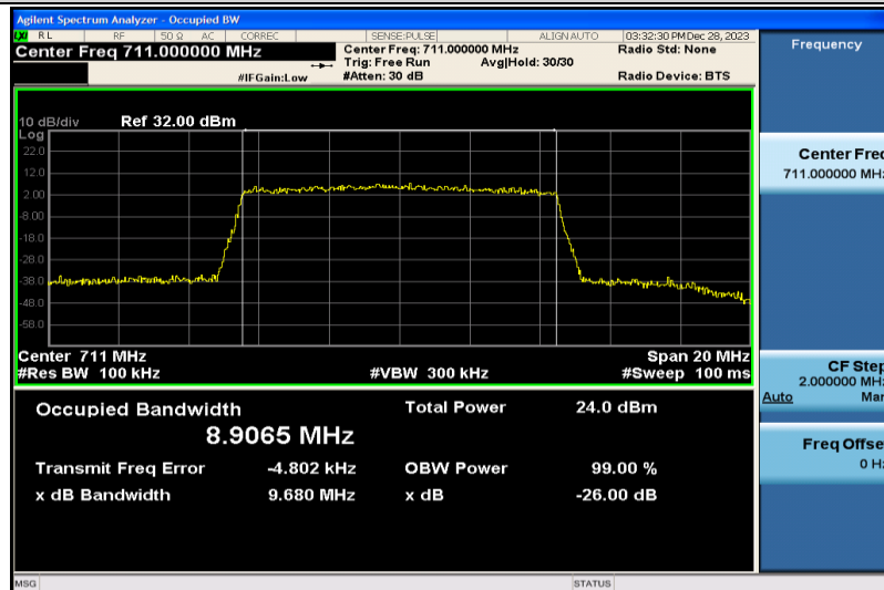
Band17-10MHz-QPSK-23800-50RB#0-8.9065
