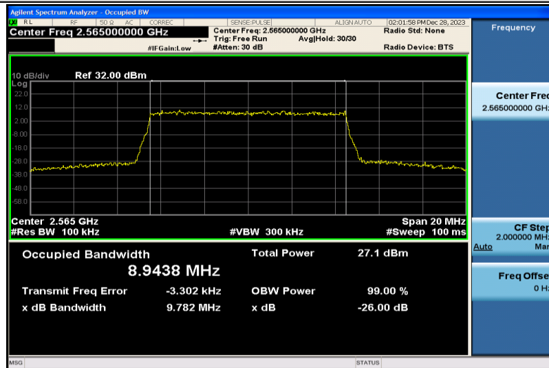
Band7-10MHz-16QAM-21400-50RB#0-8.9438
