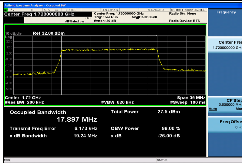
Band4-20MHz-QPSK-20050-100RB#0-17.897
