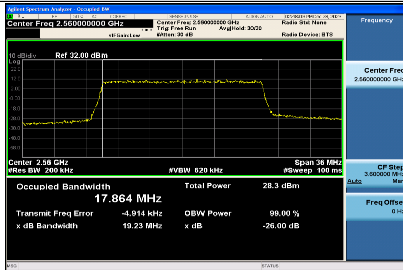
Band7-20MHz-QPSK-21350-100RB#0-17.864
