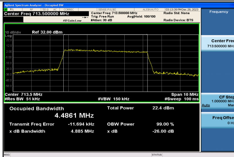
Band17-5MHz-16QAM-23825-25RB#0-4.4861
