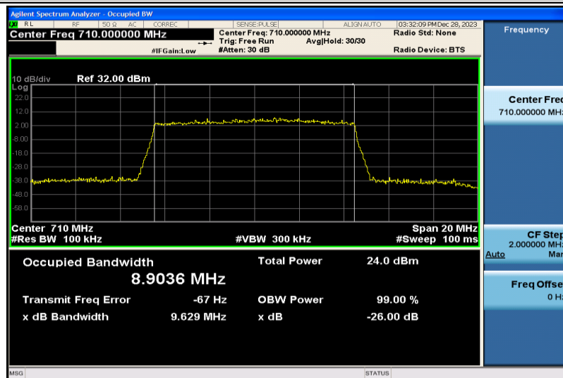
Band17-10MHz-QPSK-23790-50RB#0-8.9036
