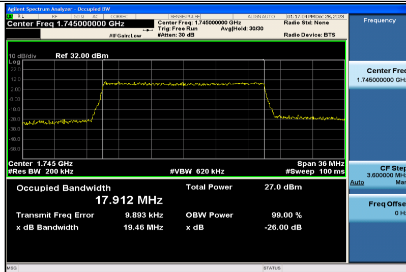
Band4-20MHz-16QAM-20300-100RB#0-17.912
