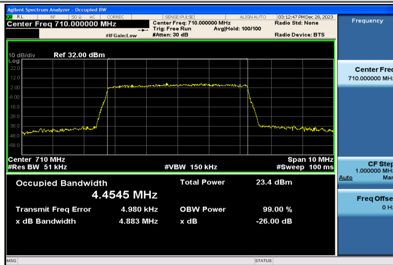
Band17-5MHz-QPSK-23790-25RB#0-4.4545
