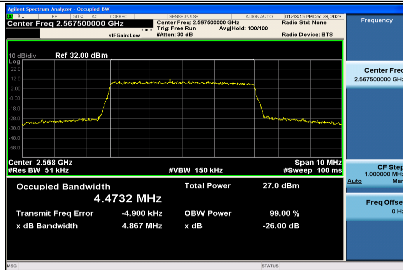
Band7-5MHz-16QAM-21425-25RB#0-4.4732
