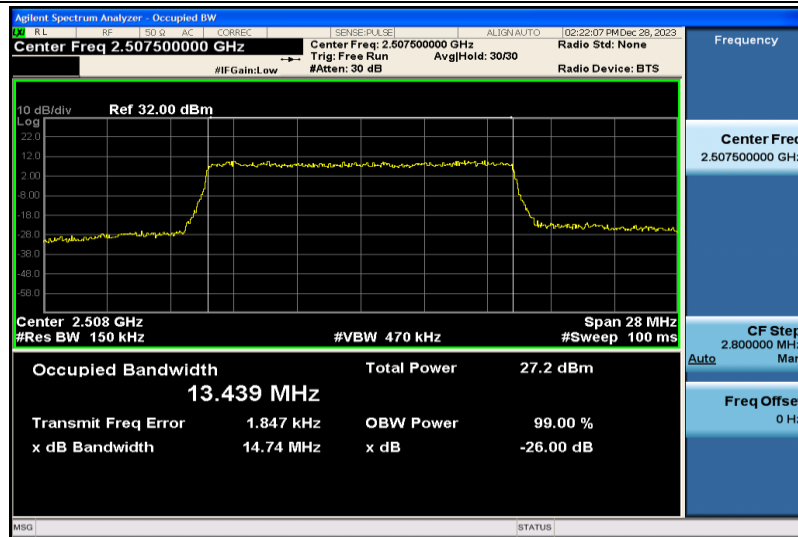
Band7-15MHz-16QAM-20825-75RB#0-13.439
