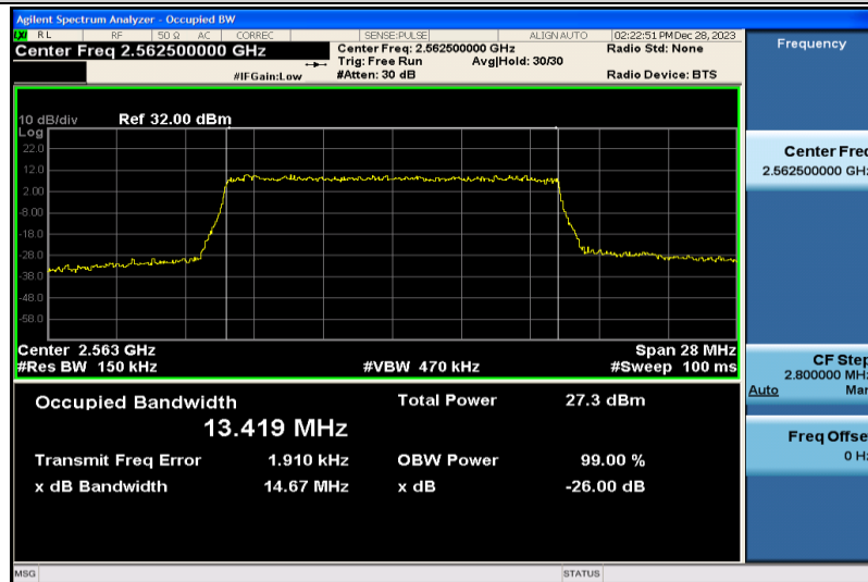
Band7-15MHz-16QAM-21375-75RB#0-13.419
