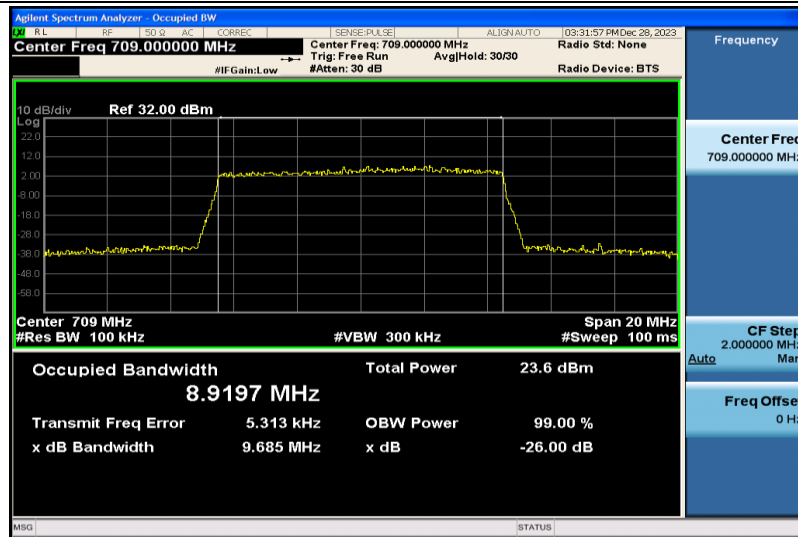
Band17-10MHz-16QAM-23780-50RB#0-8.9197
