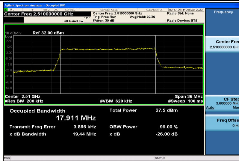
Band7-20MHz-16QAM-20850-100RB#0-17.911
