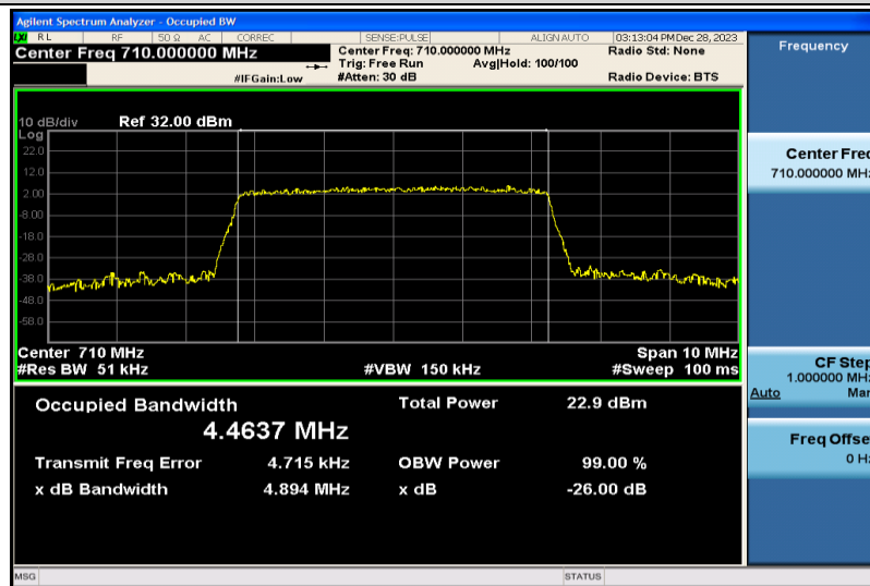
Band17-5MHz-16QAM-23790-25RB#0-4.4637
