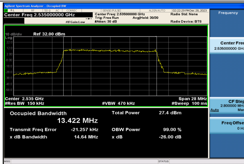
Band7-15MHz-16QAM-21100-75RB#0-13.422
