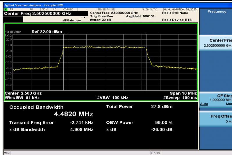
Band7-5MHz-QPSK-20775-25RB#0-4.4820
