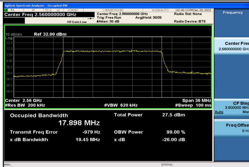
Band7-20MHz-16QAM-21350-100RB#0-17.898
