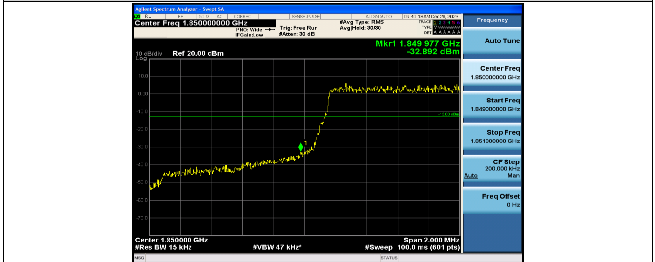
Band2-1.4MHz-QPSK-18607-1RB#0
