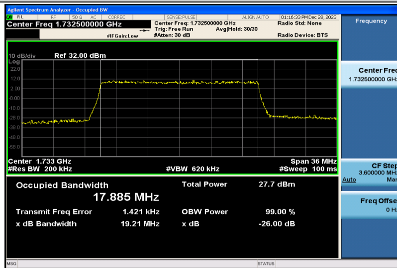
Band4-20MHz-QPSK-20175-100RB#0-17.885
