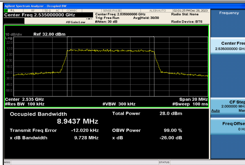
Band7-10MHz-QPSK-21100-50RB#0-8.9437
