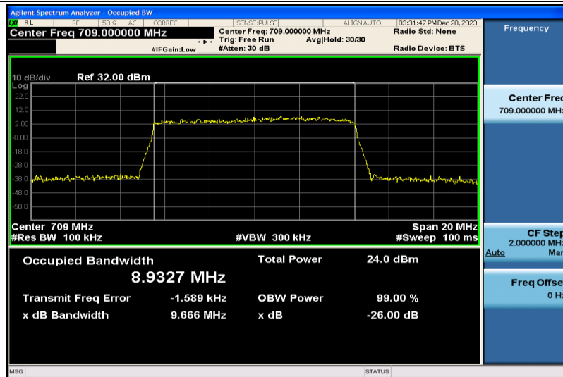
Band17-10MHz-QPSK-23780-50RB#0-8.9327
