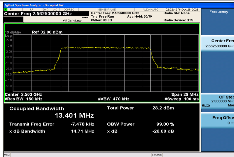
Band7-15MHz-QPSK-21375-75RB#0-13.401
