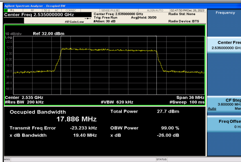
Band7-20MHz-16QAM-21100-100RB#0-17.886
