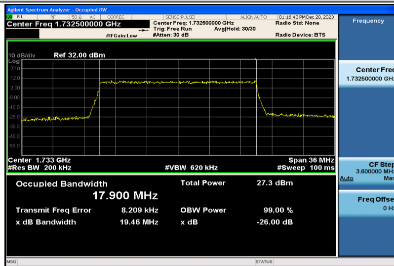
Band4-20MHz-16QAM-20175-100RB#0-17.900
