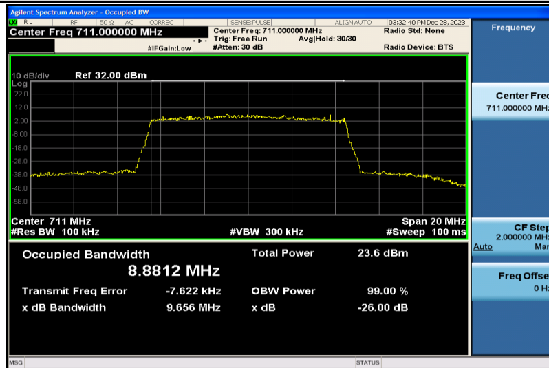
Band17-10MHz-16QAM-23800-50RB#0-8.8812
