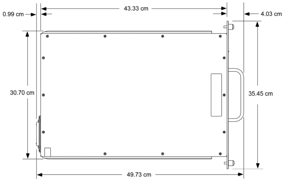
Figure 1-3. Model G3L-850-135 Amplifier Side View
