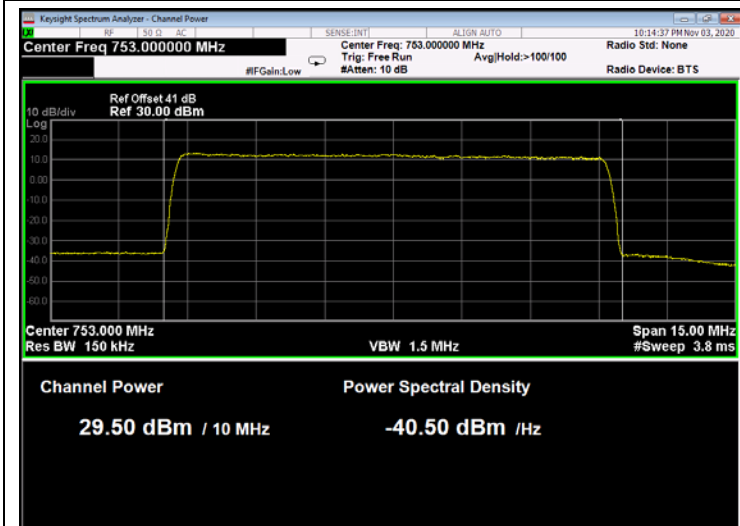
Figure 53: 64QAM 10MHz B.W.; 753.0MHz, 15kHz
