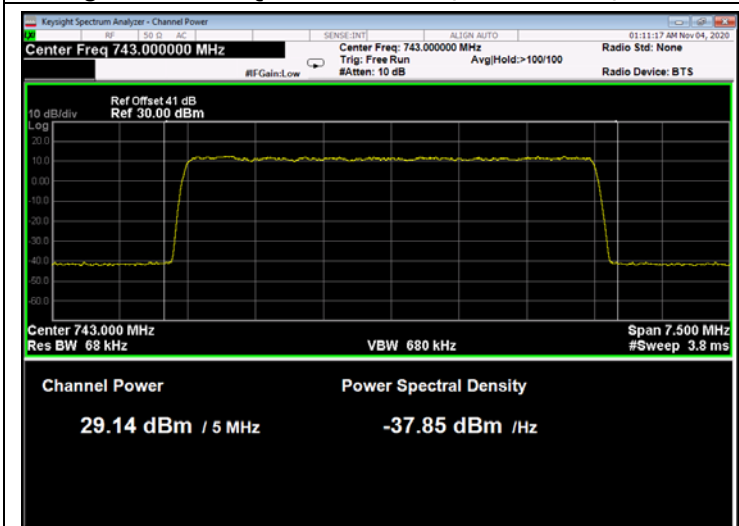
Figure 76: 256QAM 5MHz B.W.; 743.0MHz, 15kHz
