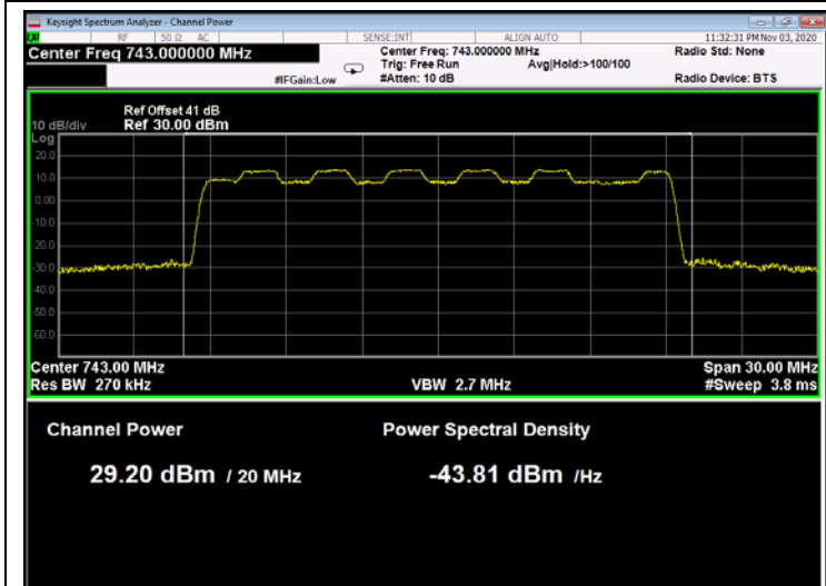
Figure 36: 16QAM 20MHz B.W.; 743.0MHz, 30kHz
