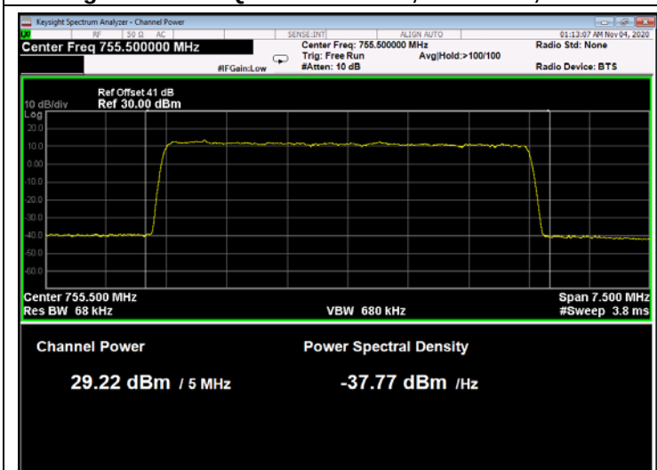
Figure 78: 256QAM 5MHz B.W.; 755.5MHz, 15kHz
