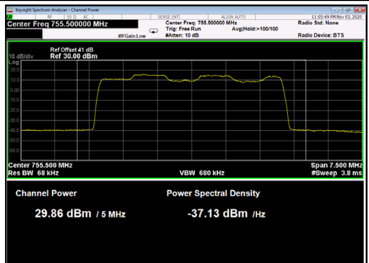
Figure 13: 16QAM 5MHz; 755.5MHz, 30kHz
