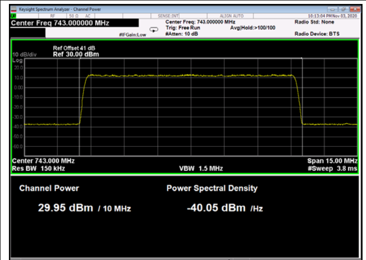
Figure 50: 64QAM 10MHz B.W.; 743.0MHz, 15kHz
