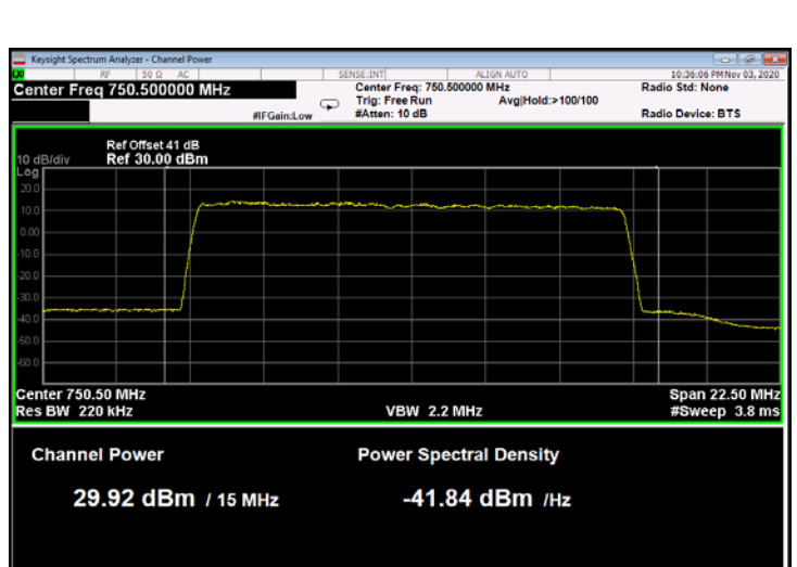
Figure 64: 64QAM 15MHz B.W.; 750.5MHz, 60kHz
