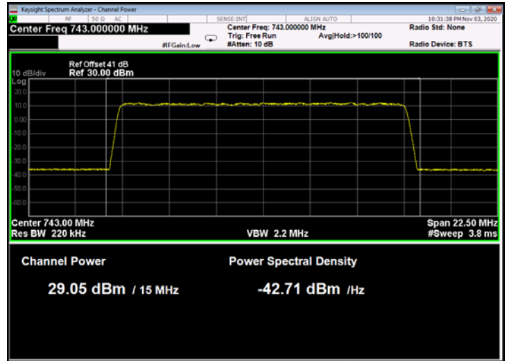
Figure 60: 64QAM 15MHz B.W.; 743.0MHz, 30kHz
