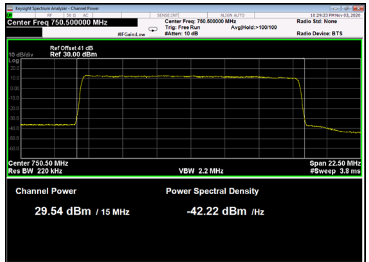
Figure 62: 64QAM 15MHz B.W.; 750.5MHz, 15kHz
