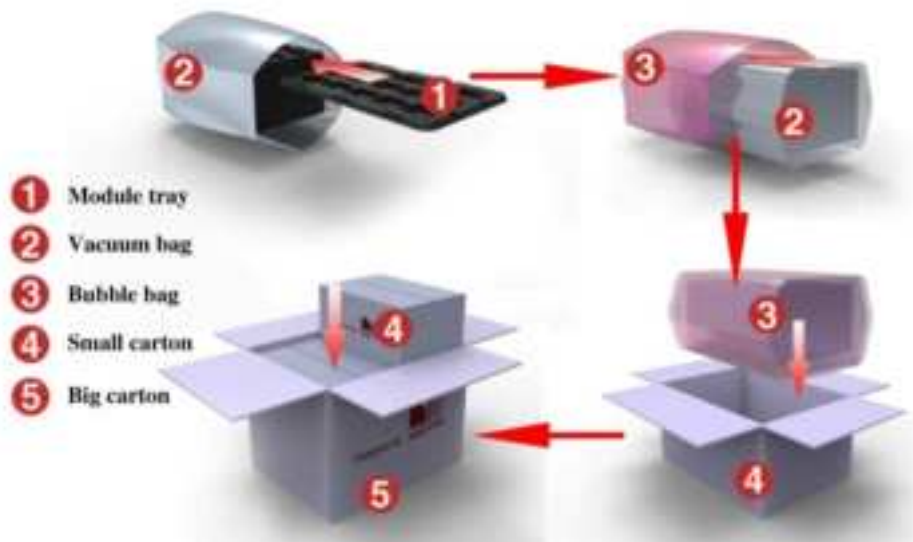
Figure 36: Packaging diagram
