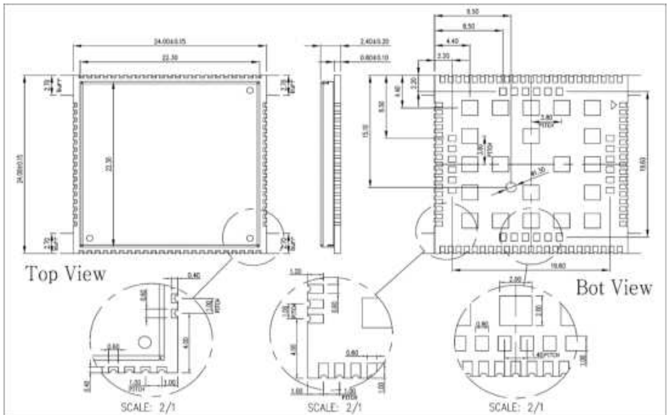
Figure 2: Dimensions (Unit: mm)
