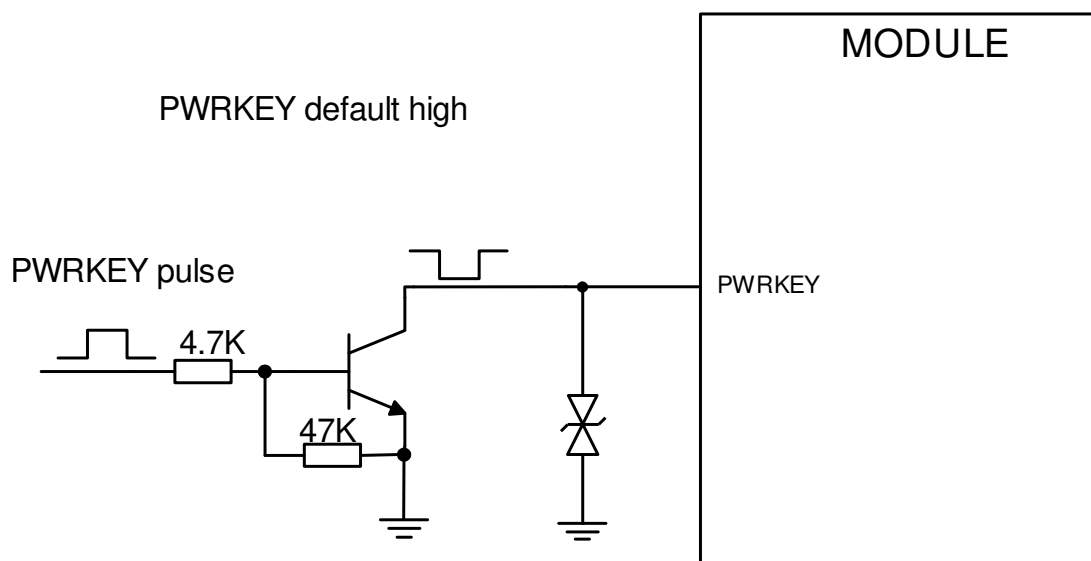
Figure 8: Reference power on/off circuit
