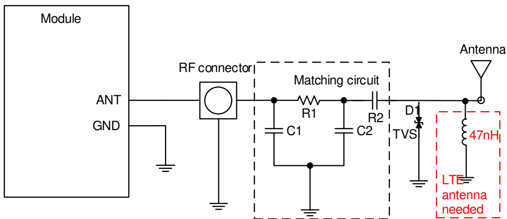
Figure 29: Passive antenna reference
