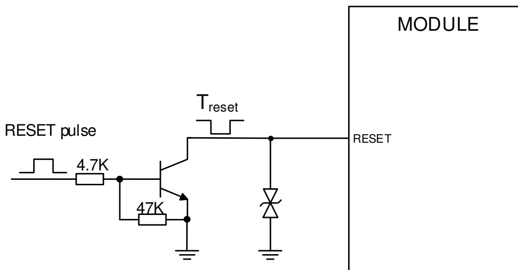
Figure 11: Reference reset circuit
