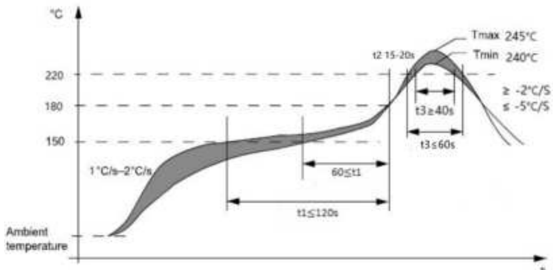
Figure 34: Recommended reflow furnace temperature curve (lead-free)
