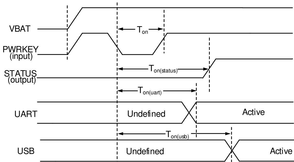
Figure 9: Power on sequence
