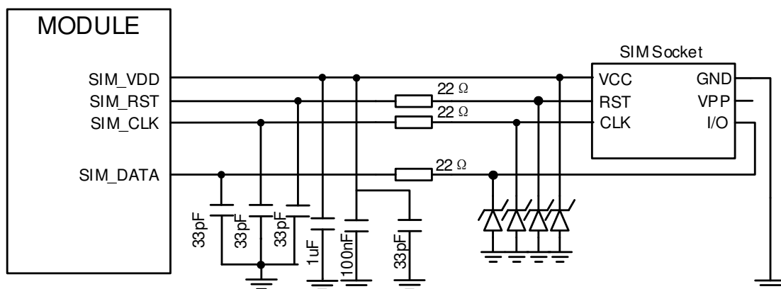
Figure 19: SIM interface reference circuit
