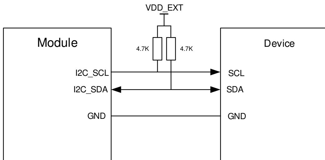
Figure 21: I2C reference circuit
