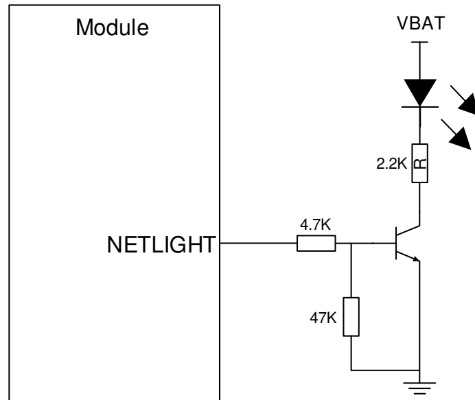
Figure 23: NETLIGHT reference circuit
