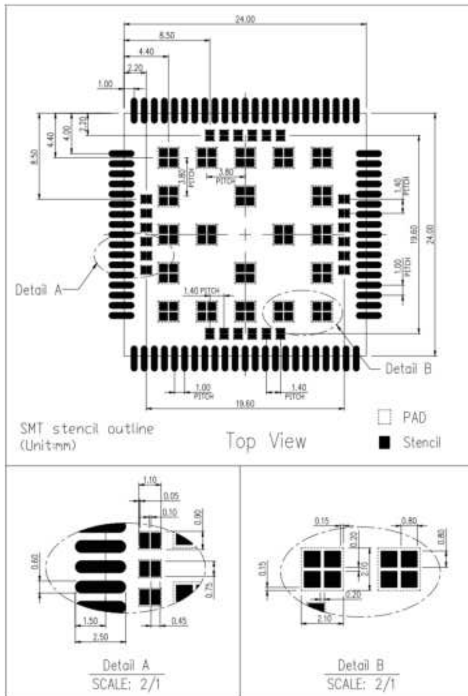
Figure 4: Recommend stencil dimension (Unit: mm)
