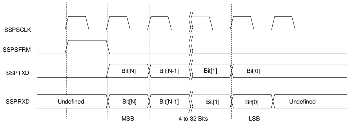
Figure 26: PCM sequence
