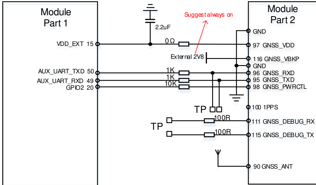
Figure 24: GNSS reference design (Non-standalone GNSS solution)
