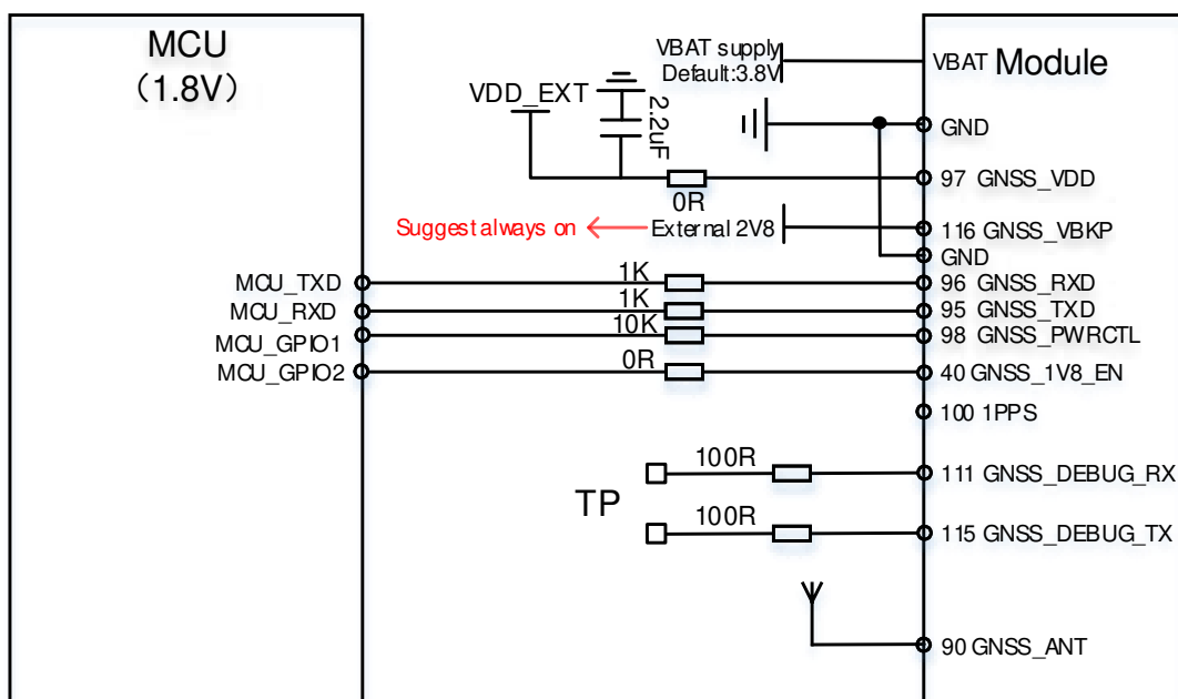
Figure 25: GNSS reference design (Standalone GNSS solution)
