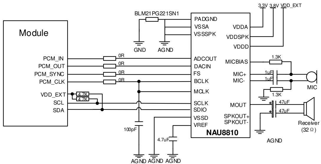
Figure 27: PCM reference design
