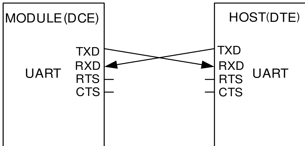
Figure 13: Serial port connection diagram (NULL mode)
