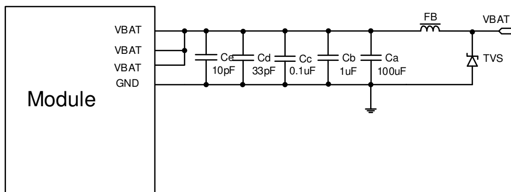
Figure 5: Power supply application circuit
