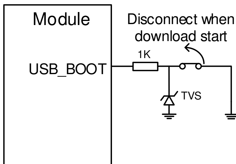
Figure 17: Reference USB_BOOT circuit
