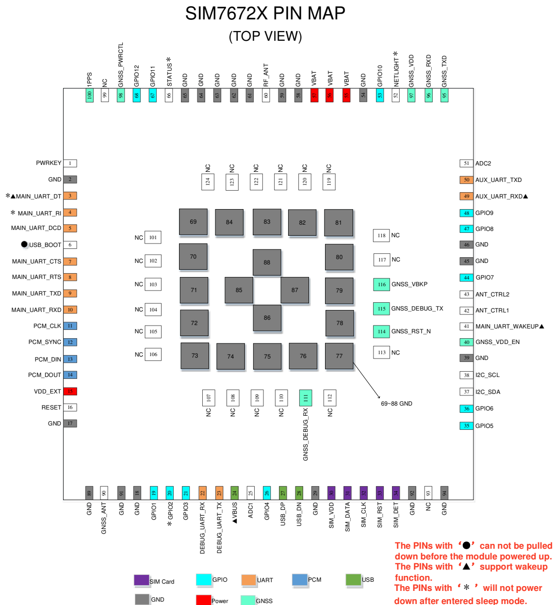
Figure 1: Pin assignment overview for SIM7672X
