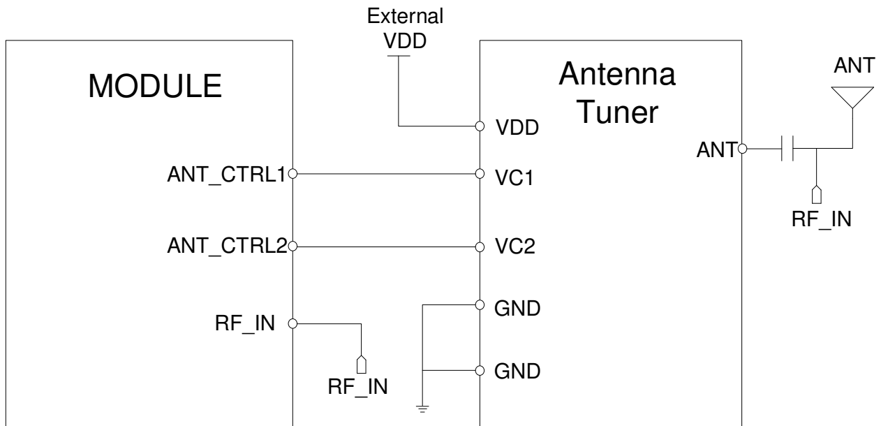
Figure 28: RF control interface reference circuit
