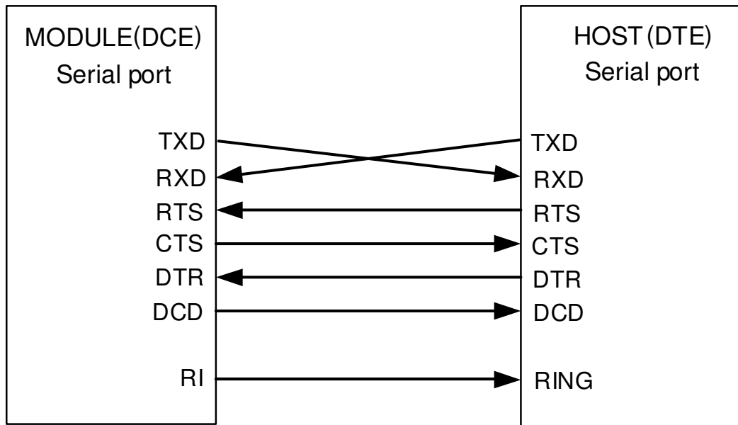
Figure 12: Serial port connection diagram (full-function mode)
