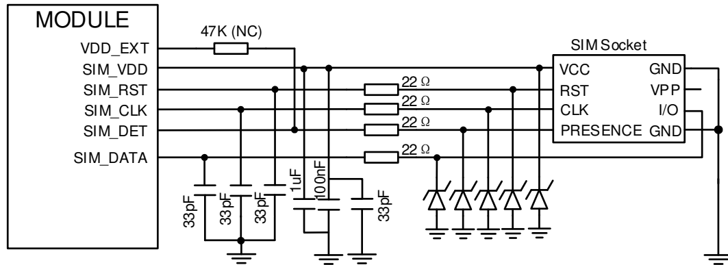
Figure 20: SIM interface reference circuit (8PIN)
