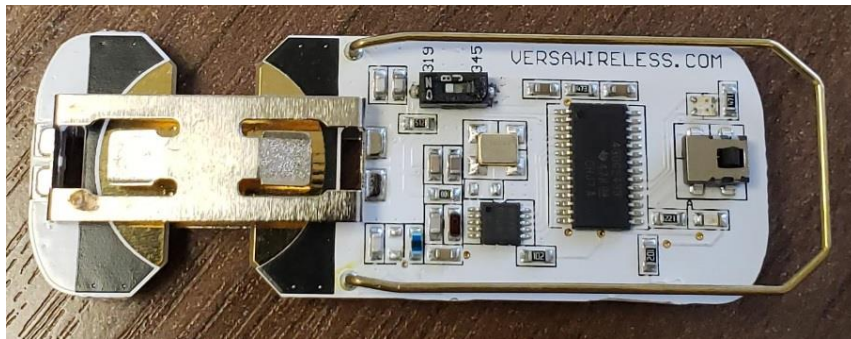
VERSAHP Top Side of PCB
