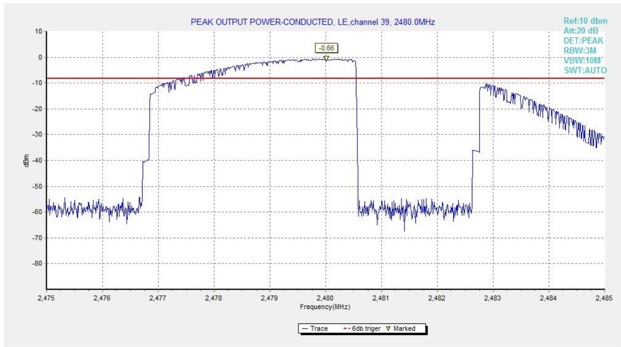
Fig.3 RF output power (Ch 39)
