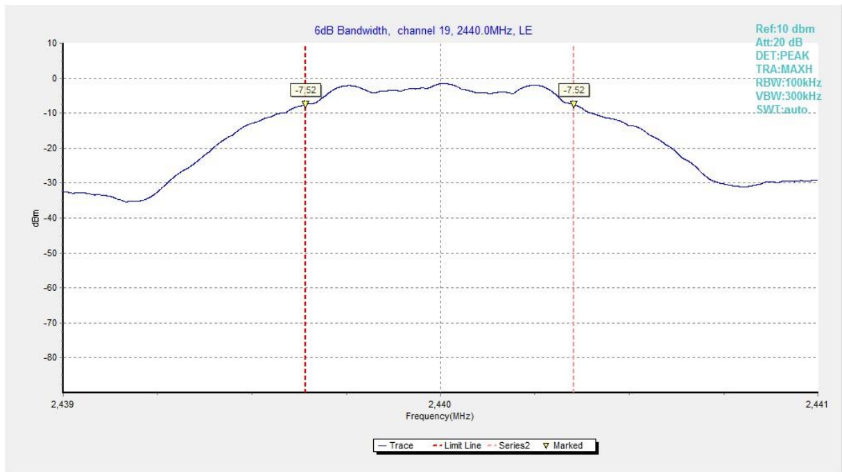
Fig.8 6dB Bandwidth (Ch 19)
