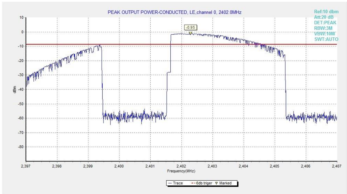
Fig.1 RF output power (Ch 0)
