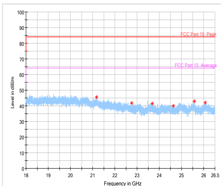
Fig 88. Radiated emission: GFSK, 18 GHz – 26.5 GHz
