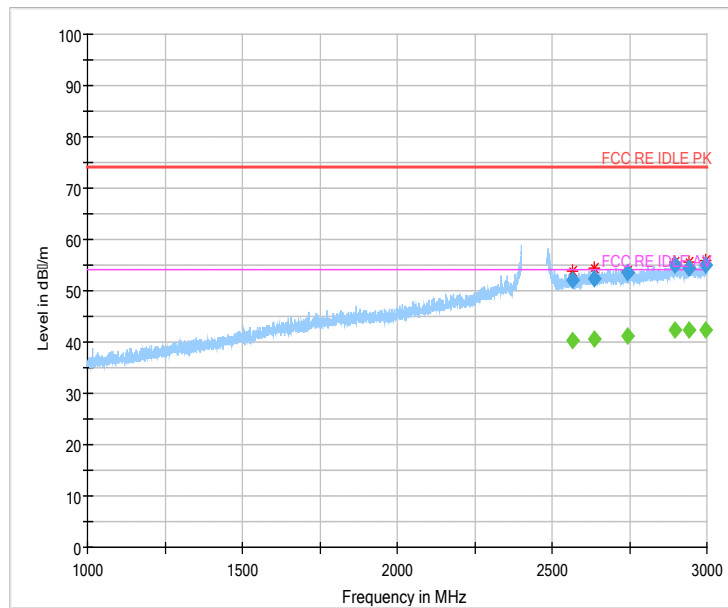
Fig 65. Radiated Spurious Emission (802.11g,Ch6,1GHz~3GHz)
