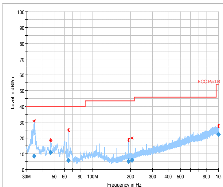
Fig 85. Radiated Spurious Emission (802.11 n-20MHz,Ch1,30MHz~1GHz)
