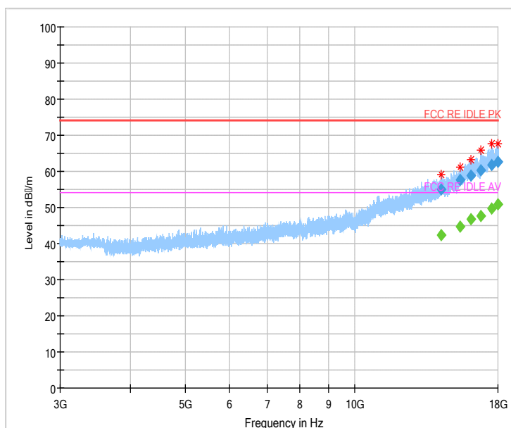
Fig 87. Radiated Spurious Emission (802.11 n-20MHz,Ch1,3GHz~18GHz)
