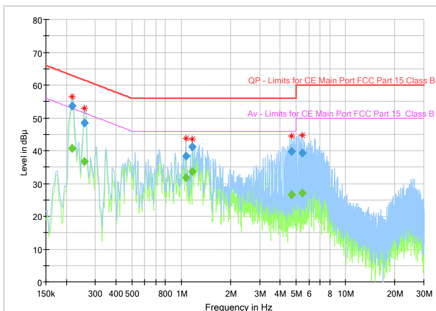
Fig 89. AC Conducted Emission
