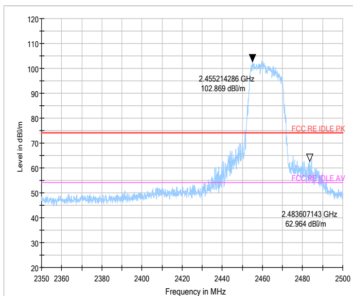
Fig 74. Radiated emission (Power): 802.11b, high channel
