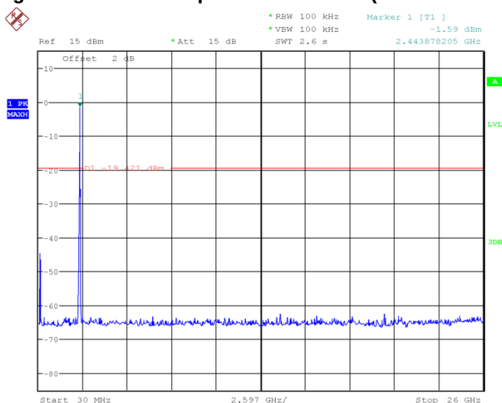
Fig 55. Conducted Spurious Emission (802.11n-40MHz, Ch11)
