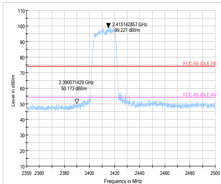
Fig 67. Radiated emission (Power): 802.11n, low channel
