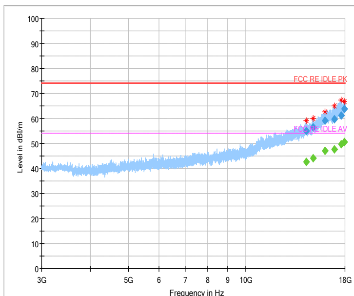
Fig 82. Radiated Spurious Emission (802.11g,Ch6,3GHz~18GHz)
