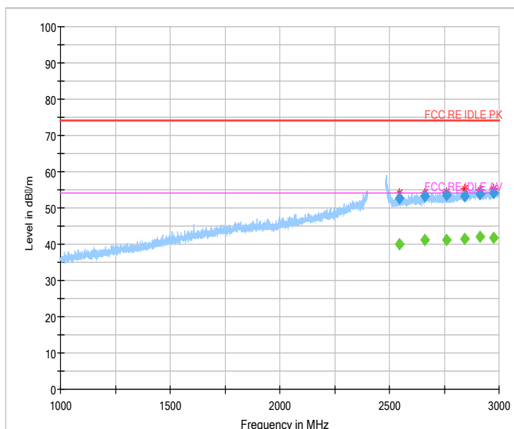
Fig 86. Radiated Spurious Emission (802.11 n-20MHz,Ch1,1GHz~3GHz)
