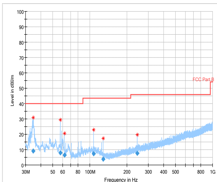
Fig 75. Radiated Spurious Emission (802.11b,Ch6,30MHz~1GHz)
