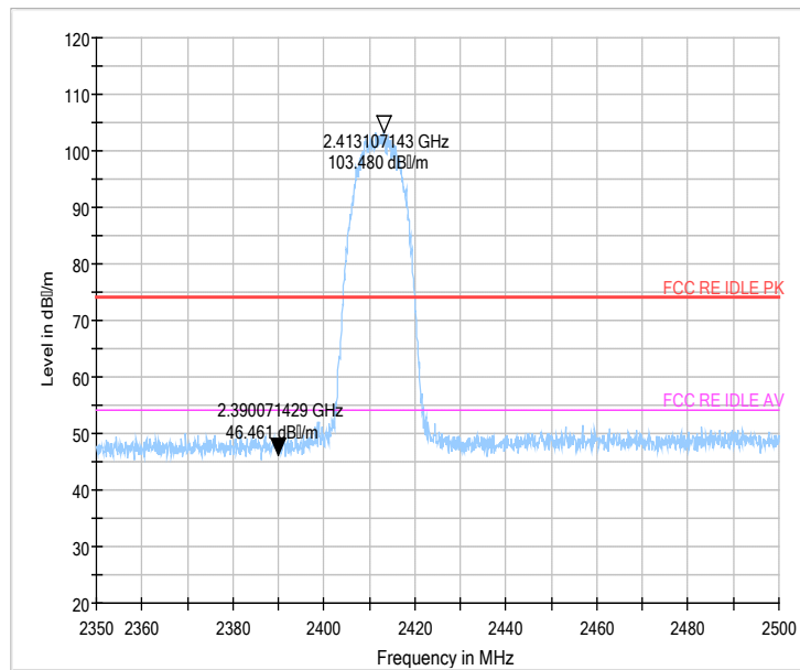
Fig 57. Radiated emission (Power): 802.11b, low channel
