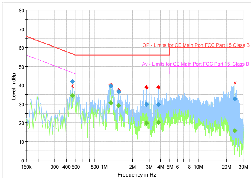
Fig 90. AC Conducted Emission
