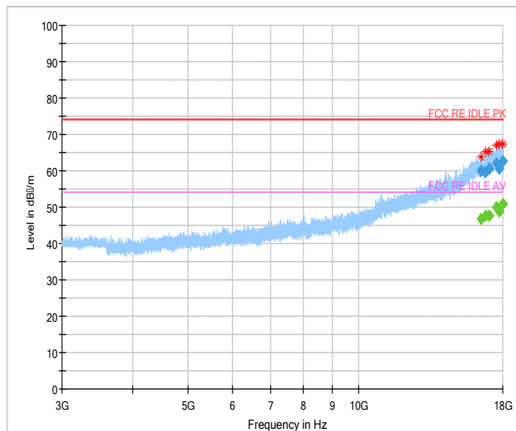
Fig 66. Radiated Spurious Emission (802.11g,Ch6,3GHz~18GHz)
