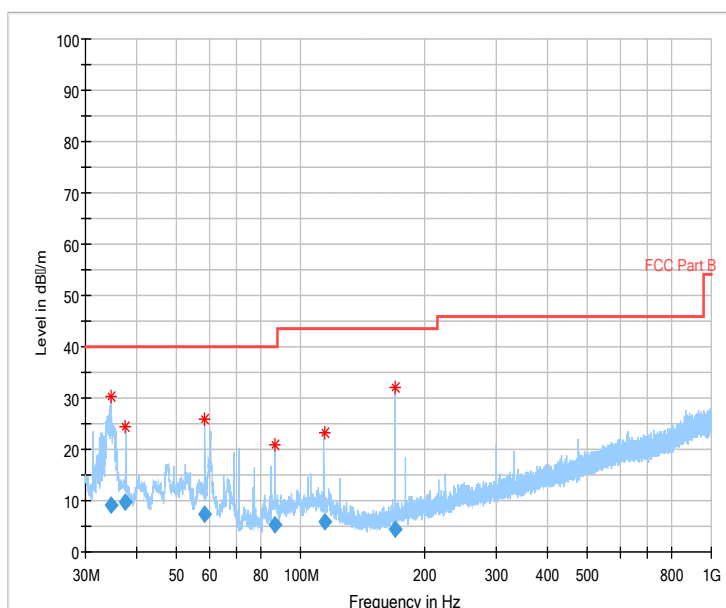
Fig 64. Radiated Spurious Emission (802.11g, Ch6, 30MHz~1GHz)
