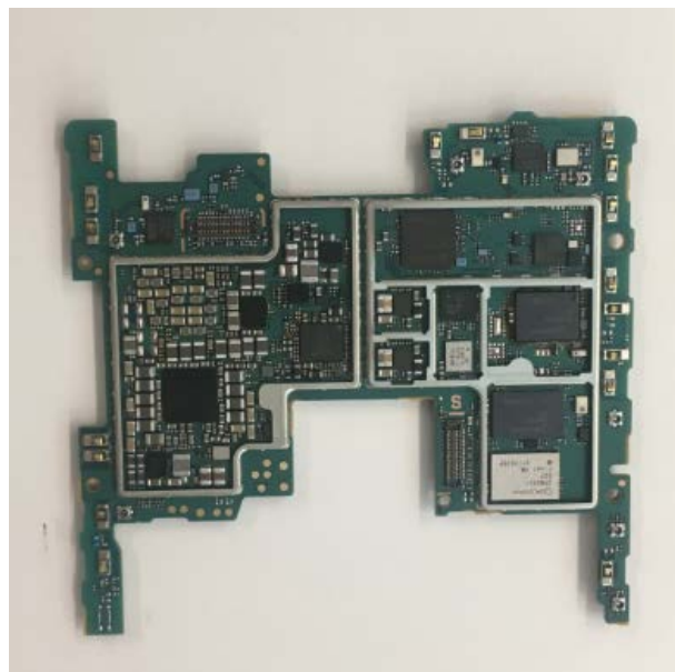
Internal PWB without Shield cases (Rear-side)
