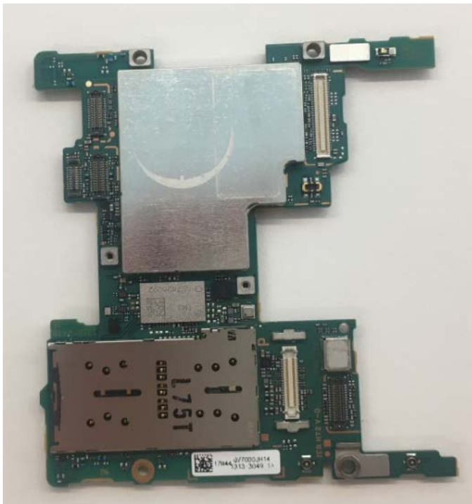
Internal PWB with Shield cases (Front-side)
