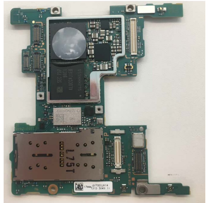
Internal PWB without Shield cases (Front-side)
