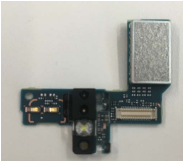
Internal Sub-PWB (Rear-side)
