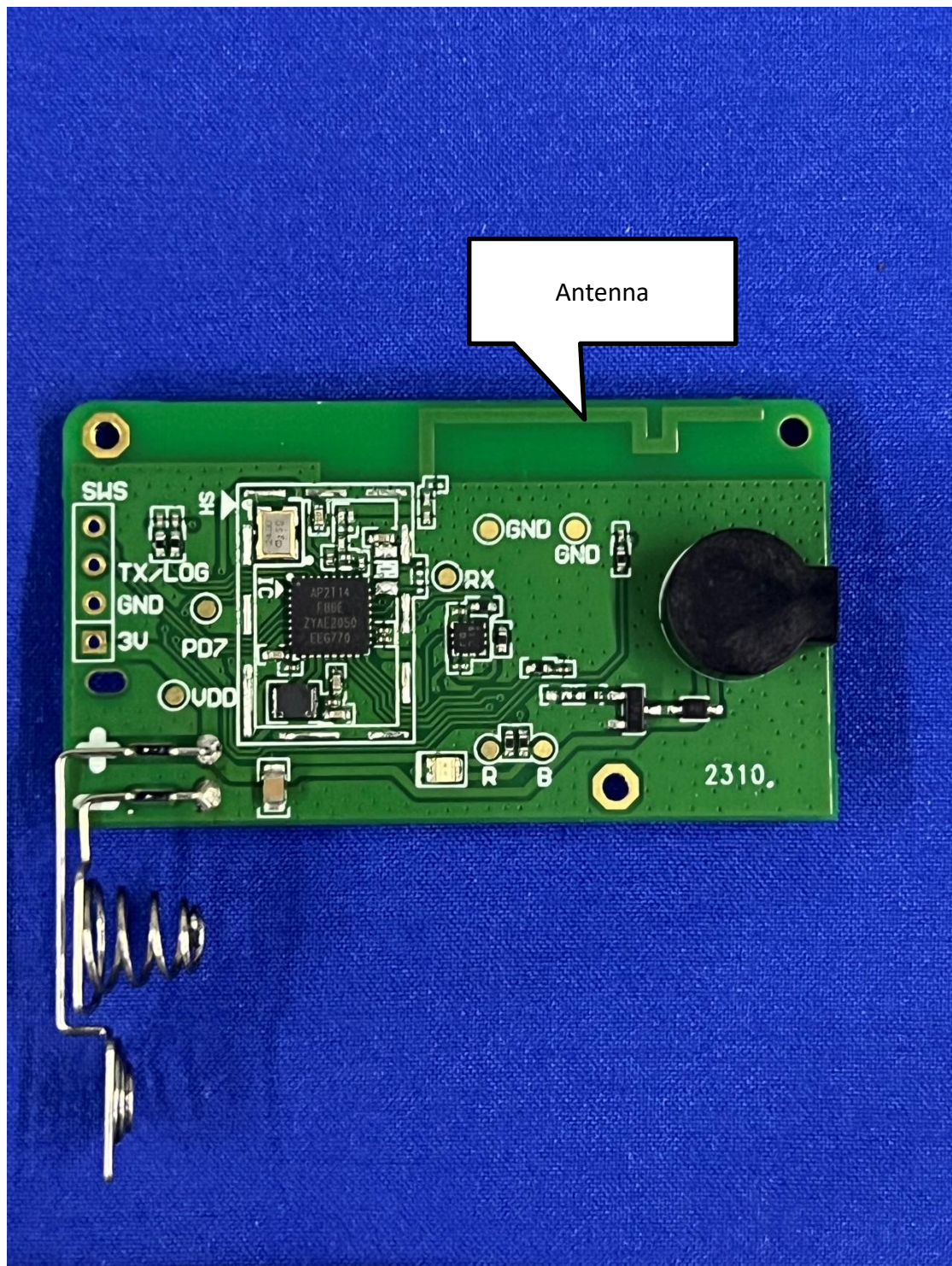
Photo 4: PCB view
