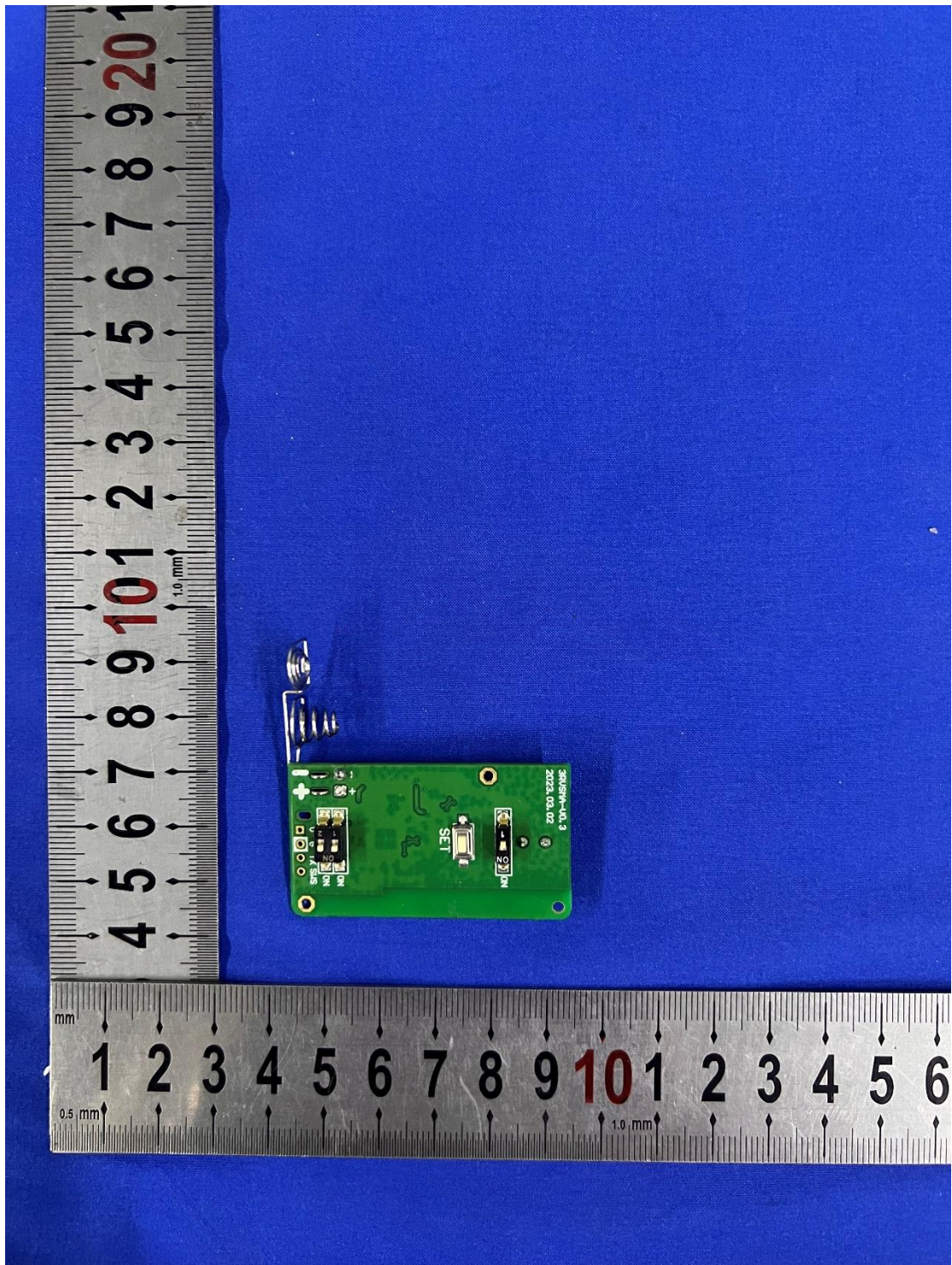
Photo 3: PCB view
