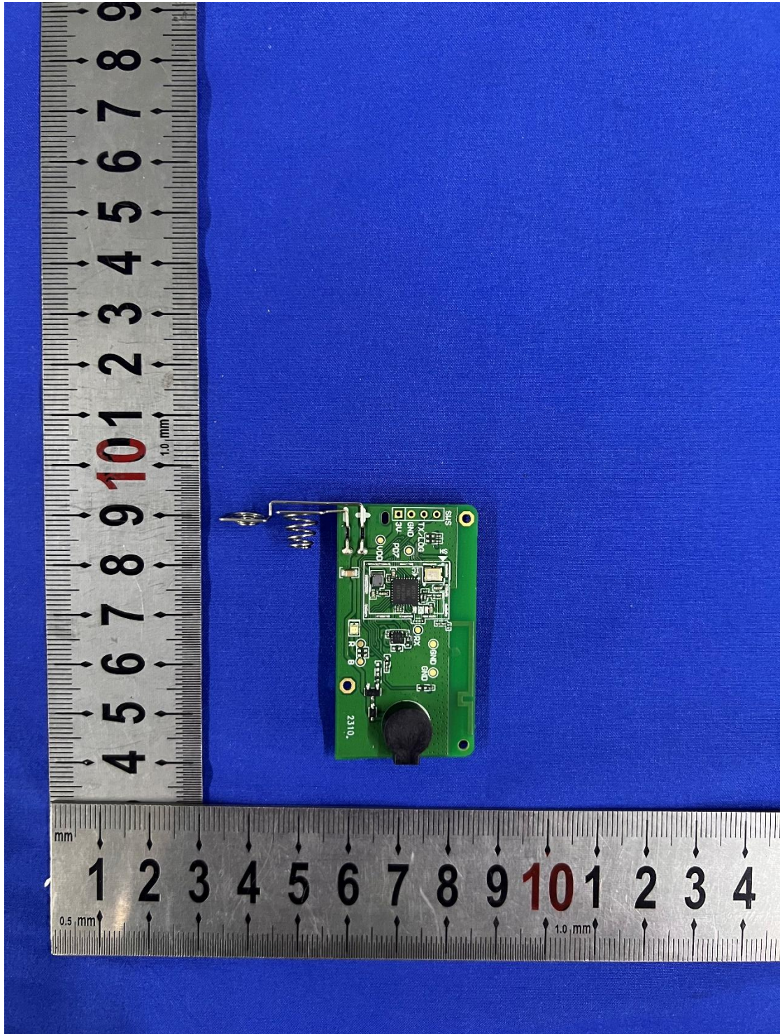
Photo 2: PCB view
