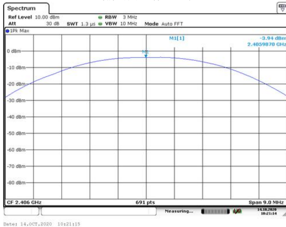
Power NVNT 2406MHz Ant1
