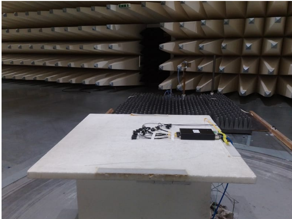
Photo 3: setup radiated emission >1 GHz
