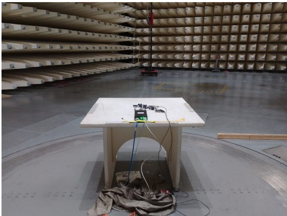
Photo 2: setup radiated emission <1 GHz
