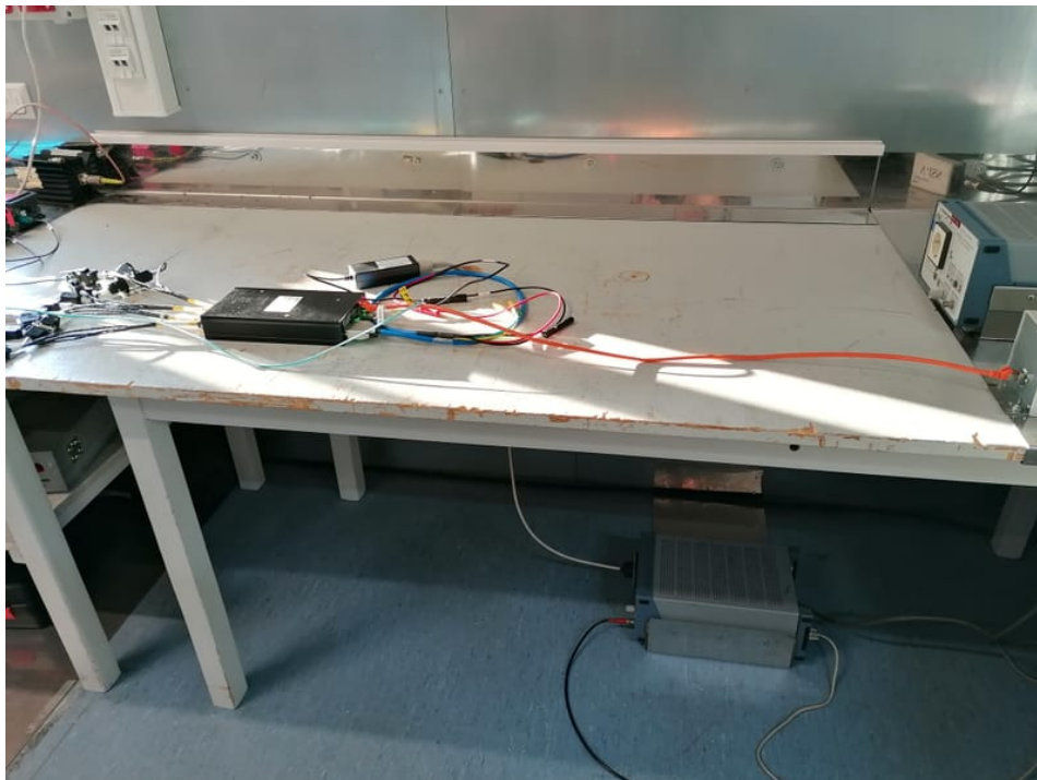
Photo 1: setup conducted emission
