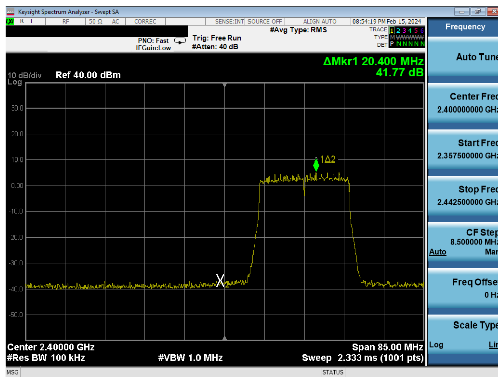
Plot 7-91. Band Edge Antenna 2a (802.11ax OFDMA – RU242 – Ch. 2)
