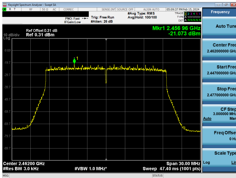
Plot 7-71. Power Spectral Density Plot Antenna 4a (802.11ax OFDMA – RU242 – Ch. 11)
