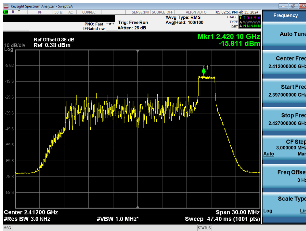
Plot 7-53. Power Spectral Density Plot Antenna 4a (802.11ax OFDMA – RU26 Index 8 – Ch. 1)
