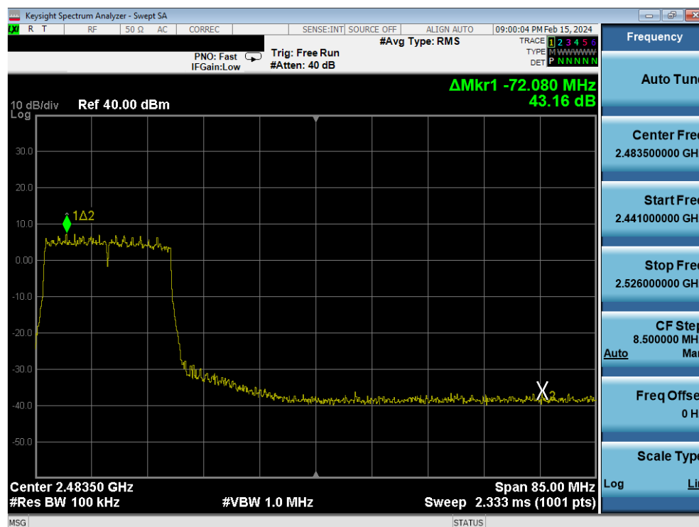
Plot 7-97. Band Edge Antenna 2a (802.11ax OFDMA – RU242 – Ch. 9)
