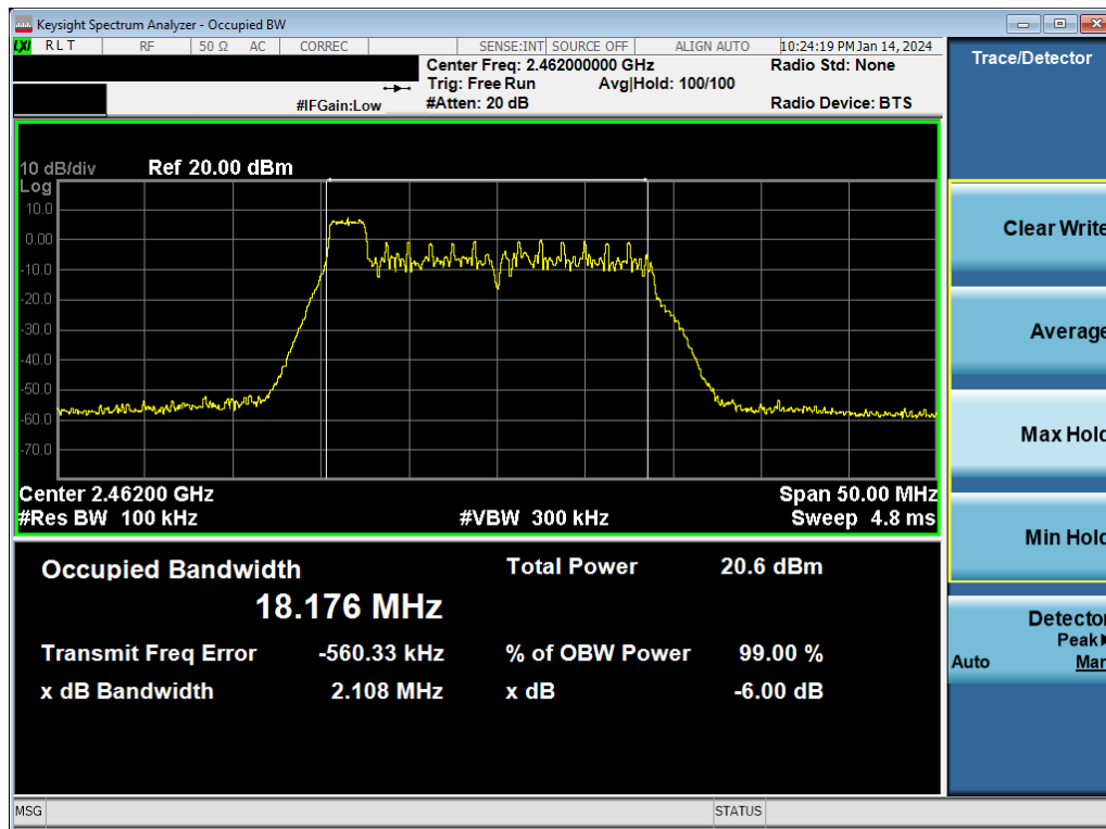
Plot 7-19. 6dB BW & 99% OBW Antenna 2a (802.11ax OFDMA – RU26 Index 0 – Ch. 11)
