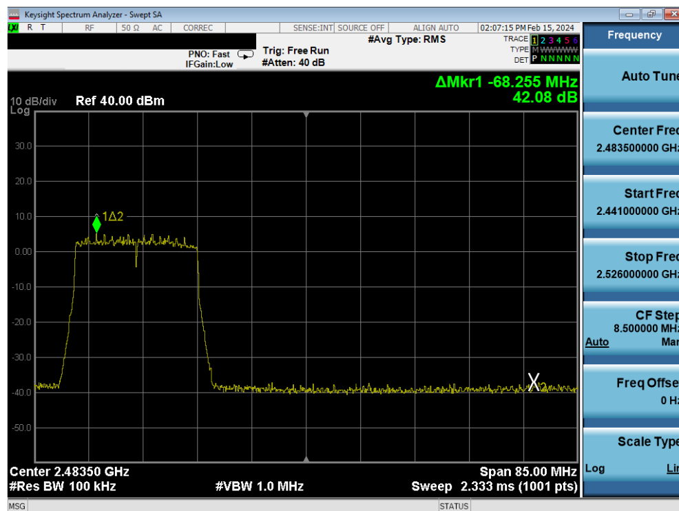
Plot 7-84. Band Edge Antenna 4a (802.11ax OFDMA – RU242 – Ch. 10)
