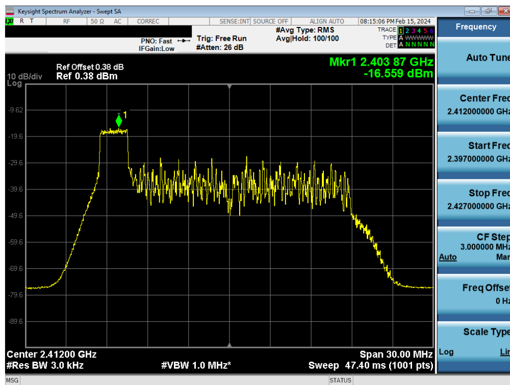
Plot 7-50. Power Spectral Density Plot Antenna 2a (802.11ax OFDMA – RU26 Index 0 – Ch. 1)
