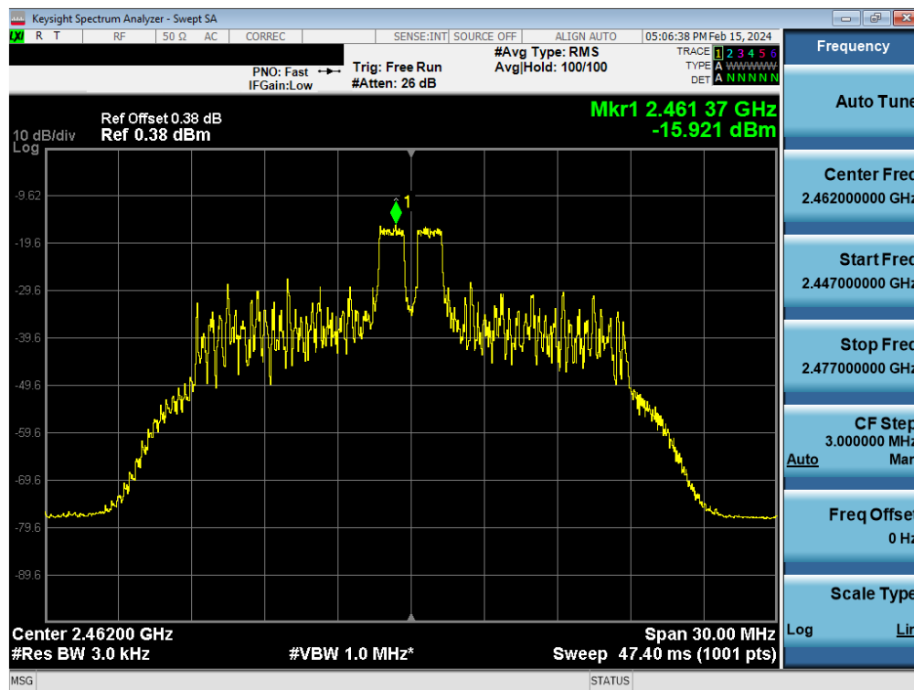
Plot 7-63. Power Spectral Density Plot Antenna 4a (802.11ax OFDMA – RU26 Index 4 – Ch. 11)
