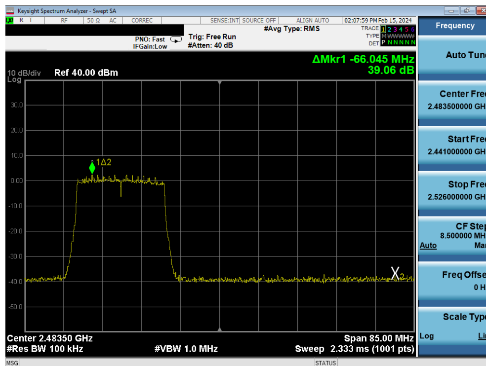
Plot 7-85. Band Edge Antenna 4a (802.11ax OFDMA – RU242 – Ch. 11)
