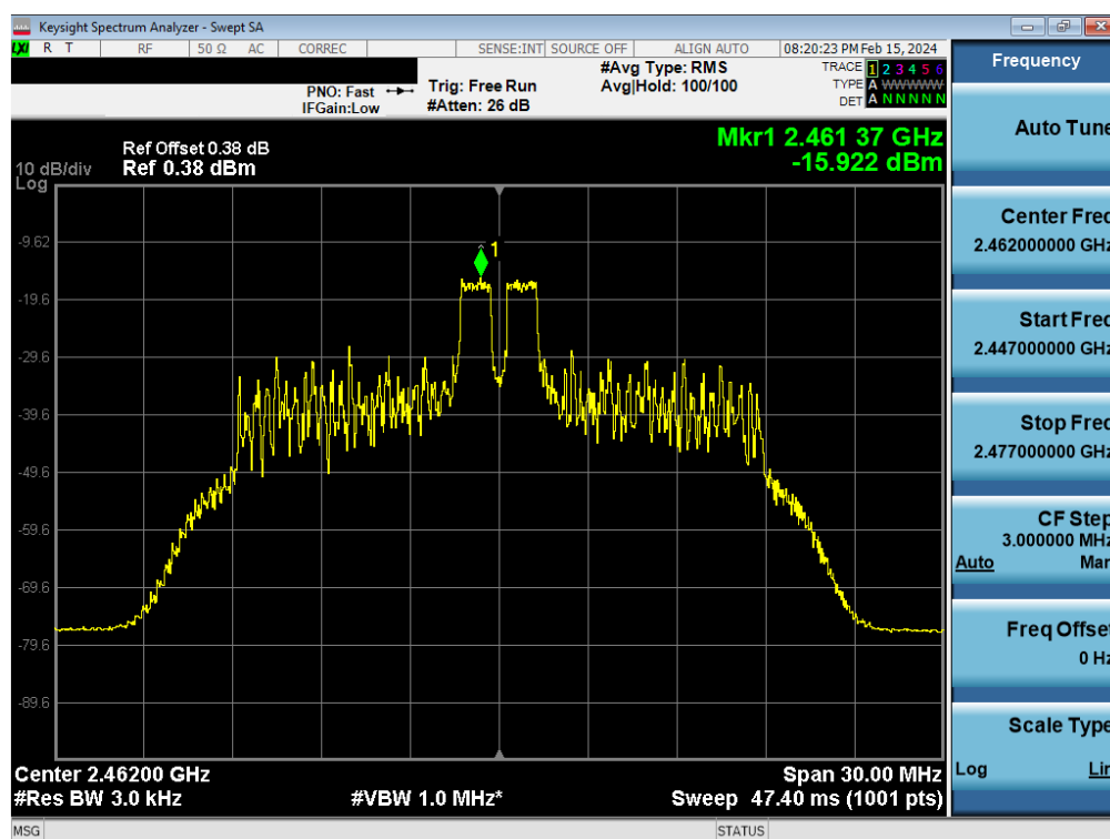
Plot 7-64. Power Spectral Density Plot Antenna 2a (802.11ax OFDMA – RU26 Index 4 – Ch. 11)
