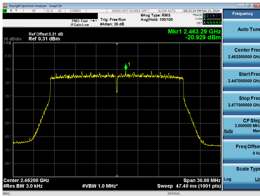
Plot 7-72. Power Spectral Density Plot Antenna 2a (802.11ax OFDMA – RU242 – Ch. 11)
