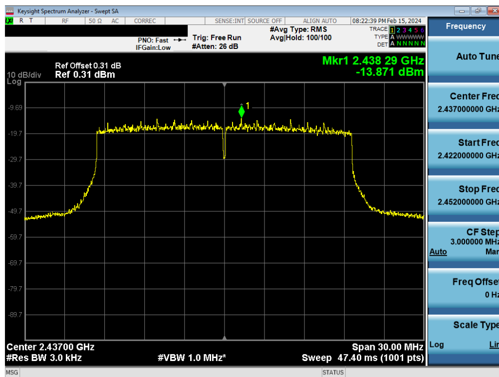
Plot 7-70. Power Spectral Density Plot Antenna 2a (802.11ax OFDMA – RU242 – Ch. 6)
