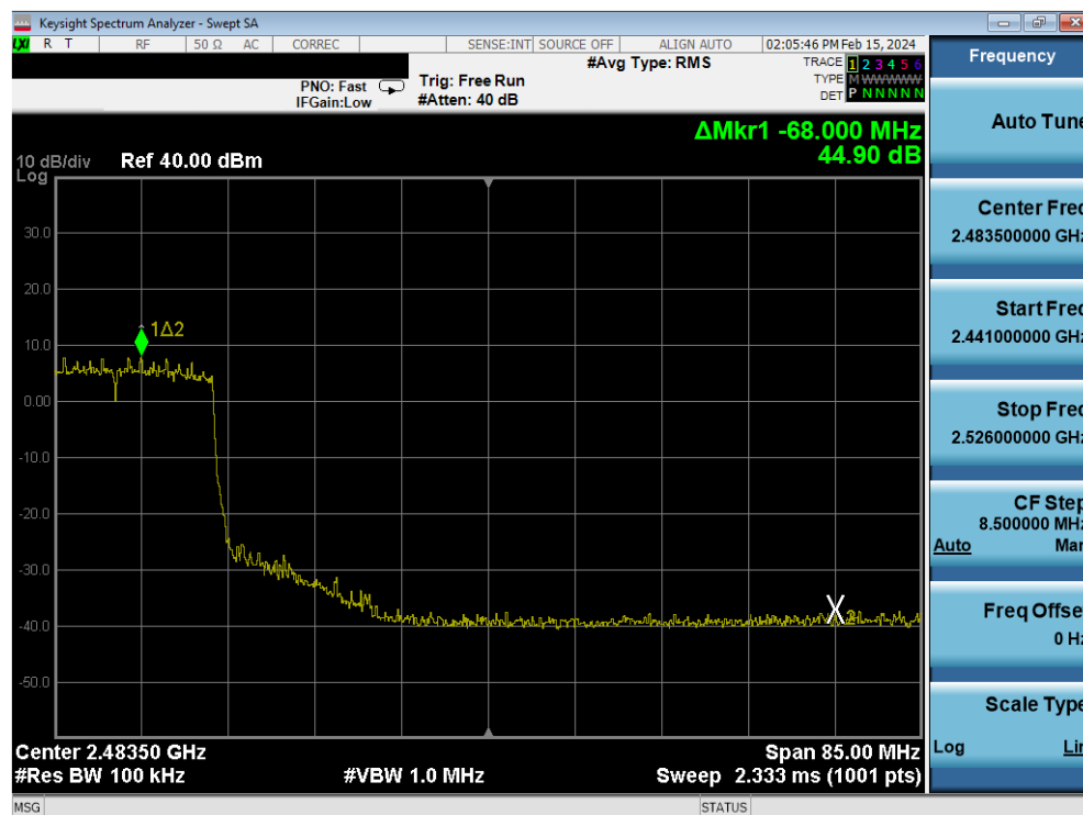
Plot 7-82. Band Edge Antenna 4a (802.11ax OFDMA – RU242 – Ch. 8)
