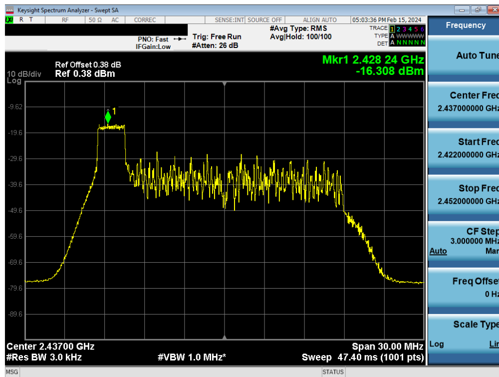
Plot 7-55. Power Spectral Density Plot Antenna 4a (802.11ax OFDMA – RU26 Index 0 – Ch. 6)
