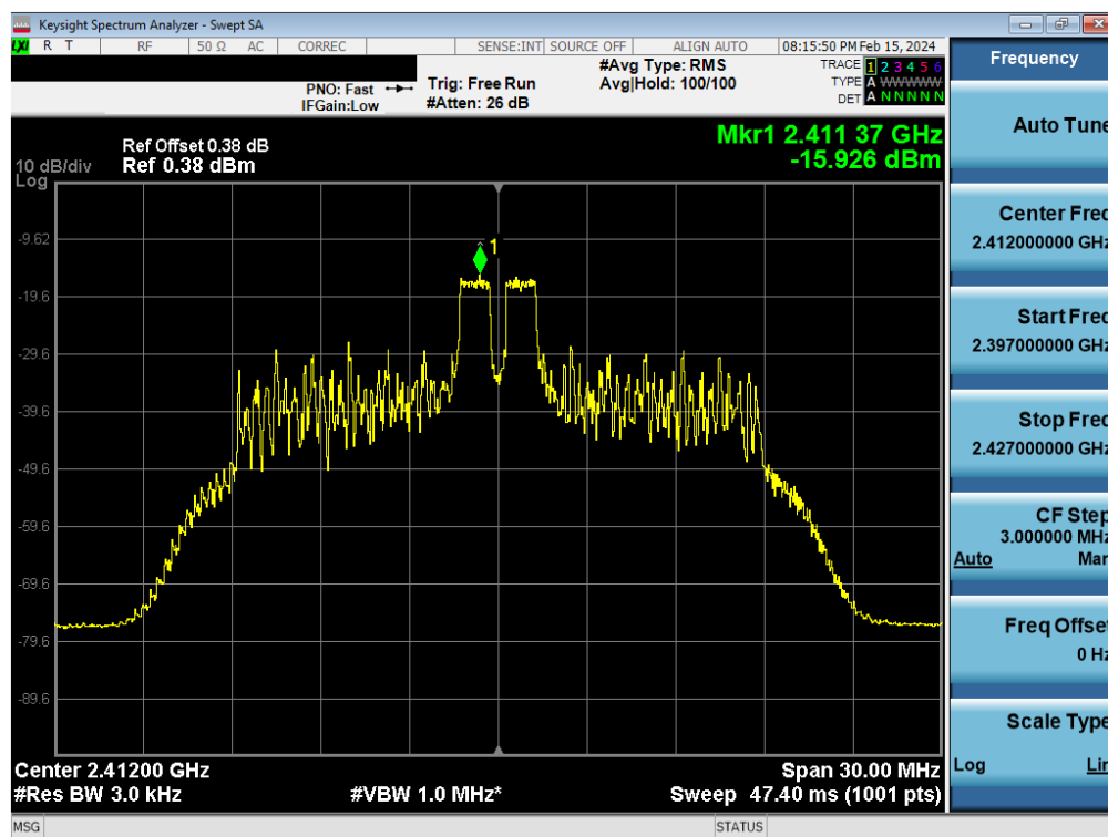
Plot 7-52. Power Spectral Density Plot Antenna 2a (802.11ax OFDMA – RU26 Index 4 – Ch. 1)
