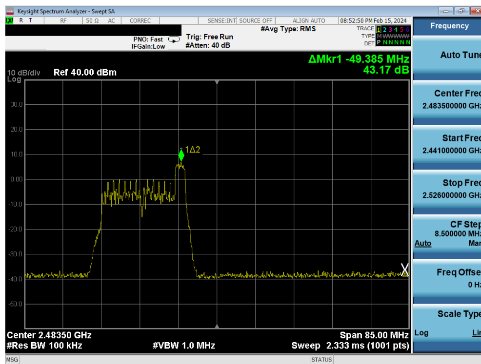
Plot 7-89. Band Edge Antenna 2a (802.11ax OFDMA – RU26 Index 8 – Ch. 12)
