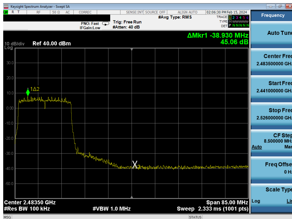
Plot 7-83. Band Edge Antenna 4a (802.11ax OFDMA – RU242 – Ch. 9)
