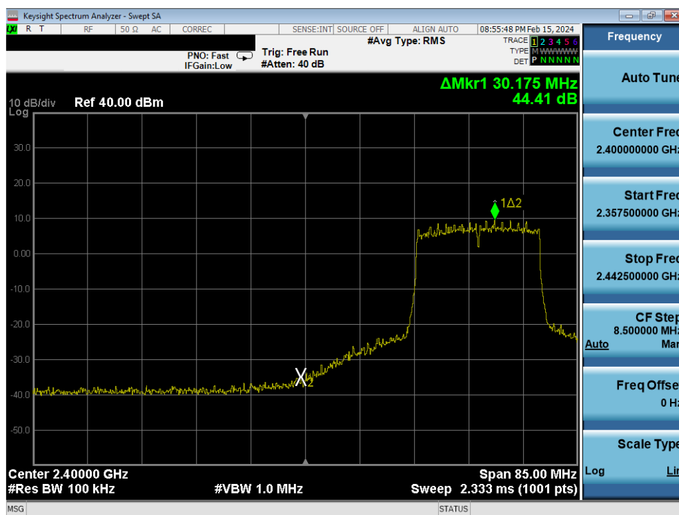
Plot 7-93. Band Edge Antenna 2a (802.11ax OFDMA – RU242 – Ch. 4)
