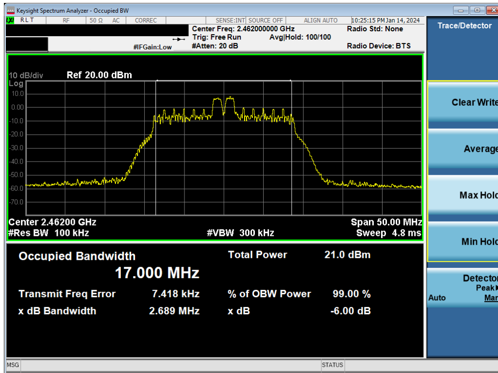
Plot 7-20. 6dB BW & 99% OBW Antenna 2a (802.11ax OFDMA – RU26 Index 4 – Ch. 11)
