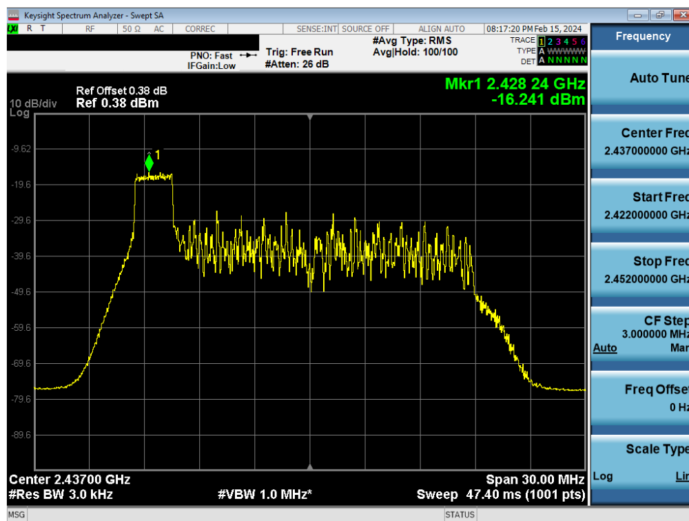
Plot 7-56. Power Spectral Density Plot Antenna 2a (802.11ax OFDMA – RU26 Index 0 – Ch. 6)
