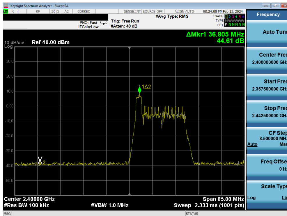
Plot 7-87. Band Edge Antenna 2a (802.11ax OFDMA – RU26 Index 0 – Ch. 1)
