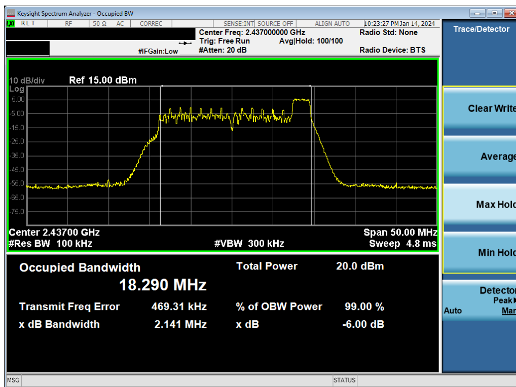
Plot 7-18. 6dB BW & 99% OBW Antenna 2a (802.11ax OFDMA – RU26 Index 8 – Ch. 6)
