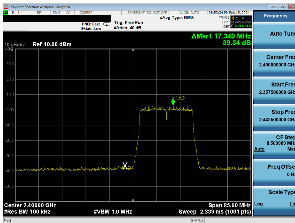
Plot 7-90. Band Edge Antenna 2a (802.11ax OFDMA – RU242 – Ch. 1)
