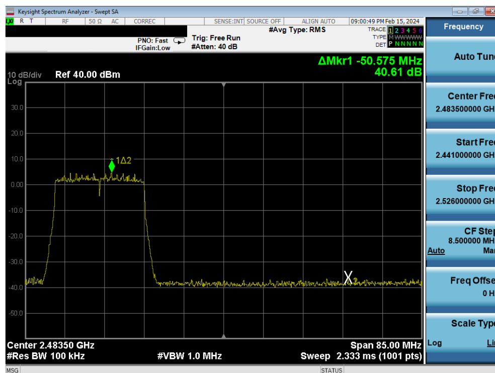
Plot 7-98. Band Edge Antenna 2a (802.11ax OFDMA – RU242 – Ch. 10)
