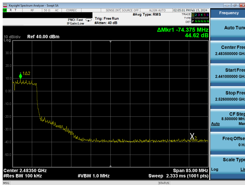
Plot 7-81. Band Edge Antenna 4a (802.11ax OFDMA – RU242 – Ch. 7)
