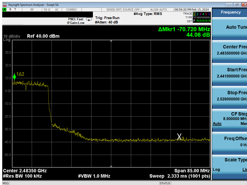
Plot 7-96. Band Edge Antenna 2a (802.11ax OFDMA – RU242 – Ch. 8)
