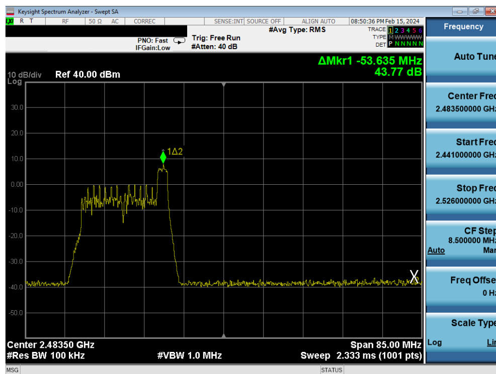
Plot 7-88. Band Edge Antenna 2a (802.11ax OFDMA – RU26 Index 8 – Ch. 11)
