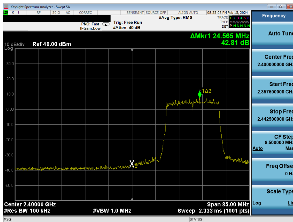
Plot 7-92. Band Edge Antenna 2a (802.11ax OFDMA – RU242 – Ch. 3)
