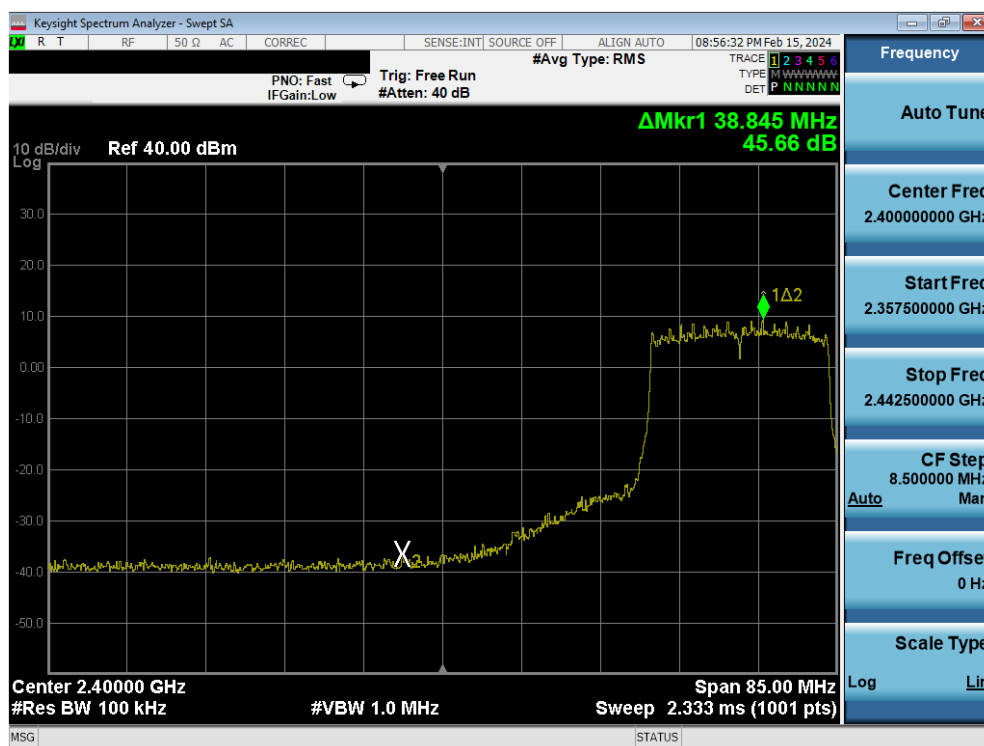
Plot 7-94. Band Edge Antenna 2a (802.11ax OFDMA – RU242 – Ch. 5)
