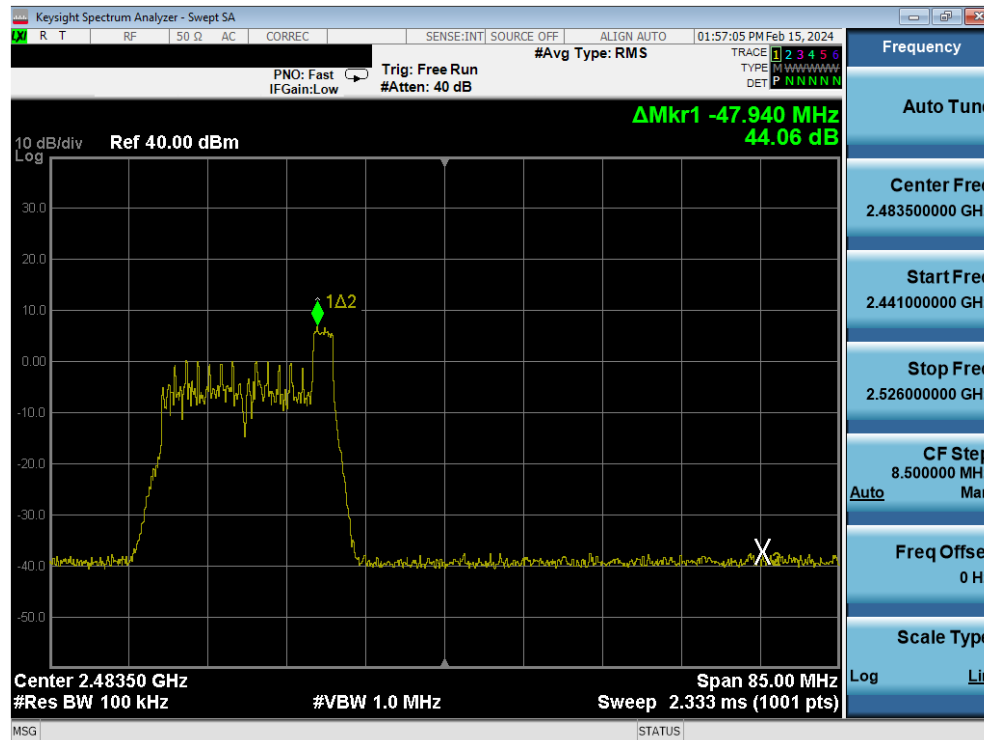
Plot 7-74. Band Edge Antenna 4a (802.11ax OFDMA – RU26 Index 8 – Ch. 11)
