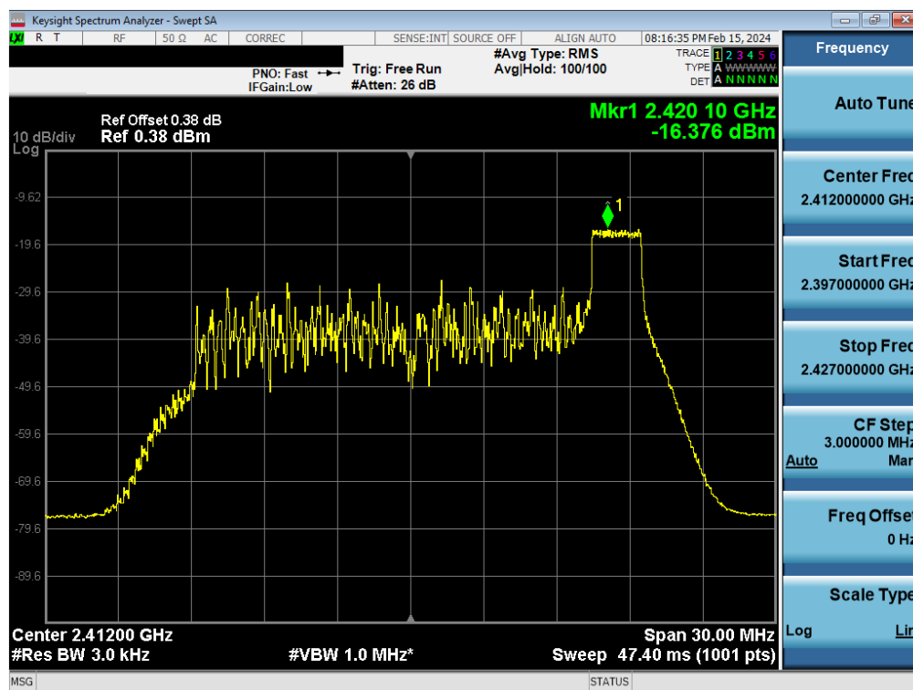
Plot 7-54. Power Spectral Density Plot Antenna 2a (802.11ax OFDMA – RU26 Index 8 – Ch. 1)
