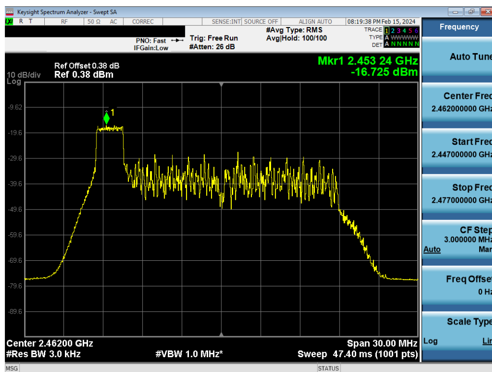
Plot 7-62. Power Spectral Density Plot Antenna 2a (802.11ax OFDMA – RU26 Index 0 – Ch. 11)
