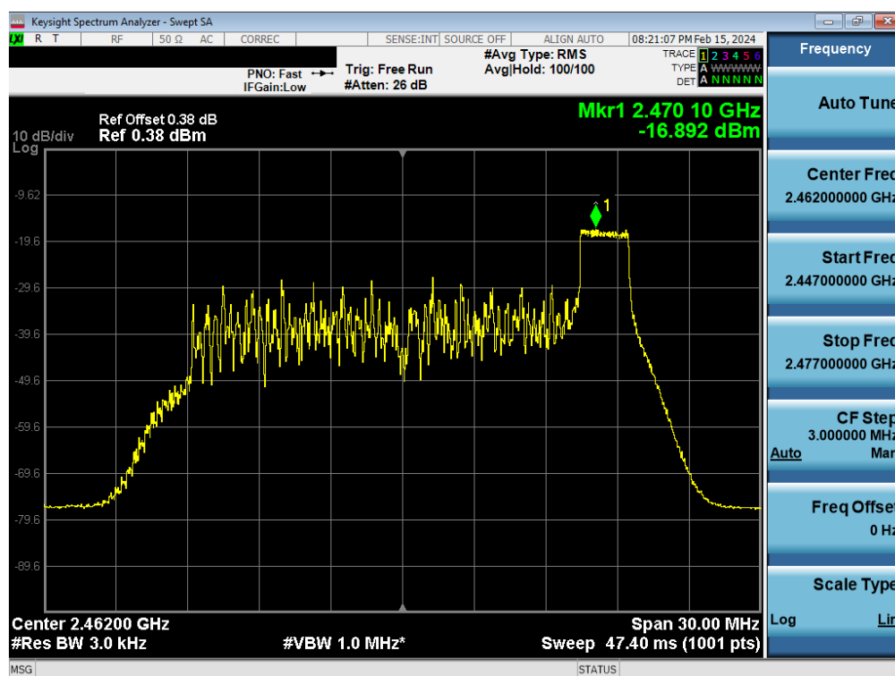
Plot 7-66. Power Spectral Density Plot Antenna 2a (802.11ax OFDMA – RU26 Index 8 – Ch. 11)
