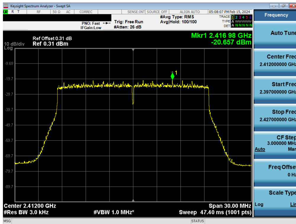
Plot 7-67. Power Spectral Density Plot Antenna 4a (802.11ax OFDMA – RU242 – Ch. 1)
