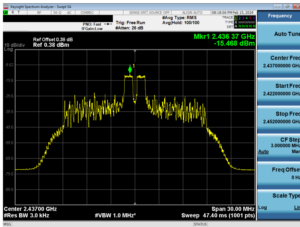
Plot 7-58. Power Spectral Density Plot Antenna 2a (802.11ax OFDMA – RU26 Index 4 – Ch. 6)
