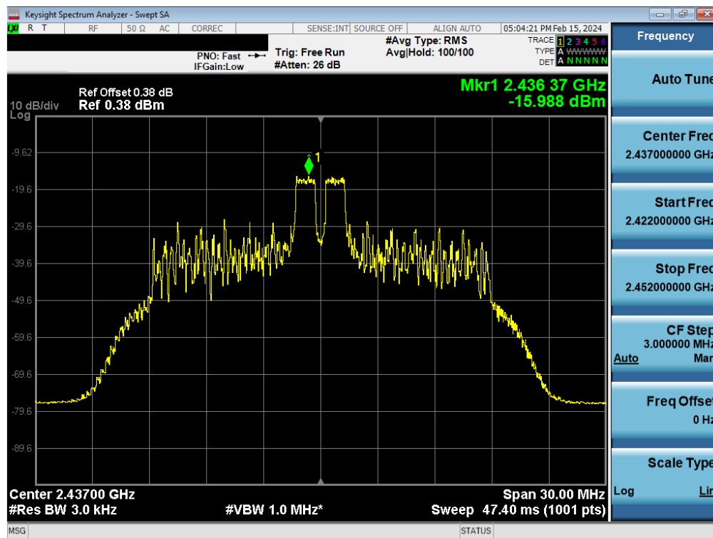
Plot 7-57. Power Spectral Density Plot Antenna 4a (802.11ax OFDMA – RU26 Index 4 – Ch. 6)
