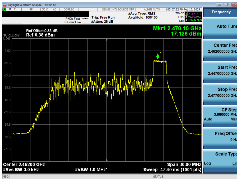
Plot 7-65. Power Spectral Density Plot Antenna 4a (802.11ax OFDMA – RU26 Index 8 – Ch. 11)
