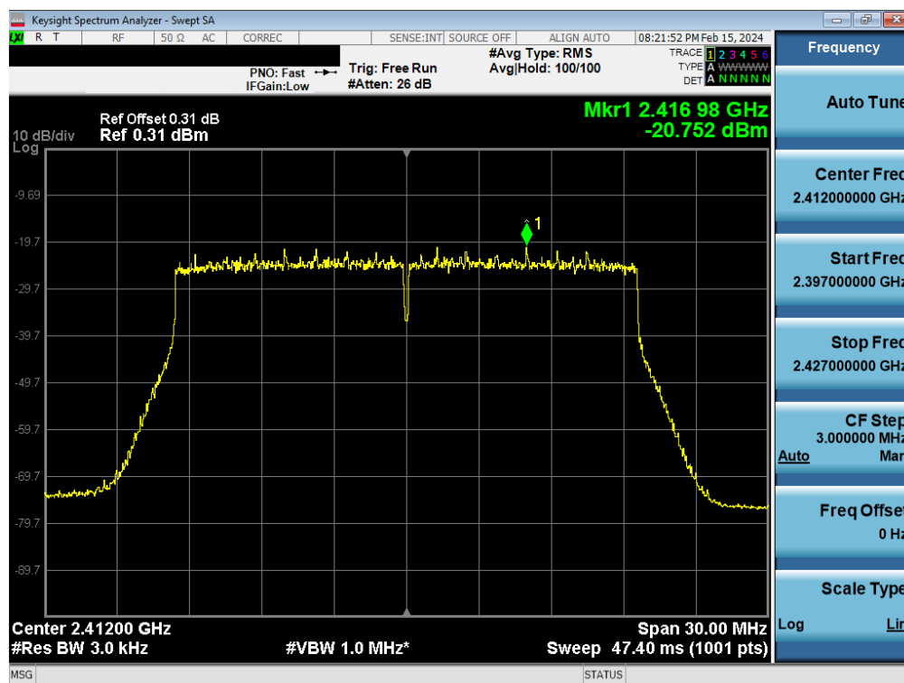
Plot 7-68. Power Spectral Density Plot Antenna 2a (802.11ax OFDMA – RU242 – Ch. 1)
