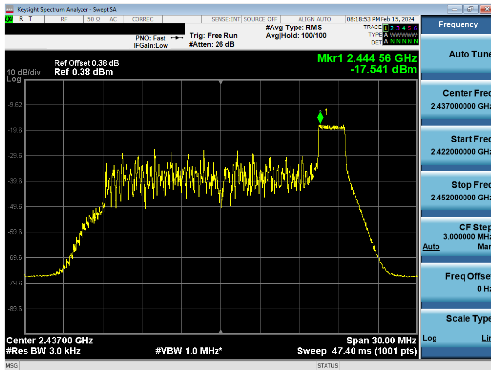
Plot 7-60. Power Spectral Density Plot Antenna 2a (802.11ax OFDMA – RU26 Index 8 – Ch. 6)
