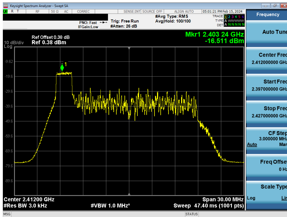
Plot 7-49. Power Spectral Density Plot Antenna 4a (802.11ax OFDMA – RU26 Index 0 – Ch. 1)
