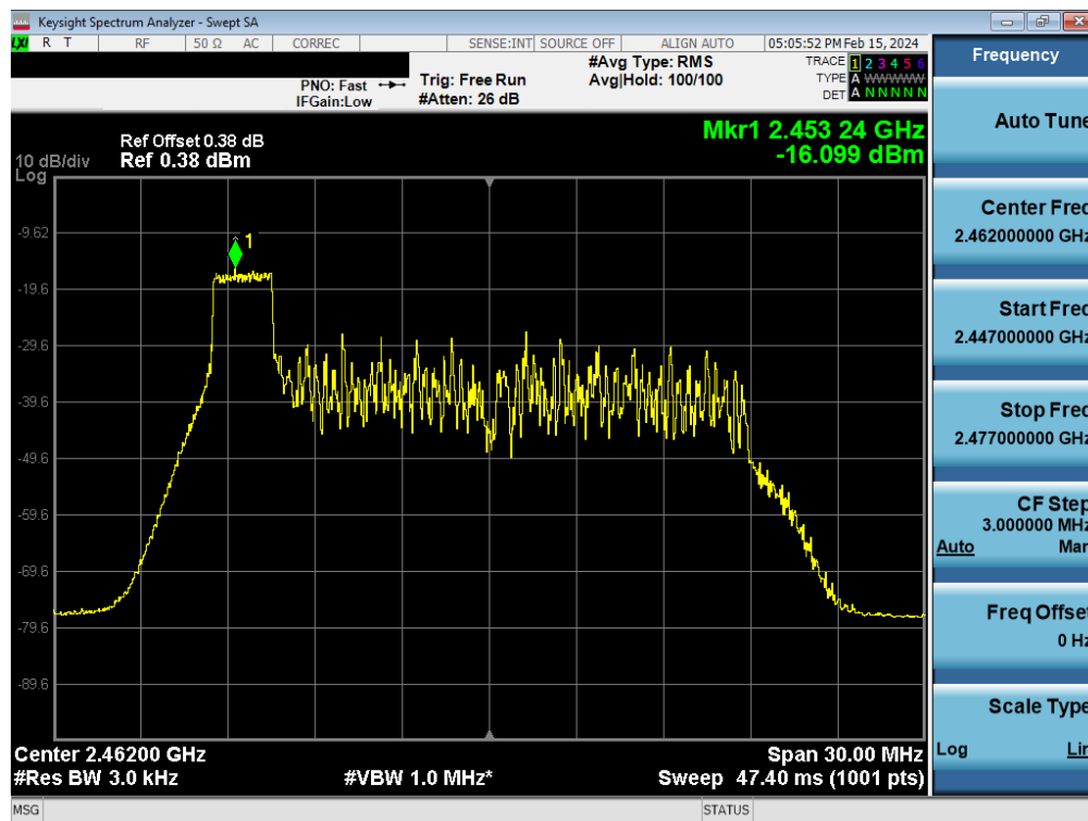
Plot 7-61. Power Spectral Density Plot Antenna 4a (802.11ax OFDMA – RU26 Index 0 – Ch. 11)
