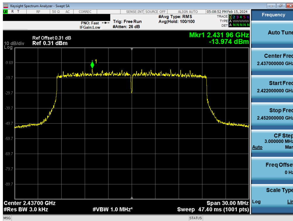
Plot 7-69. Power Spectral Density Plot Antenna 4a (802.11ax OFDMA – RU242 – Ch. 6)
