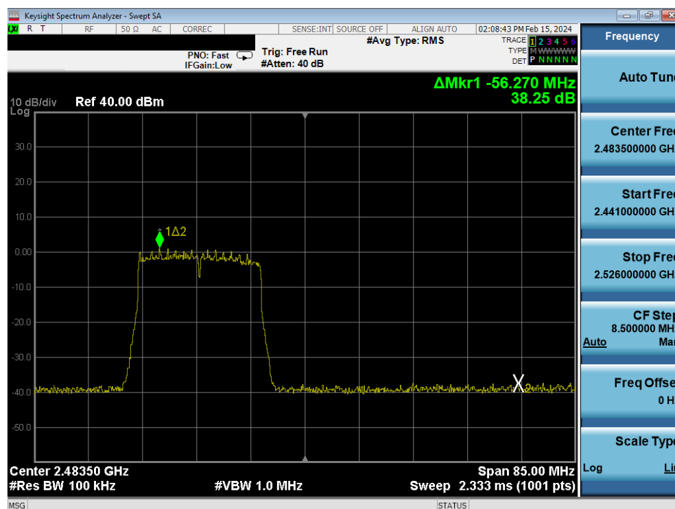
Plot 7-86. Band Edge Antenna 4a (802.11ax OFDMA – RU242 – Ch. 12)
