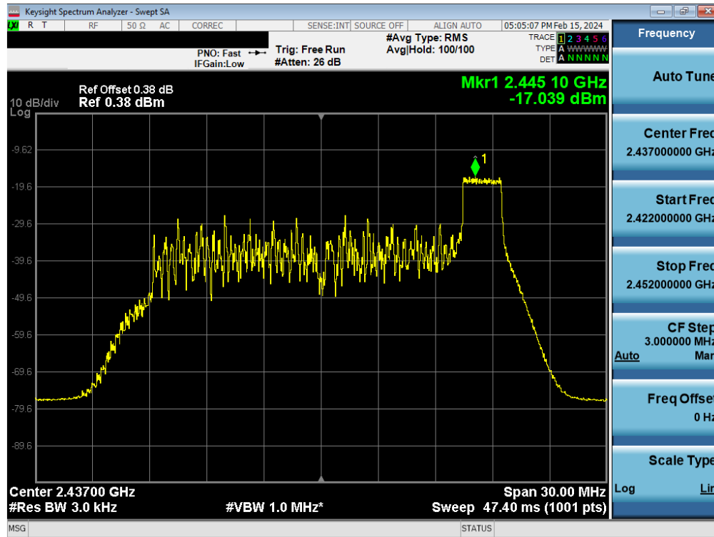
Plot 7-59. Power Spectral Density Plot Antenna 4a (802.11ax OFDMA – RU26 Index 8 – Ch. 6)
