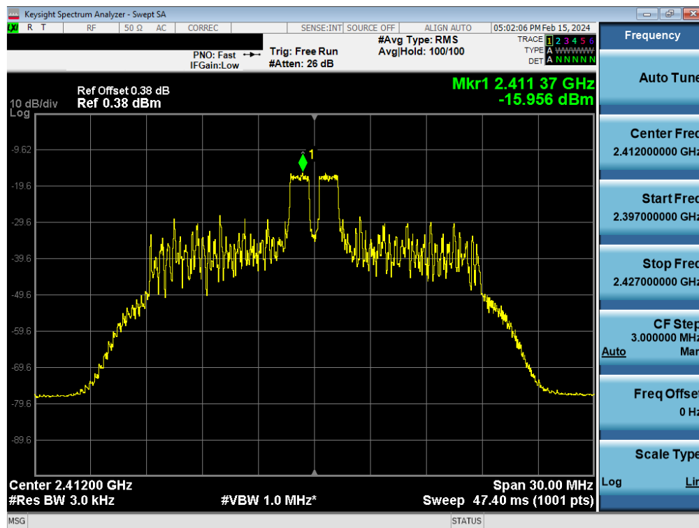
Plot 7-51. Power Spectral Density Plot Antenna 4a (802.11ax OFDMA – RU26 Index 4 – Ch. 1)
