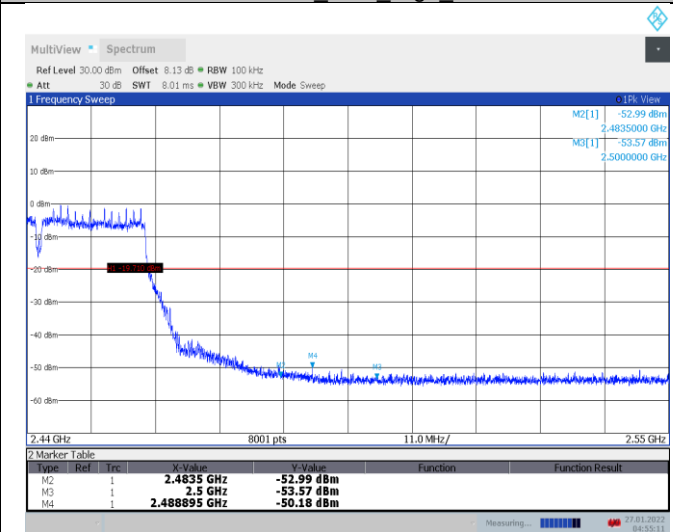
11N40SISO_Ant1_High_2447
