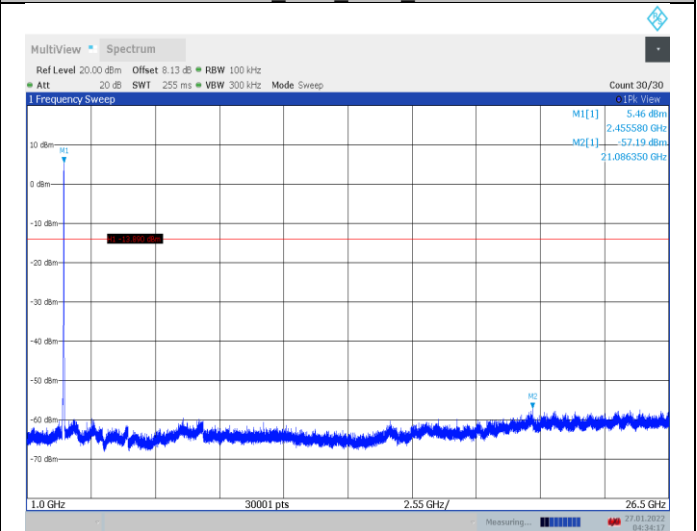
11N20SISO_Ant1_2457_1000~26500
