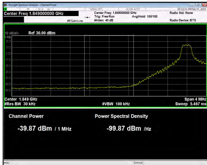
Band2 16QAM BW=10MHz Channel=18650 RB Size=1 Position=#0 Normal
