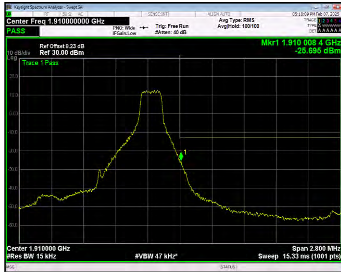
Band2 QPSK BW=1.4MHz Channel=19193 RB Size=6 Position=#0 Extended
