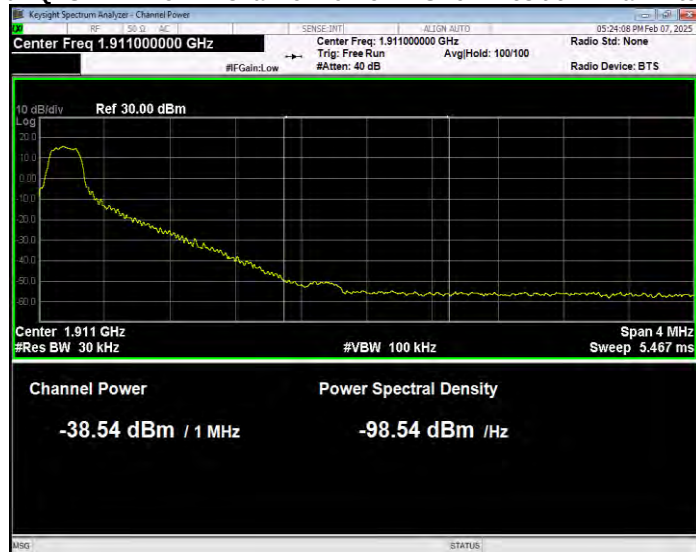
Band2 QPSK BW=15MHz Channel=19125 RB Size=1 Position=#Max Normal
