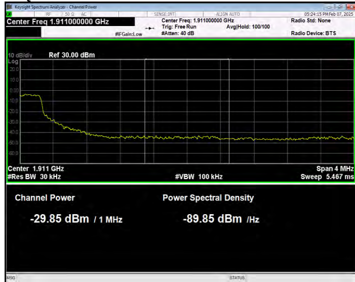
Band2 QPSK BW=15MHz Channel=19125 RB Size=75 Position=#0 Normal
