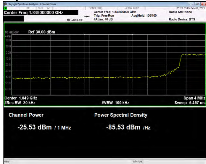
Band2 QPSK BW=10MHz Channel=18650 RB Size=50 Position=#0 Normal
