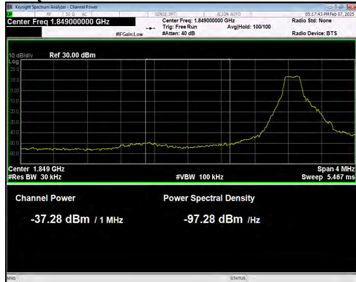
Band2 16QAM BW=1.4MHz Channel=18607 RB Size=1 Position=#0 Normal
