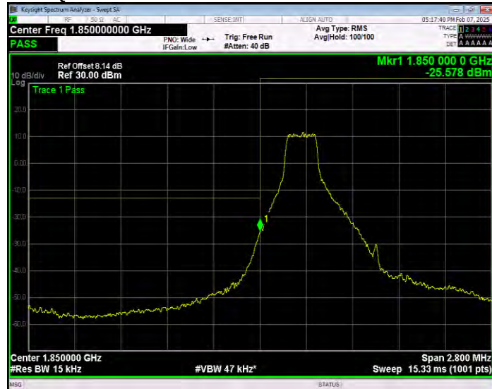
Band2 16QAM BW=1.4MHz Channel=18607 RB Size=1 Position=#Max Extended
