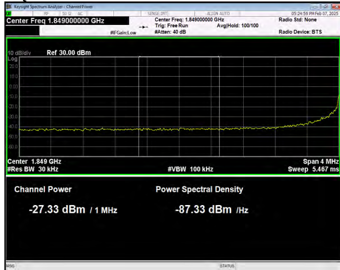
Band2 QPSK BW=20MHz Channel=18700 RB Size=100 Position=#0 Normal
