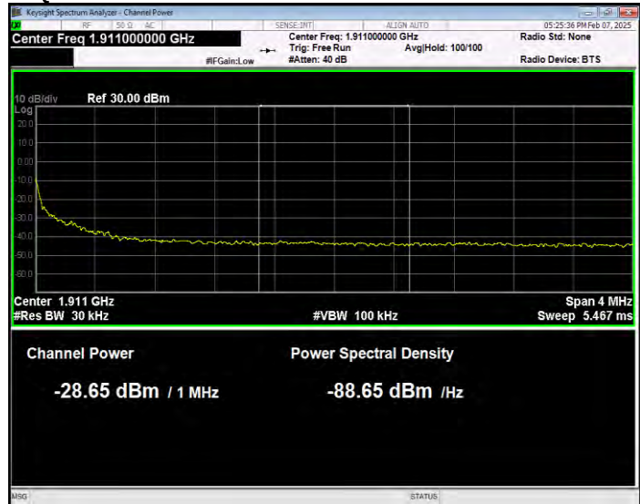
Band2 QPSK BW=20MHz Channel=19100 RB Size=100 Position=#0 Normal
