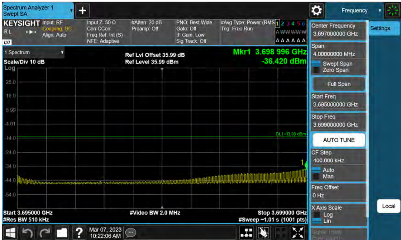
Sub6 n77(78). Low Band Edge Plot (30 M BW Ch.647668 BPSK 1RB)(2)
