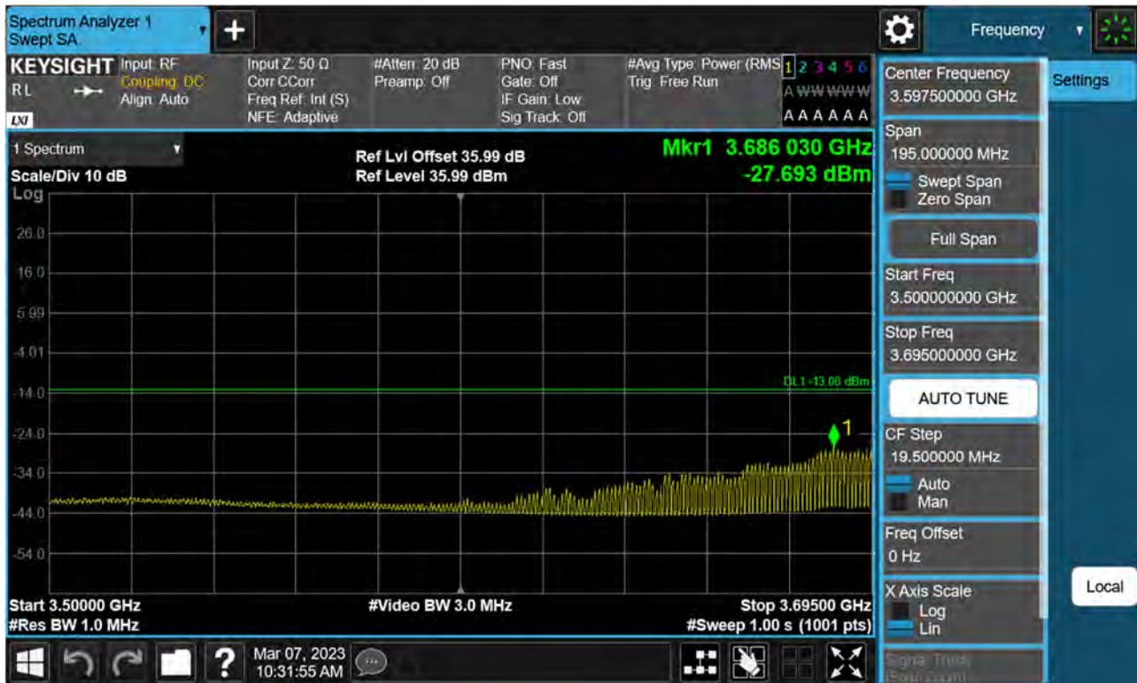
Sub6 n77(78). Low Band Edge Plot (40 M BW Ch.648000 BPSK FullRB)(3)
