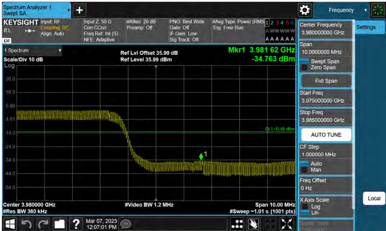
Sub6 n77(78). High Band Edge Plot (80 M BW Ch.662666 BPSK FullRB)(1)
