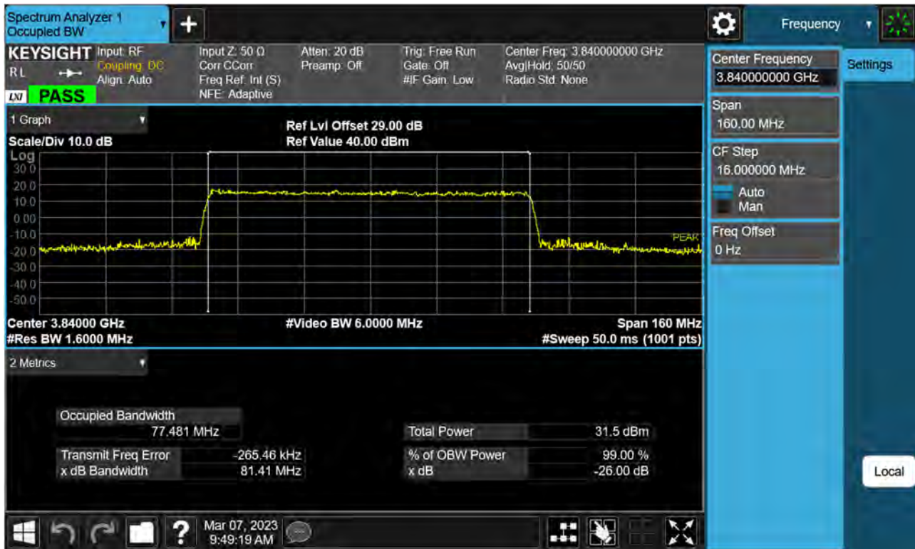
Sub6 n77(78). Occupied Bandwidth Plot (80 M BW Ch.656000 16QAM)
