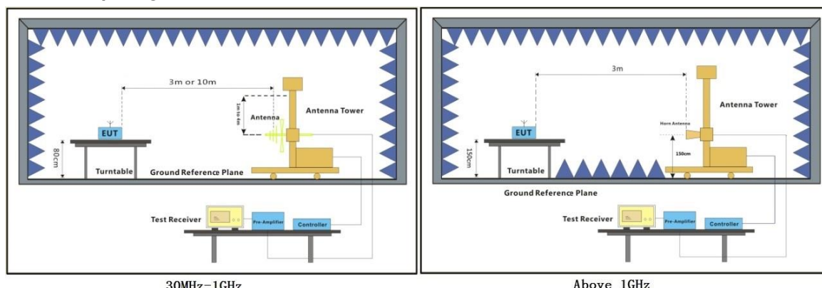
30MHz-1GHz
