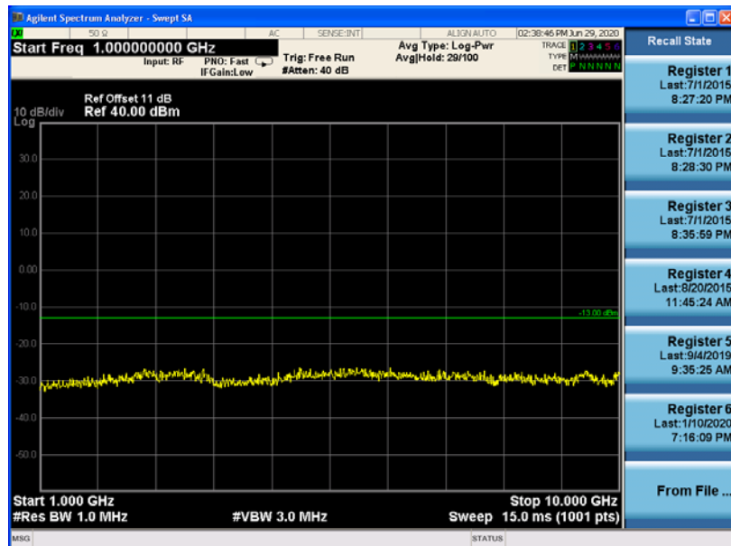
Channel 189, 1GHz~10GHz
