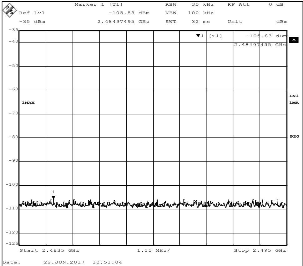
Figure 12 - Band-edge Measurement, High Channel, Restricted Frequency The plot shows an uncorrected measurement, used for relative measurements only.
