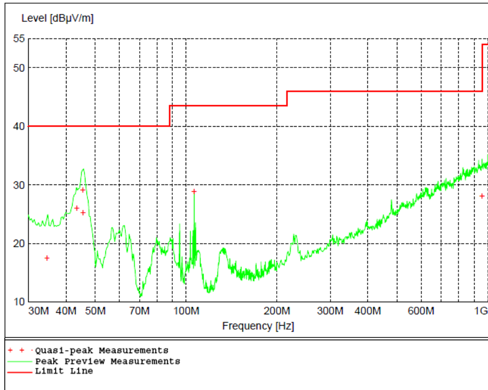
Figure 5 - Radiated Emissions Plot, High Channel X - Axis of EUT was found to be the worse-case
