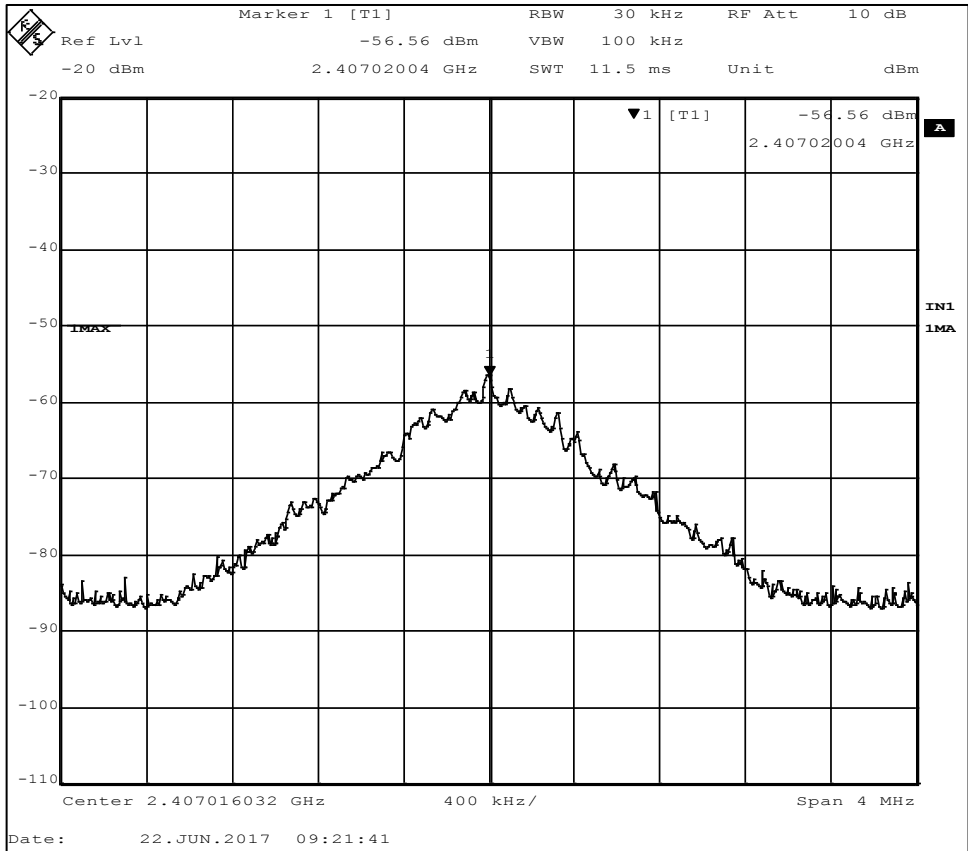
Figure 11 - Band-edge Measurement, Low Channel, Fundamental The plot shows an uncorrected measurement, used for relative measurements only.
