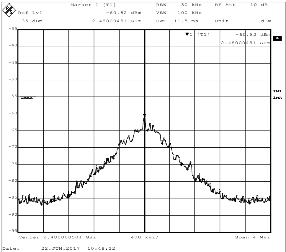
Figure 13 - Band-edge Measurement, High Channel, Fundamental The plot shows an uncorrected measurement, used for relative measurements only.
