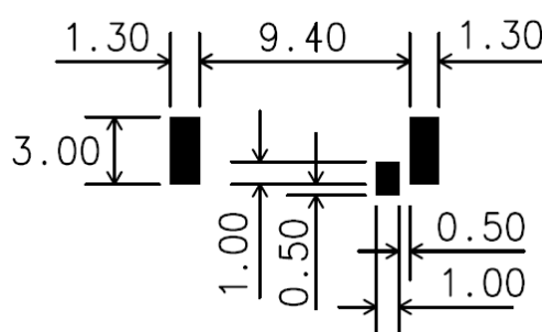
[Recommended PCB pattern]
