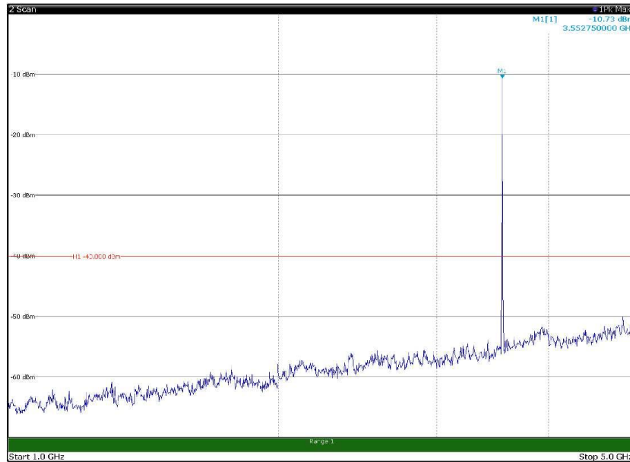
Channel: BOTTOM, Modulation: QPSK, BW=5MHz, Range: 1GHz - 5GHz, Polarization: Horizontal
