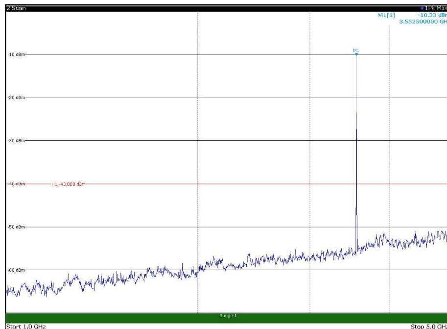
Channel: BOTTOM, Modulation: QPSK, BW=5MHz, Range: 1GHz - 5GHz, Polarization: Vertical
