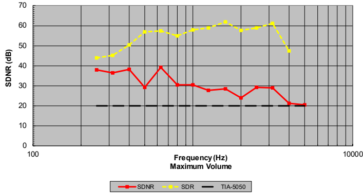
TIA-5050 Measurement at 8N Receive Signal-To-Distortion & Noise Ratio vs Frequency
