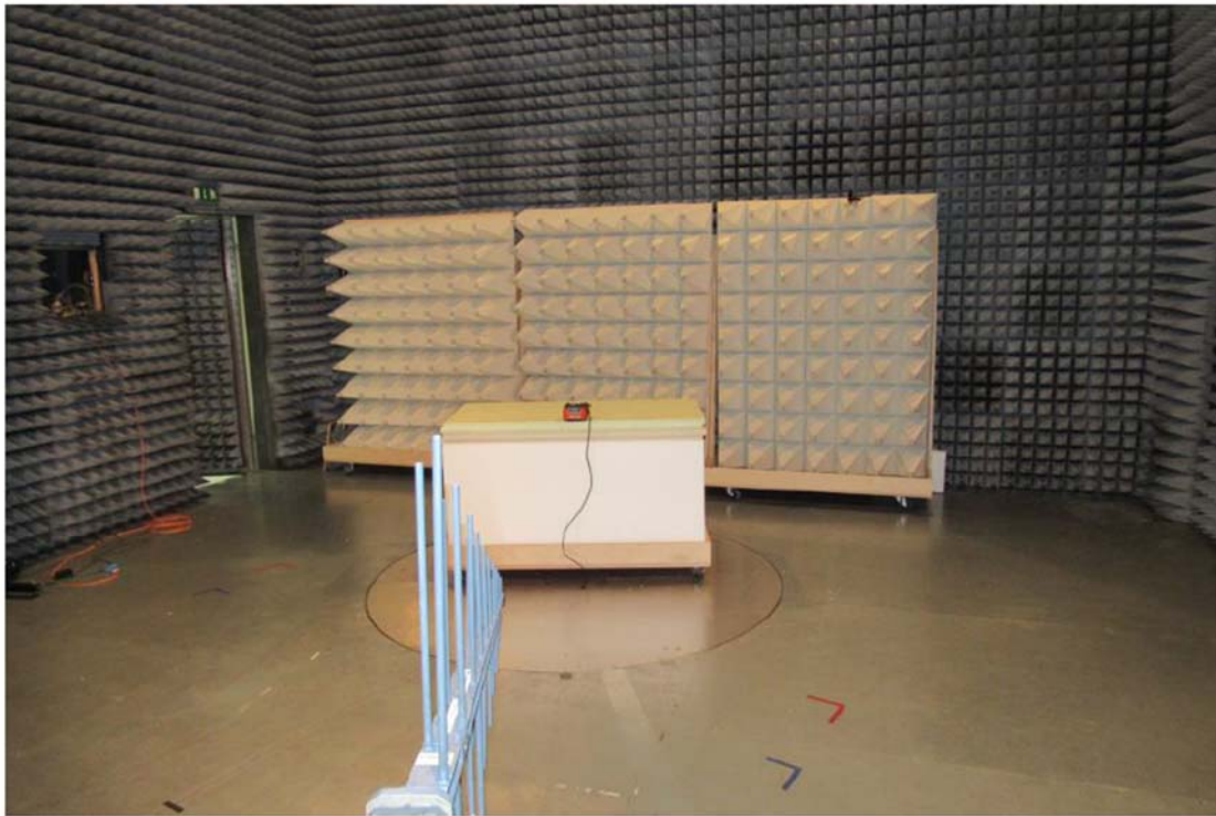
Test setup between 200MHz - 1GHz
