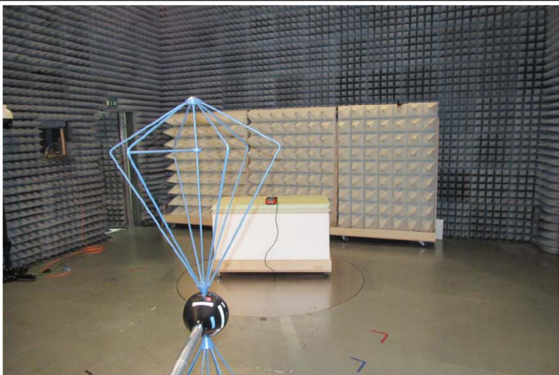
Test setup below 200MHz
