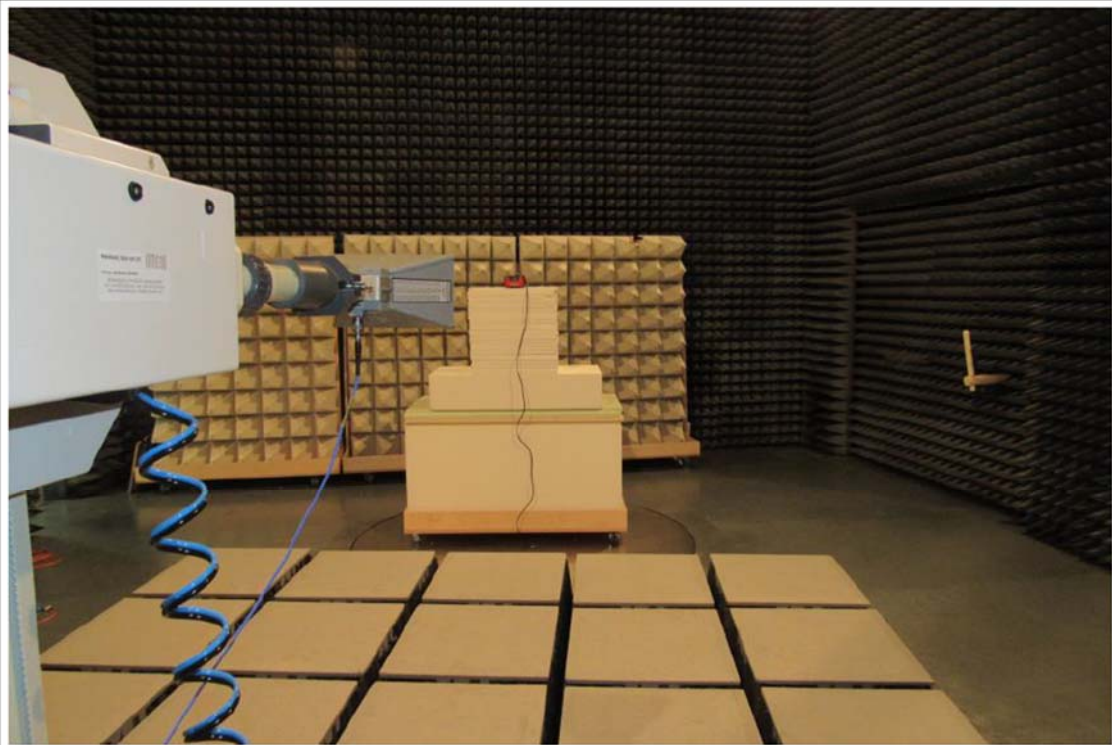
Test setup between 1GHz - 17GHz
