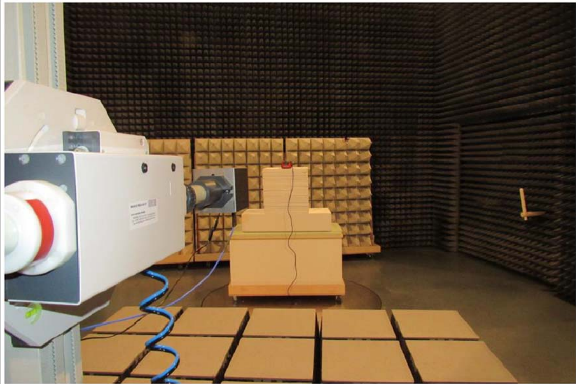
Test setup above 17GHz
