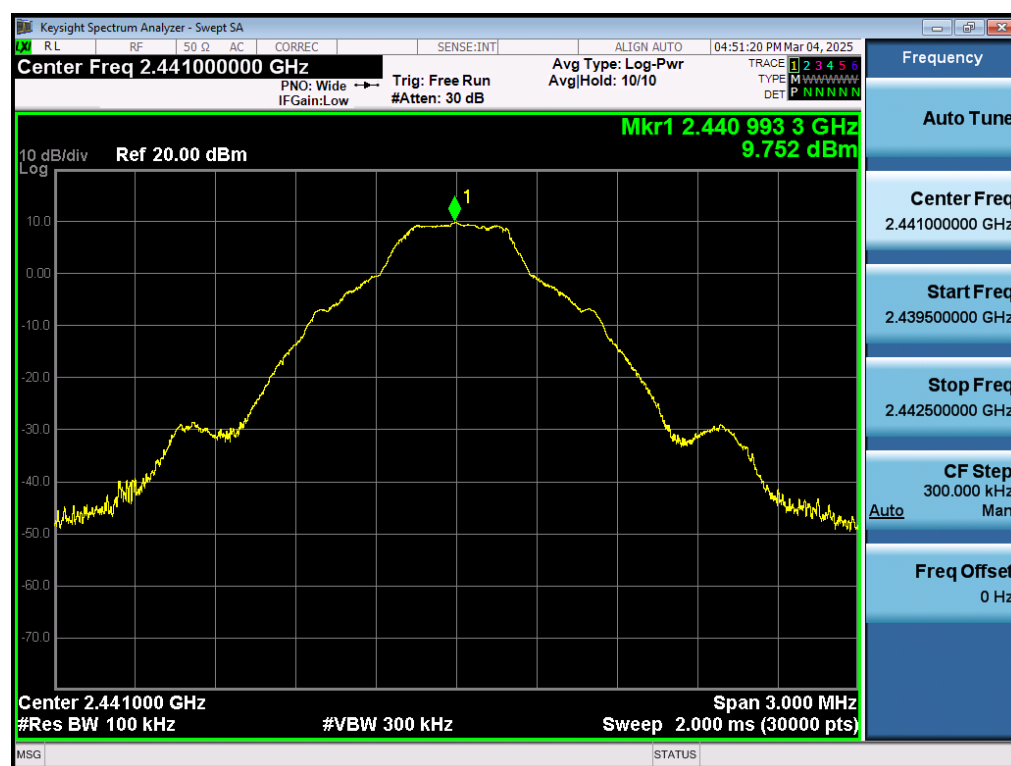
Test_Graph_BR_ANT1_2441_1Mbps_Reference Level
