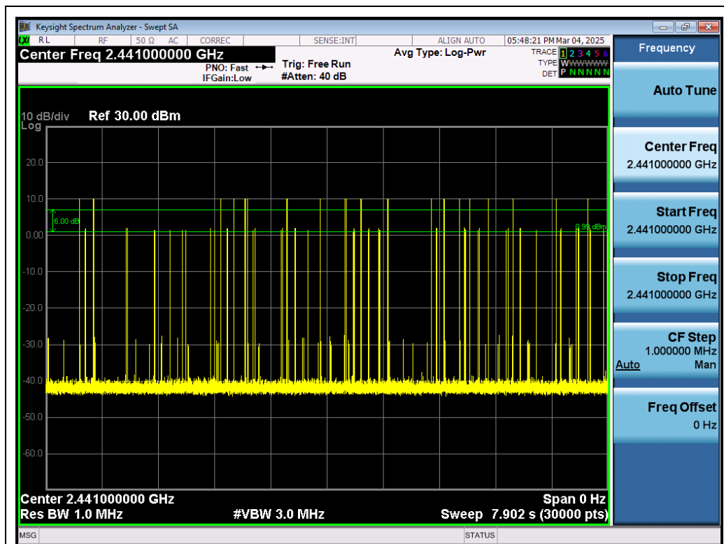
Test_Graph_BR_HOP_ANT1_NA_1Mbps_2441_Number of Busrt
