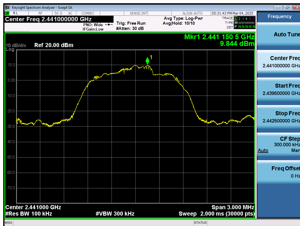
Test_Graph_EDR_ANT1_2441_3Mbps_Reference Level
