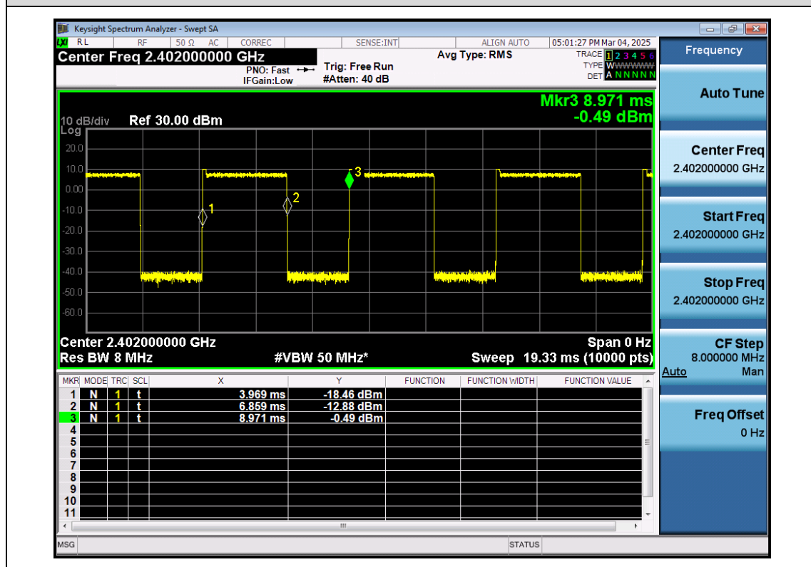
EDR- \pi /4-DQPSK-ANT1-2402
