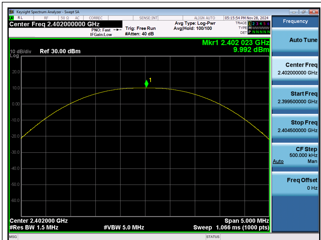
Test_Graph_BR_ANT1_2402_1Mbps_Peak Power
