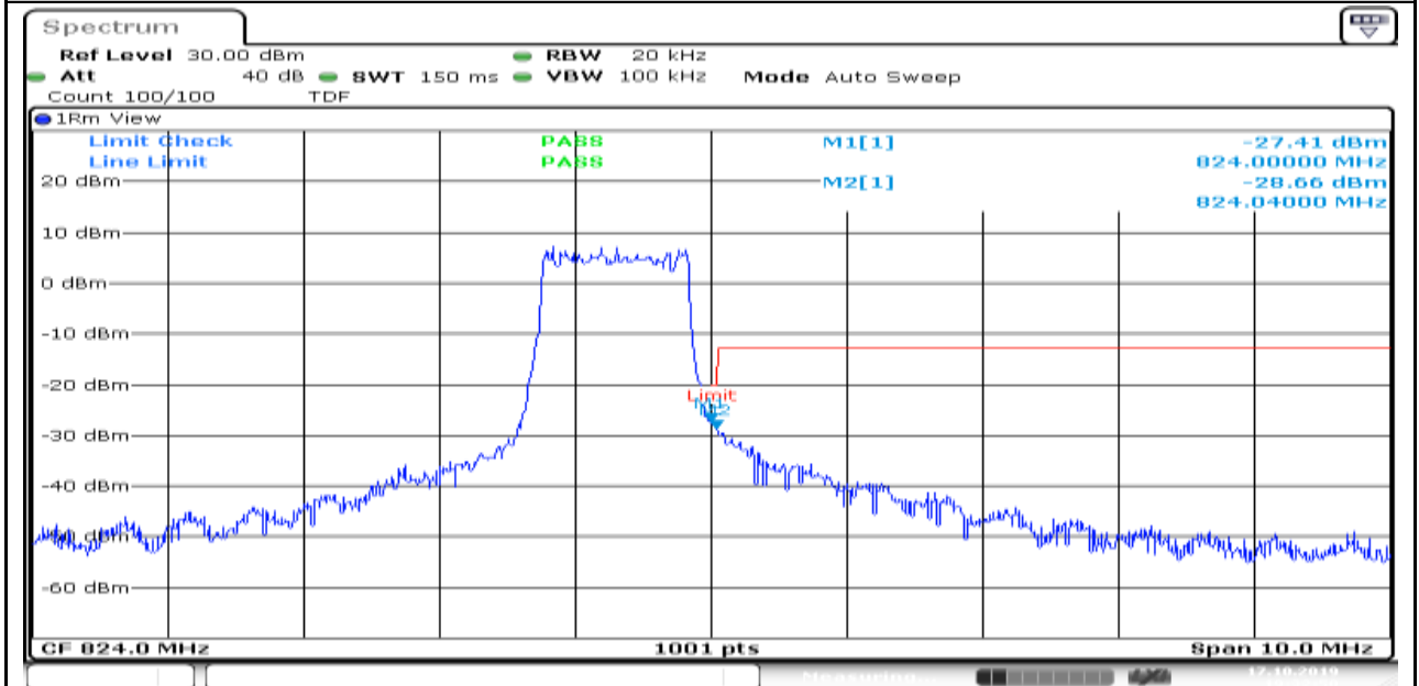
Band26_1.4MHz_16QAM_26783_6_0_Low
