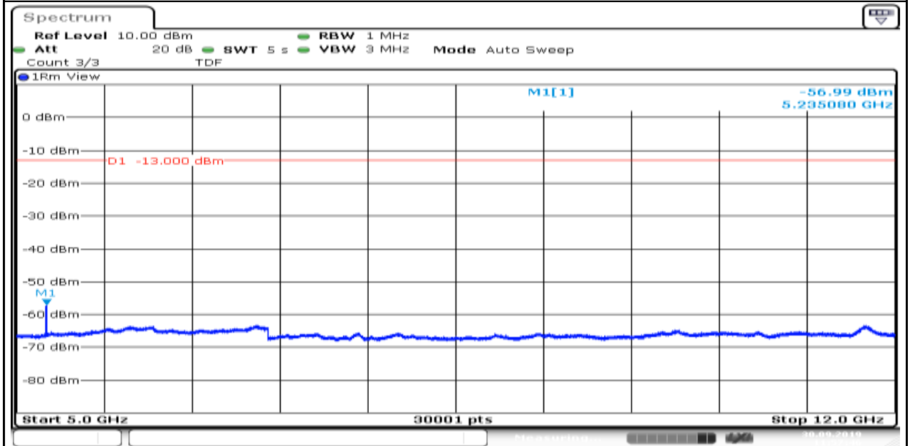
Band66_1.4MHz_16QAM_132322_6
