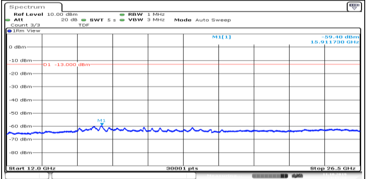
Band26_1.4MHz_QPSK_26783_1_5_Low_12000_26500
