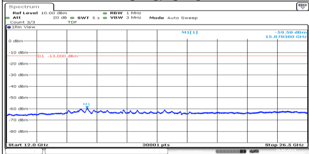
Band66_1.4MHz_QPSK_131979_1
