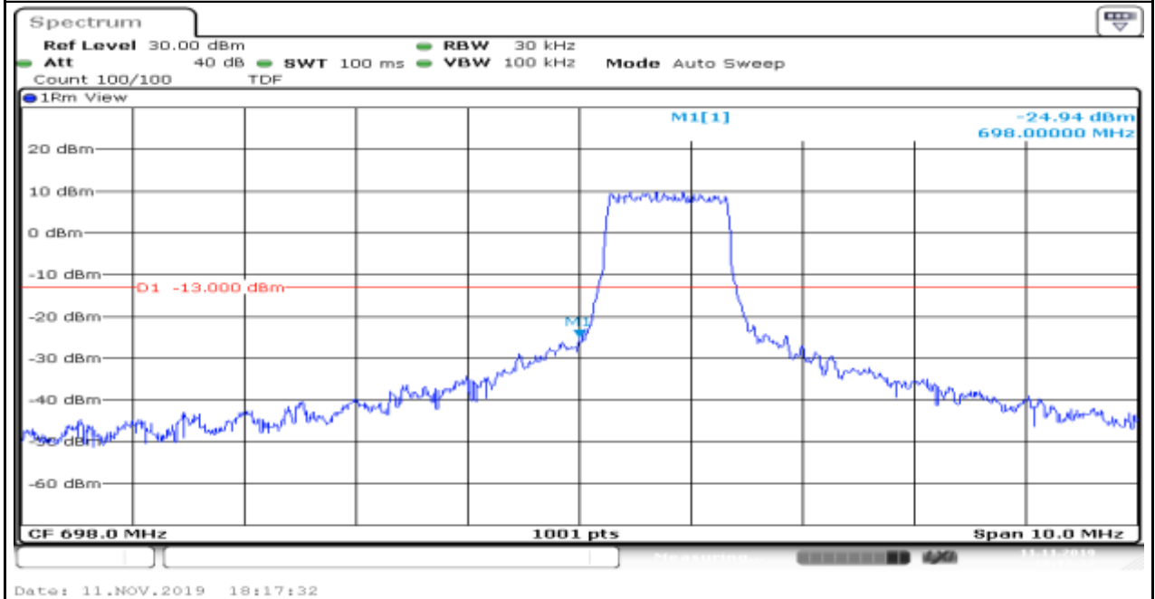
Band85_5MHz_16QAM_134027_1_0_Low
