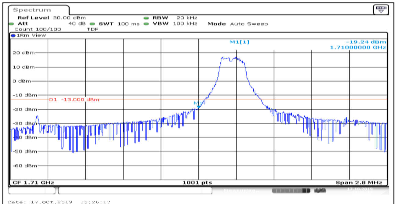
Band66_1.4MHz_16QAM_132665_6_0_Low
