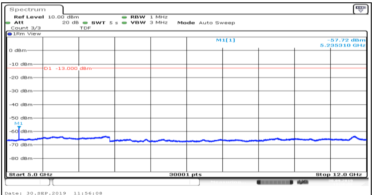
Band66_1.4MHz_QPSK_132322_6
