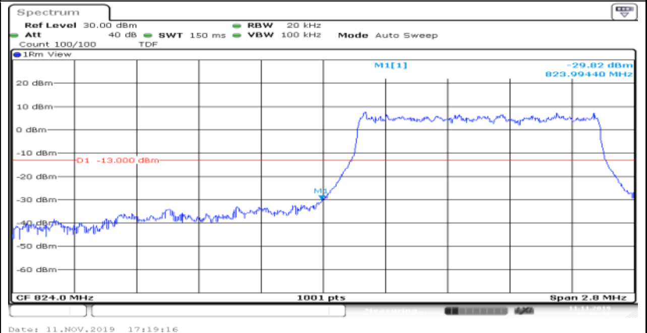
Band26_1.4MHz_16QAM_26797_1_0_Low
