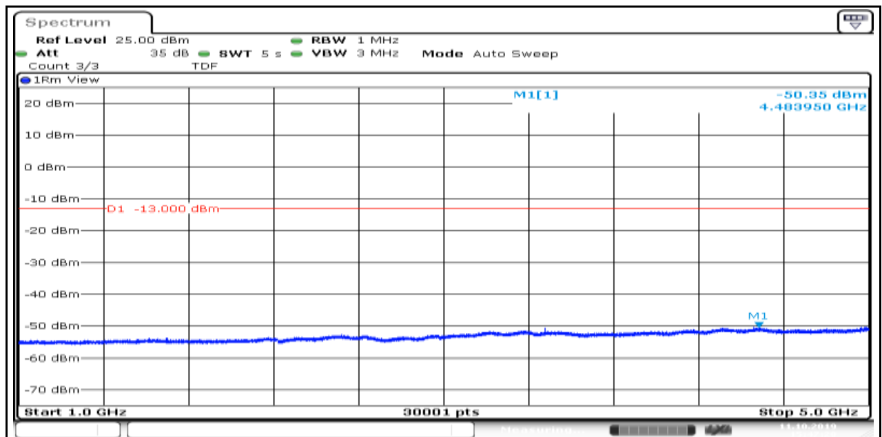
Band26_1.4MHz_QPSK_27033_1_5_Low_5000_12000
