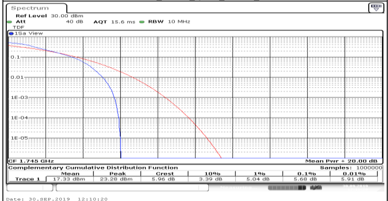
Band66_5MHz_QPSK_132322_6
