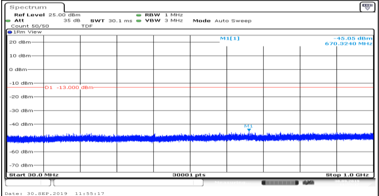
Band66_1.4MHz_QPSK_132665_1
