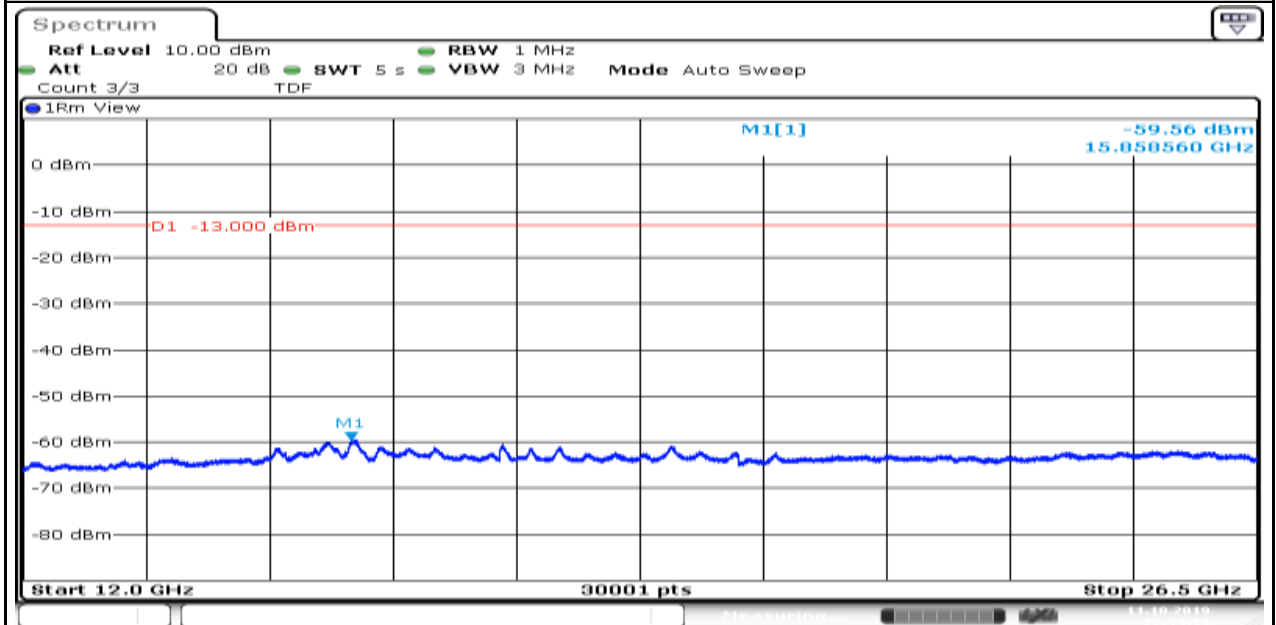
Band26_1.4MHz_QPSK_27033_1_5_Low_12000_26500
