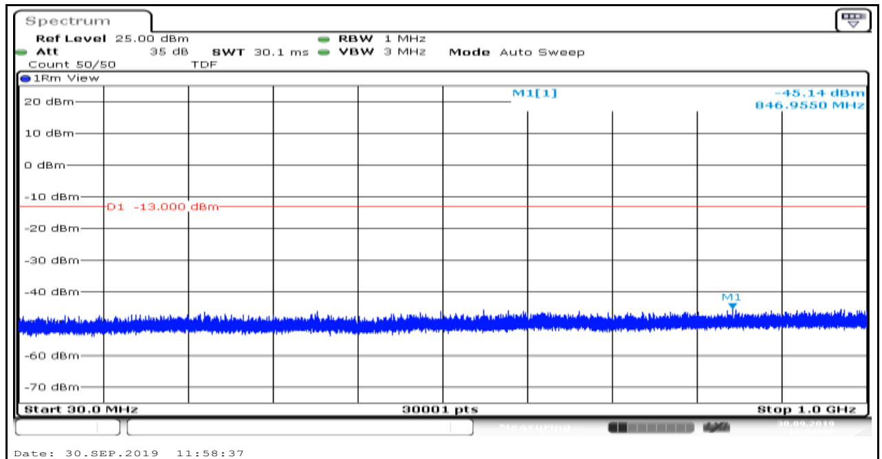
Band66_1.4MHz_QPSK_132665_6
