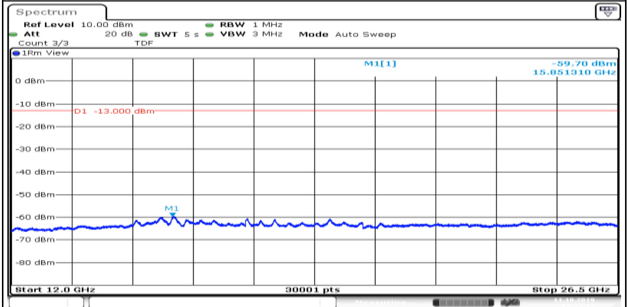
Band26_1.4MHz_QPSK_26797_1_0_Low_12000_26500
