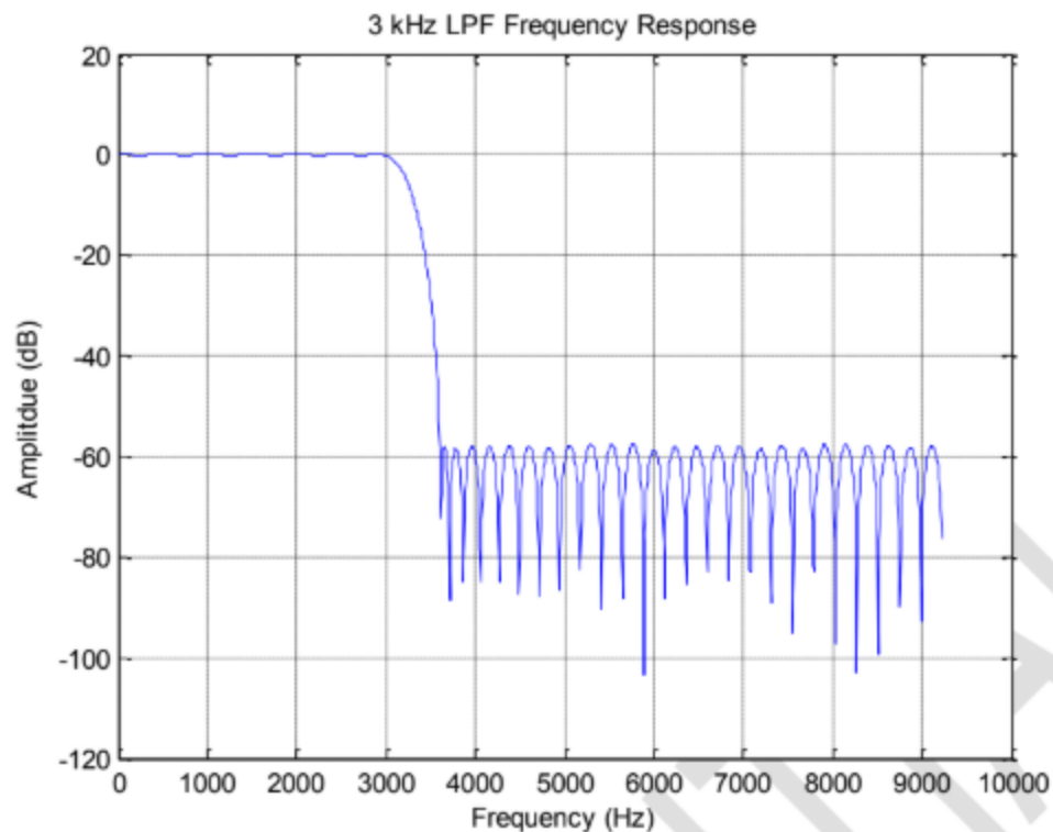
Figure 10. Frequency Response of Low Pass Filter
