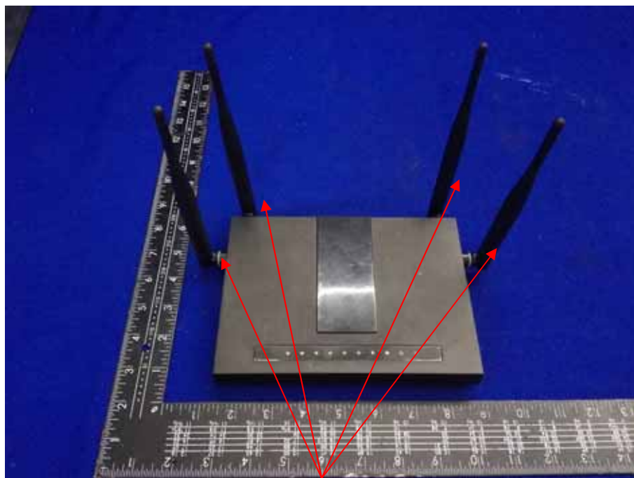
WIFI 2.4G+5G antenna
