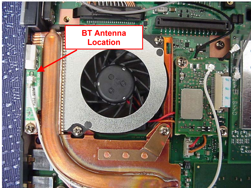
Bluetooth Antenna Location
