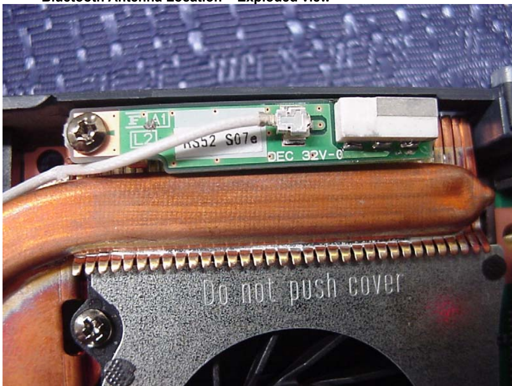
Bluetooth Antenna Location – Exploded view
