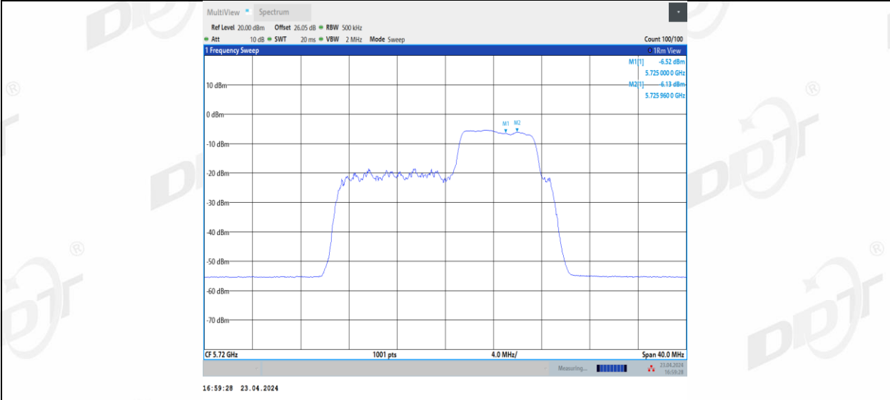
11BE20MIMO_Ant1_5720_UNII-3_106+26_1
