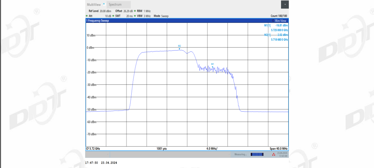
11BE20MIMO Ant3 5720 UNII-2C 106+26 2
