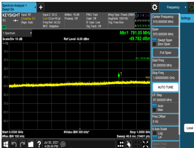
Plot 7-1107. Conducted Spurious Emission Plot 30 MHz to 1 GHz (B66_20M_1C_16QAM - Low Channel, Port 1)
