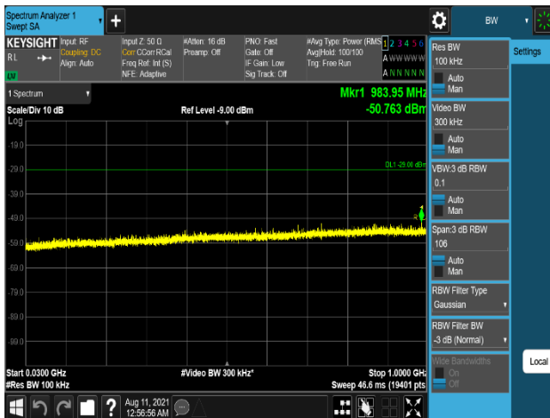
Plot 7-1071. Conducted Spurious Emission Plot 30 MHz to 1 GHz (B2_10M+20M_2C_QPSK - Port 2)
