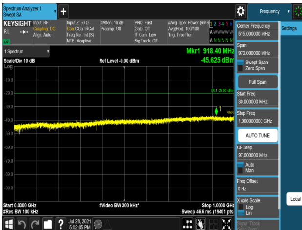
Plot 7-1089. Conducted Spurious Emission Plot 30 MHz to 1 GHz (B66_5M_1C_64QAM - Low Channel, Port 1)
