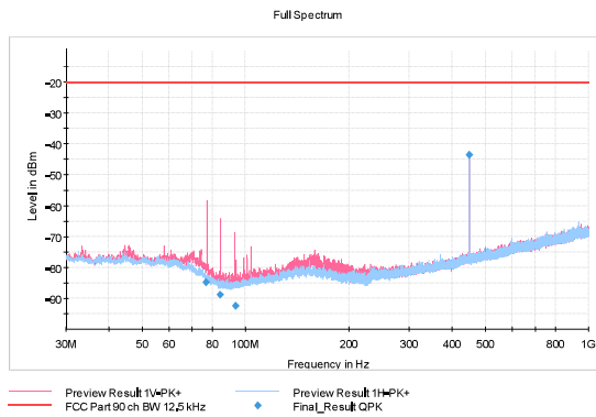
Figure 208: TX 450.5 MHz, 12.5 kHz, 9600 bps
