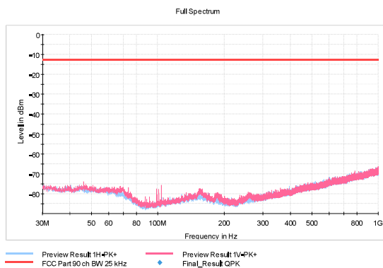
Figure 210: TX 469.5 MHz, 25 kHz, 4800 bps
