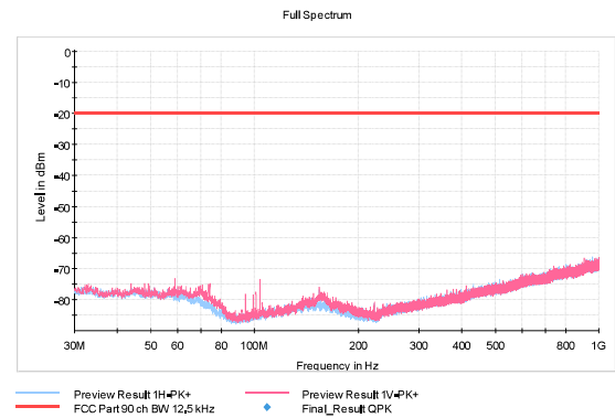
Figure 209: RX 450.5 MHz, 12.5 kHz, 9600 bps
