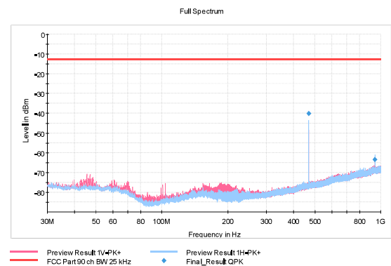
Figure 211: RX 469.5 MHz, 25 kHz, 4800 bps
