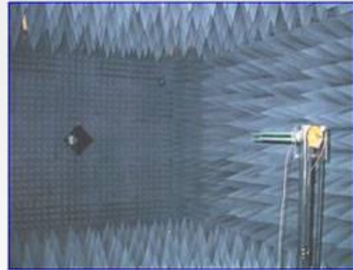
Figure 1b: A-Plus chamber setup
