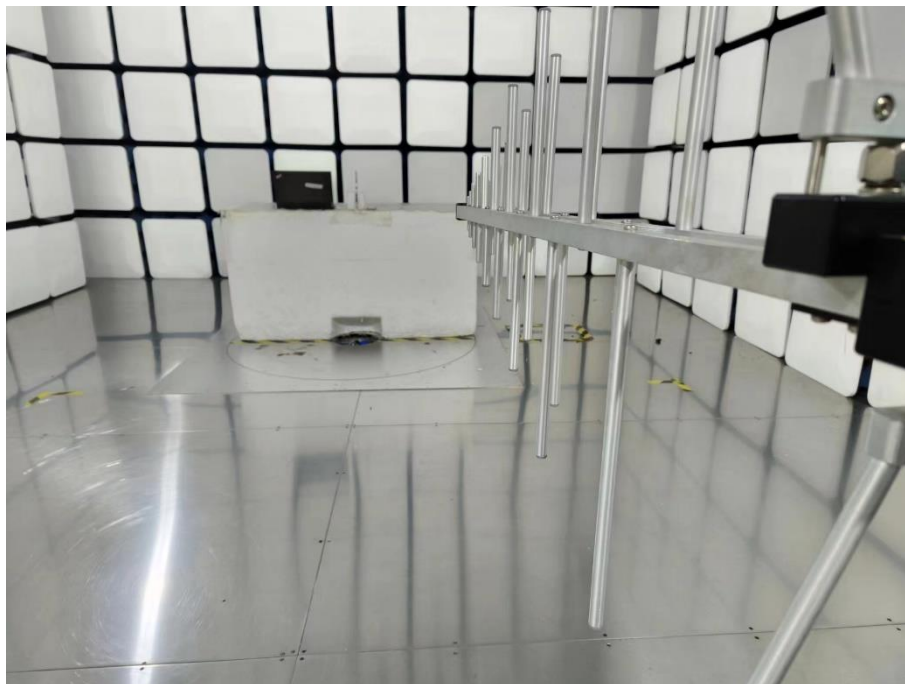
30MHz-1GHz-LoRa-2
