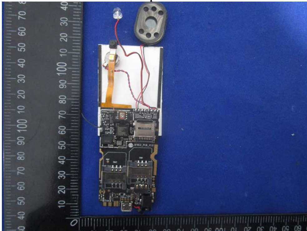
EUT –MB Top Unshield View
