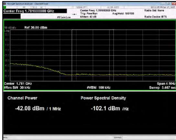
Band66 QPSK BW=20MHz Channel=132572 RB Size=1 Position=#0 Normal
