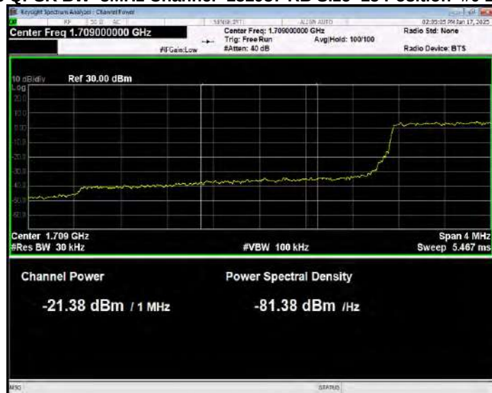
Band66 QPSK BW=3MHz Channel=131987 RB Size=15 Position=#0 Normal
