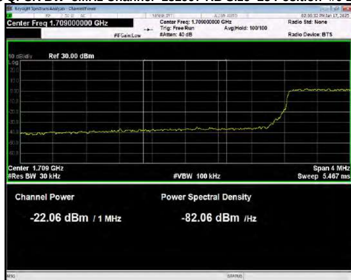
Band66 QPSK BW=5MHz Channel=131997 RB Size=25 Position=#0 Normal
