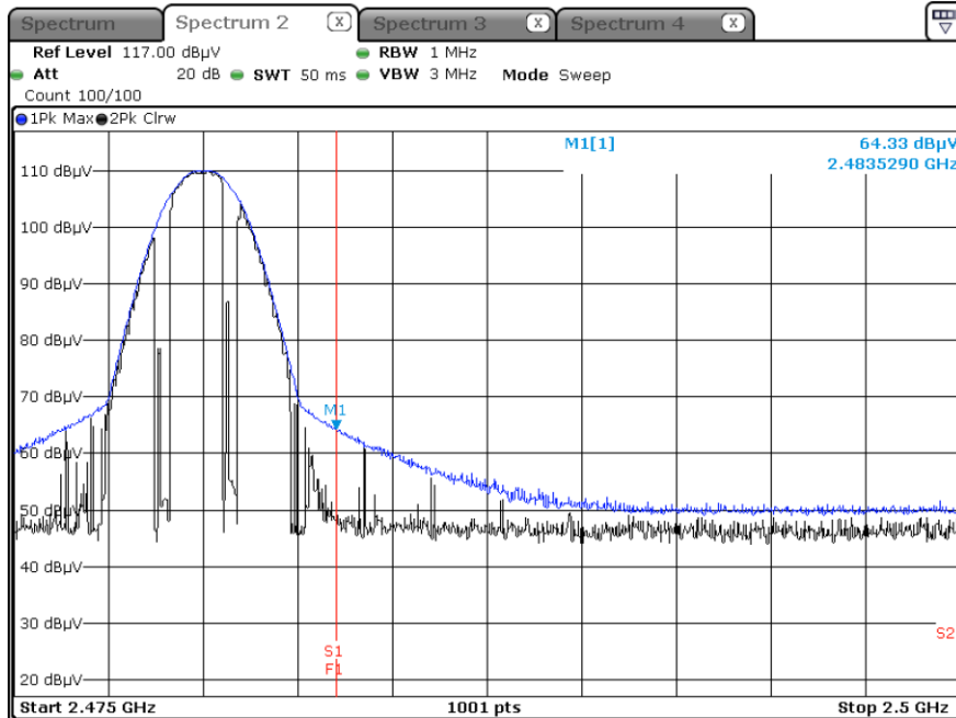
Radiated Restricted Band Edges plot – Peak & Average Result ( \pi/4 DQPSK, Ch.78, Z-V)
