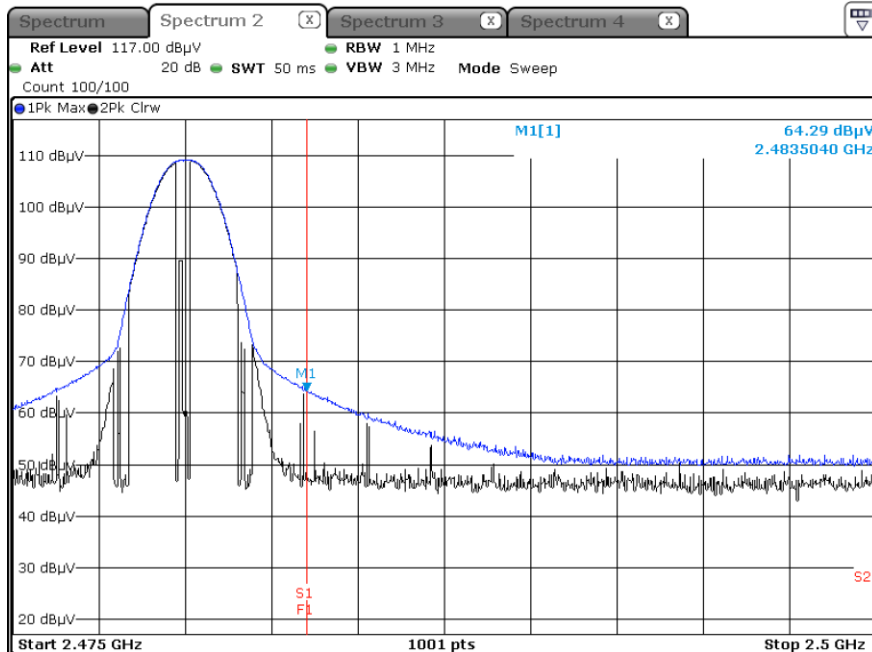
Radiated Restricted Band Edges plot – Peak &amp; Average Result (GFSK, Ch.78, Z-V)
