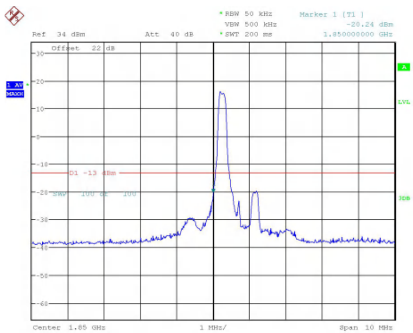
Band2-Low Channel-1.4MHz Bandwidth-1RB-16QAM
