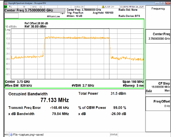
n78(3700-3800MHz) 80M DFT-s-OFDM 64QAM Outer_Full Mid
