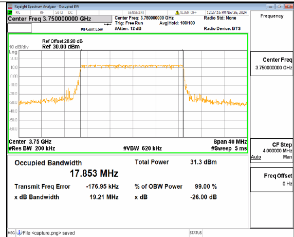
n78(3700-3800MHz) 20M DFT-s-OFDM 64QAM Outer_Full Mid
