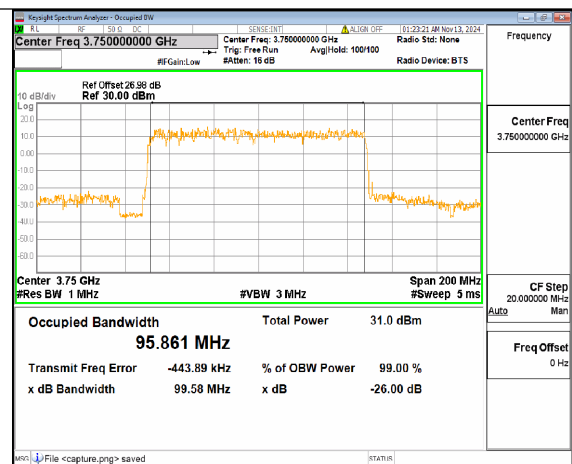
n78(3700-3800MHz) 100M DFT-s-OFDM QPSK Outer_Full Mid
