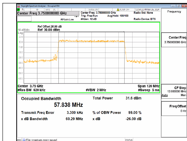
n78(3700-3800MHz) 60M DFT-s-OFDM 16QAM Outer_Full Mid
