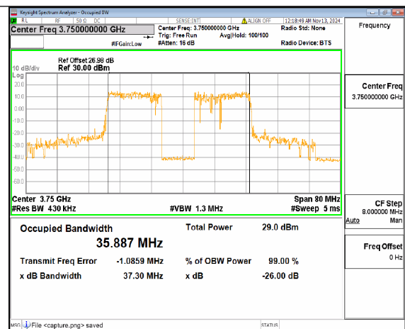
n78(3700-3800MHz) 40M DFT-s-OFDM QPSK Outer_Full Mid
