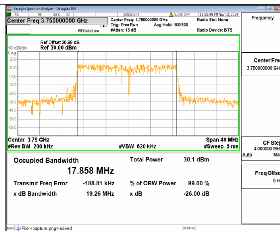
n78(3700-3800MHz) 20M DFT-s-OFDM QPSK Outer_Full Mid
