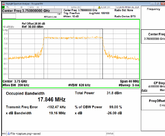
n78(3700-3800MHz) 20M DFT-s-OFDM 16QAM Outer_Full Mid
