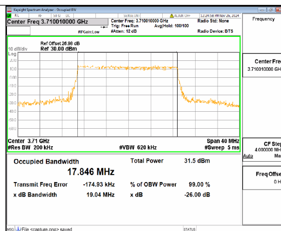
n78(3700-3800MHz) 20M DFT-s-OFDM 64QAM Outer_Full Low
