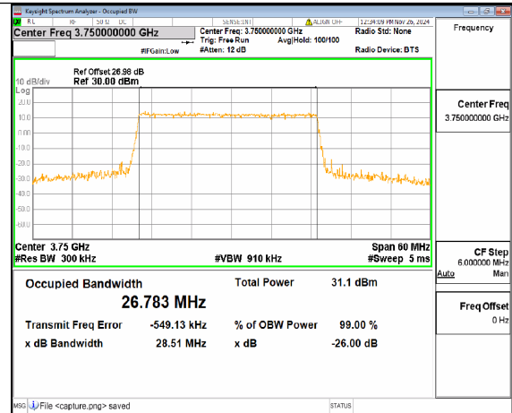
n78(3700-3800MHz) 30M DFT-s-OFDM 64QAM Outer_Full Mid
