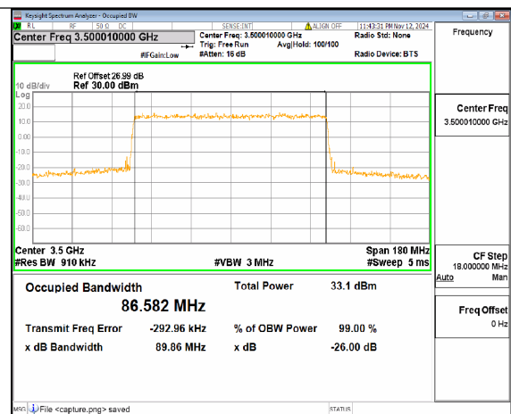
n78(3450-3550MHz) 90M DFT-s-OFDM QPSK Outer_Full Mid
