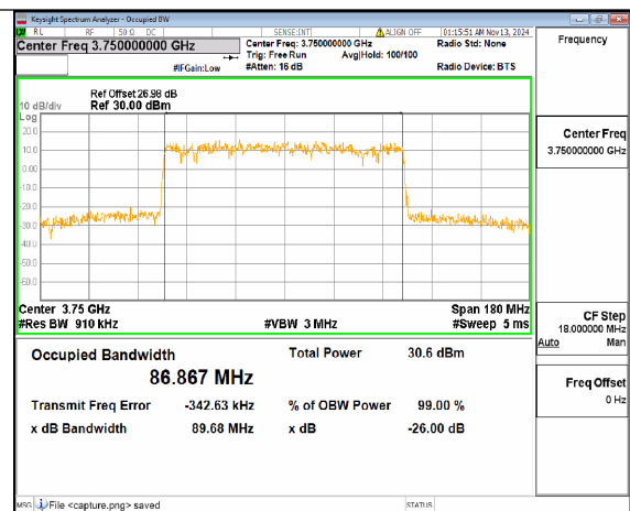
n78(3700-3800MHz) 90M DFT-s-OFDM QPSK Outer_Full Mid
