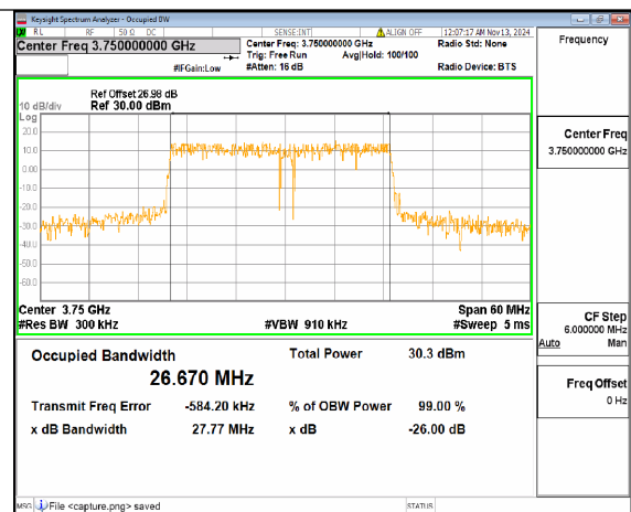
n78(3700-3800MHz) 30M DFT-s-OFDM QPSK Outer_Full Mid
