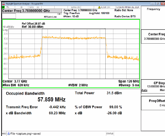
n78(3700-3800MHz) 60M DFT-s-OFDM 16QAM Outer_Full High
