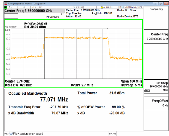
n78(3700-3800MHz) 80M DFT-s-OFDM 64QAM Outer_Full High
