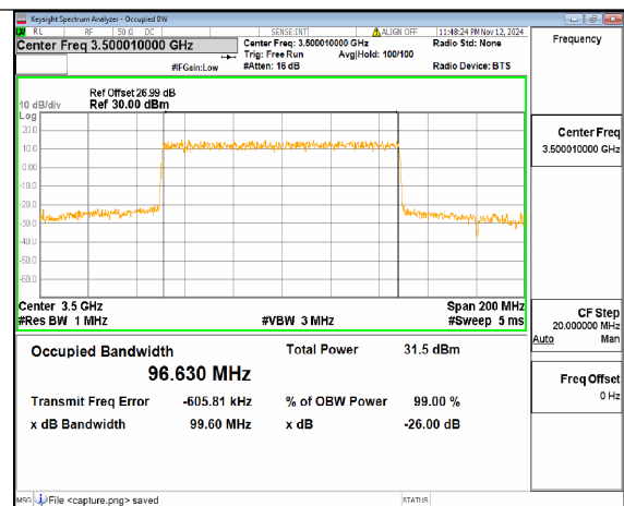
n78(3450-3550MHz) 100M DFT-s-OFDM QPSK Outer_Full Mid
