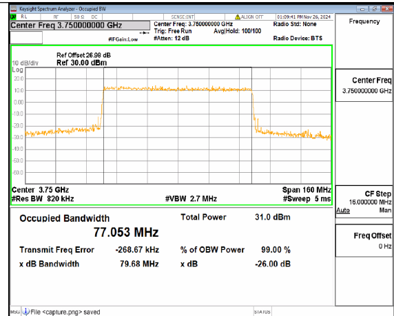
n78(3700-3800MHz) 80M CP-OFDM QPSK Outer_Full Mid
