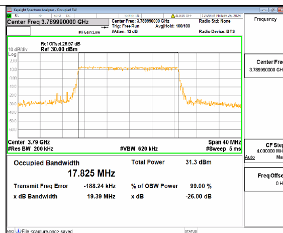
n78(3700-3800MHz) 20M DFT-s-OFDM 64QAM Outer_Full High
