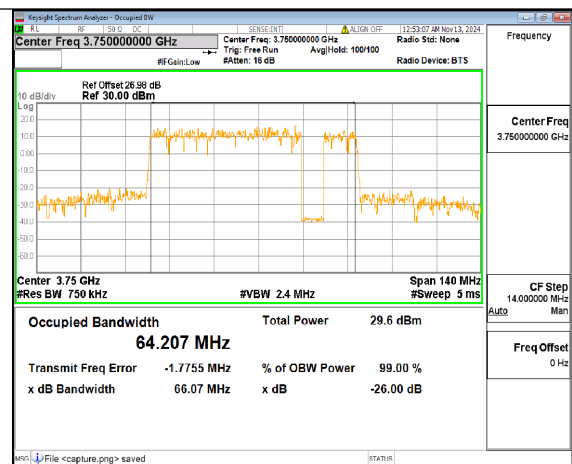
n78(3700-3800MHz) 70M DFT-s-OFDM QPSK Outer_Full Mid
