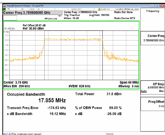
n78(3700-3800MHz) 20M DFT-s-OFDM 16QAM Outer_Full High
