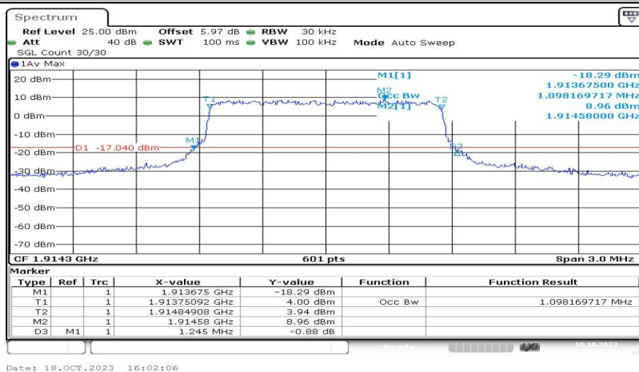
Band25-1.4MHz-QPSK-26683-6RB#0-PASS
