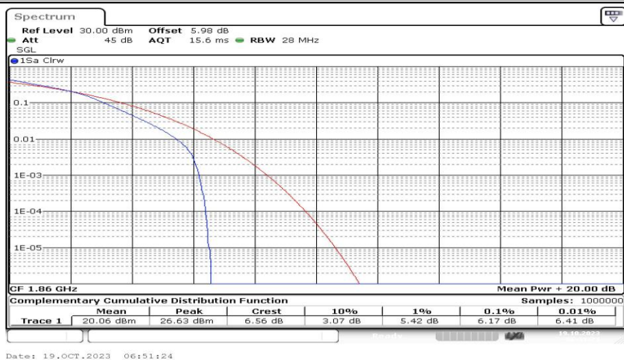
Band25-20MHz-16QAM-26140-25RB#0-PASS
