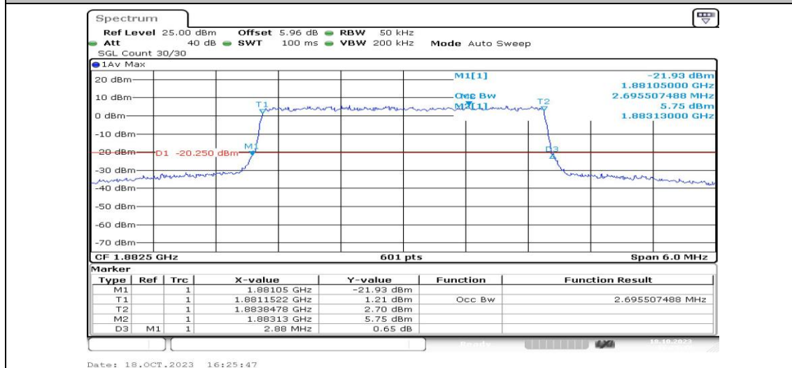
Band25-3MHz-16QAM-26365-15RB#0-PASS
