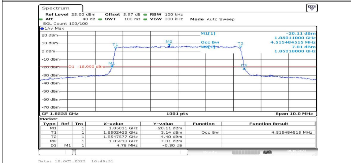
Band25-5MHz-16QAM-26065-25RB#0-PASS
