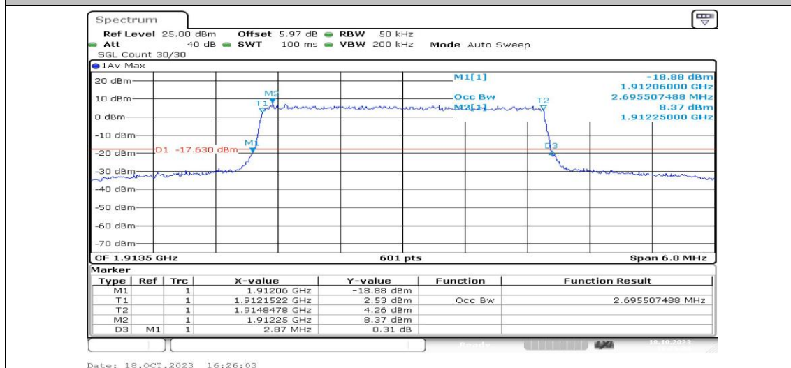
Band25-3MHz-QPSK-26675-15RB#0-PASS
