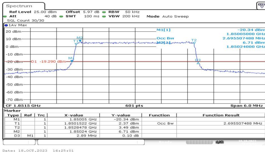
Band25-3MHz-QPSK-26055-15RB#0-PASS
