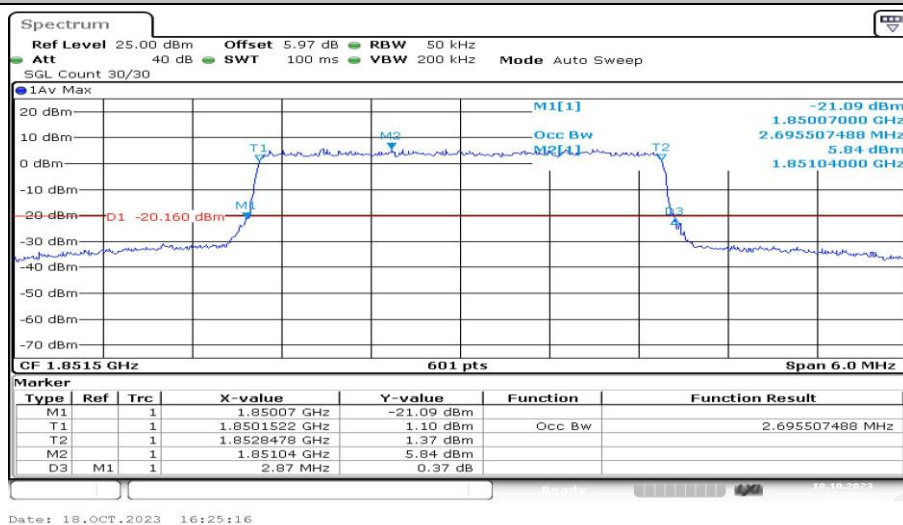
Band25-3MHz-16QAM-26055-15RB#0-PASS
