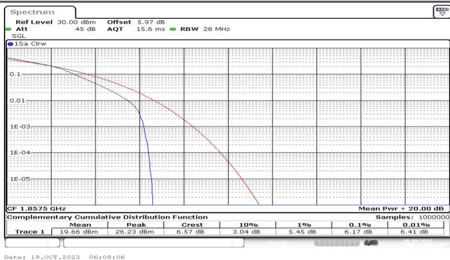
Band25-15MHz-16QAM-26115-25RB#0-PASS
