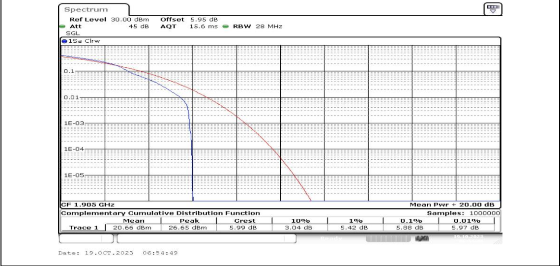
Band25-20MHz-16QAM-26590-1RB#0-PASS
