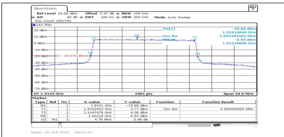
Band25-5MHz-16QAM-26665-25RB#0-PASS
