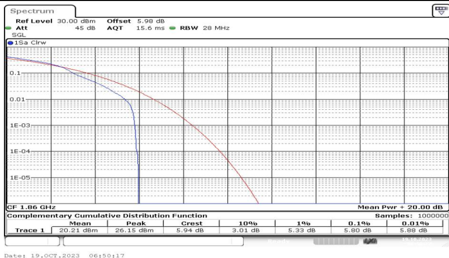
Band25-20MHz-16QAM-26140-1RB#0-PASS
