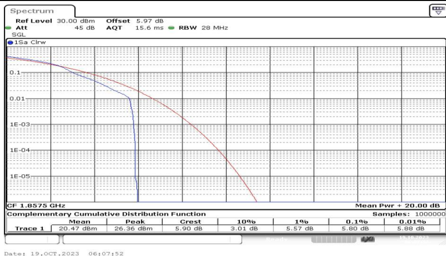
Band25-15MHz-16QAM-26115-1RB#0-PASS
