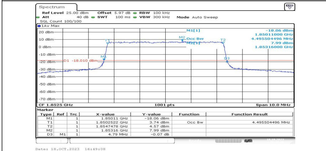
Band25-5MHz-QPSK-26065-25RB#0-PASS
