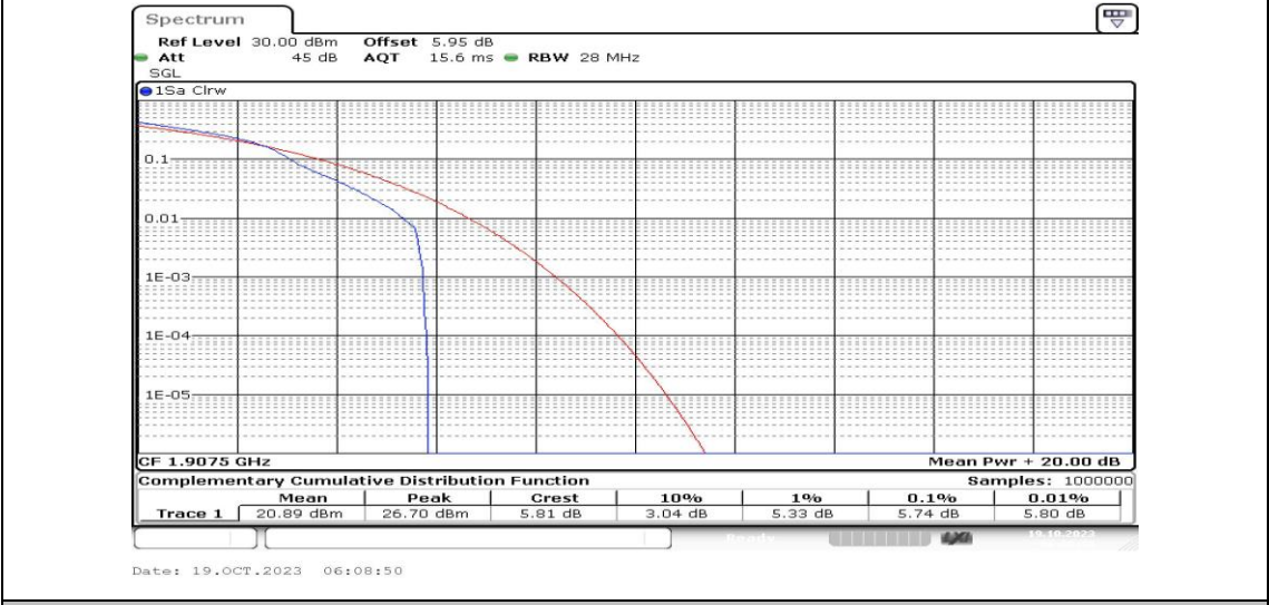
Band25-15MHz-16QAM-26615-1RB#0-PASS
