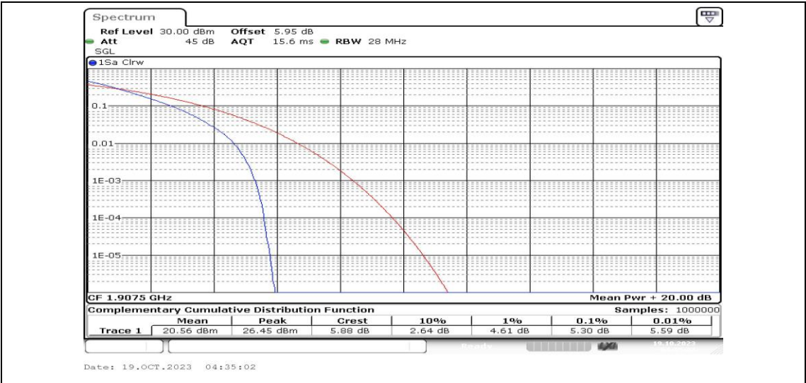
Band25-15MHz-QPSK-26615-75RB#0-PASS
