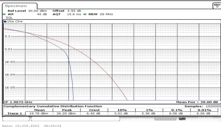
Band25-15MHz-16QAM-26615-25RB#0-PASS
