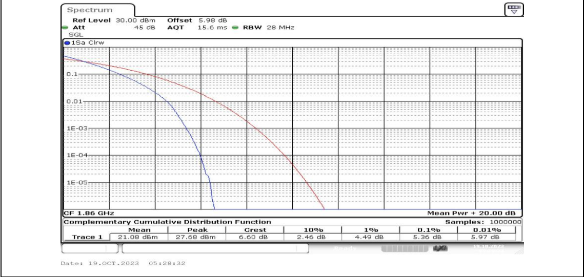
Band25-20MHz-QPSK-26140-100RB#0-PASS
