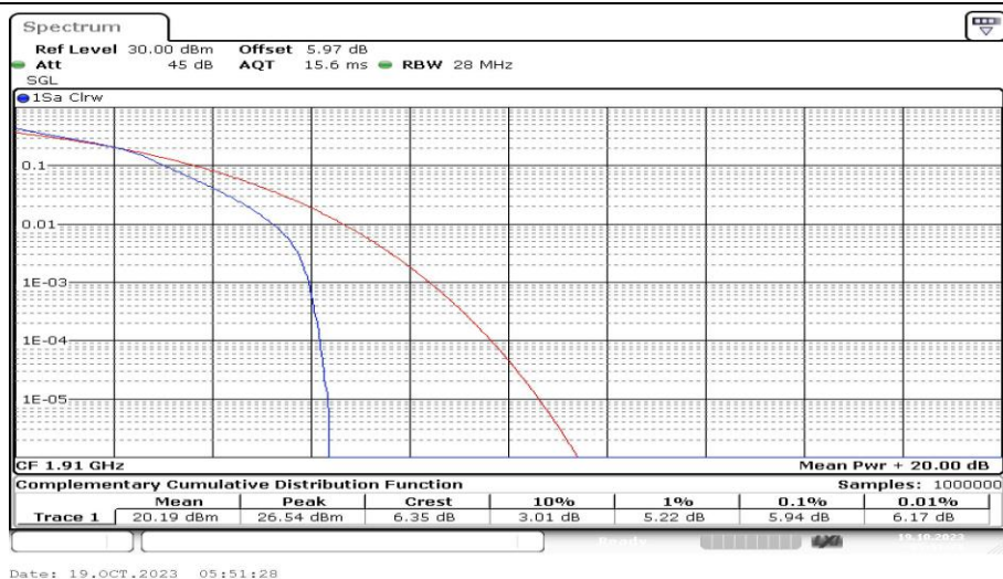
Band25-10MHz-16QAM-26640-25RB#0-PASS
