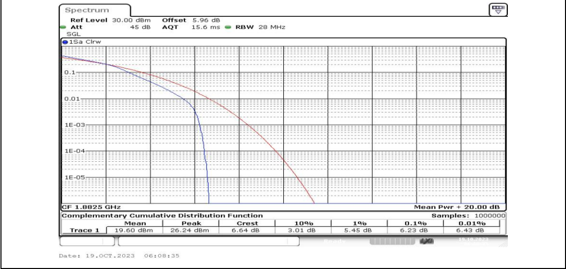
Band25-15MHz-16QAM-26365-25RB#0-PASS
