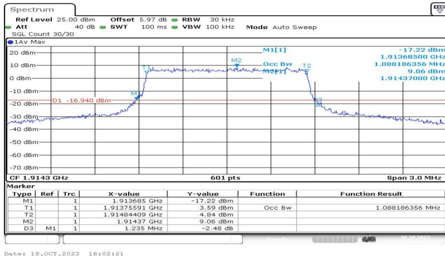
Band25-1.4MHz-16QAM-26683-6RB#0-PASS
