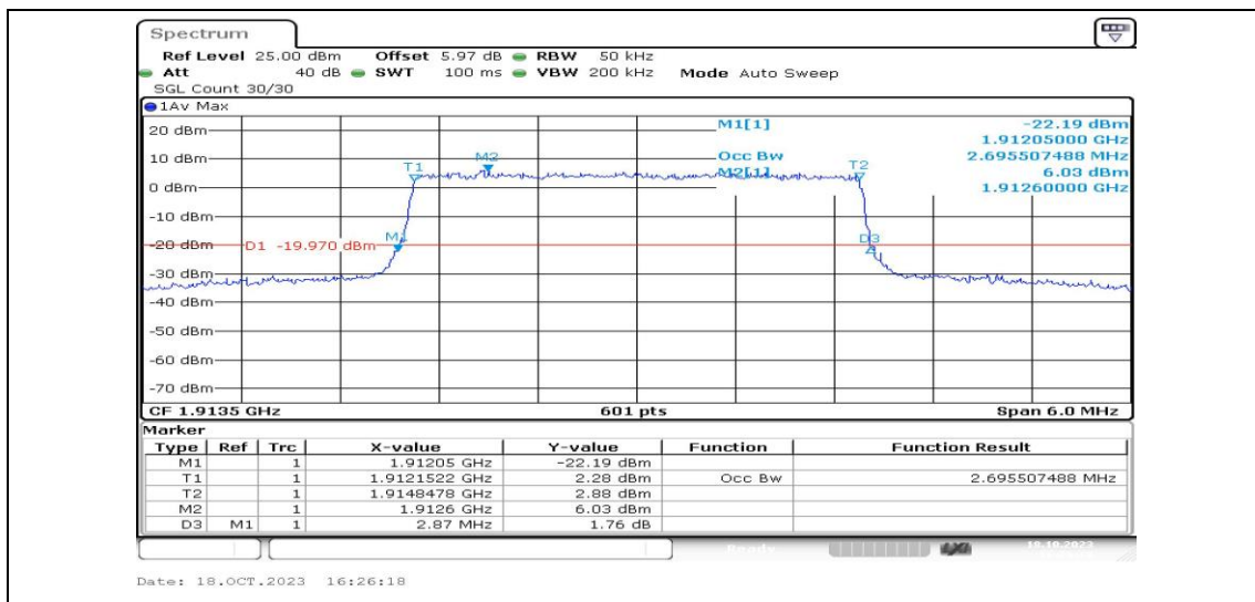
Band25-3MHz-16QAM-26675-15RB#0-PASS
