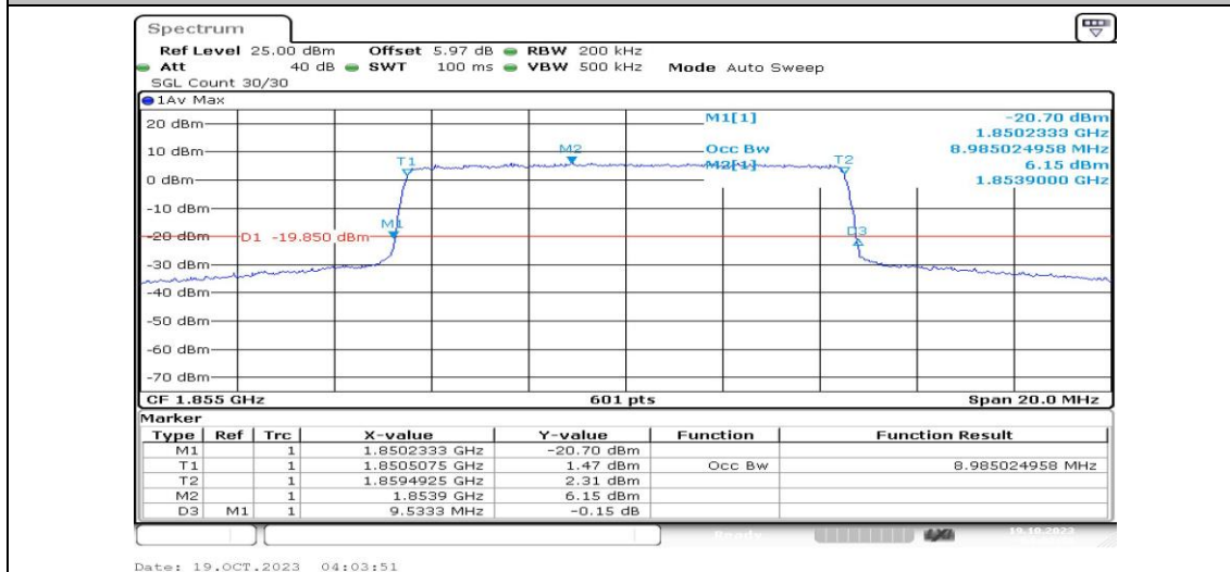
Band25-10MHz-QPSK-26090-50RB#0-PASS
