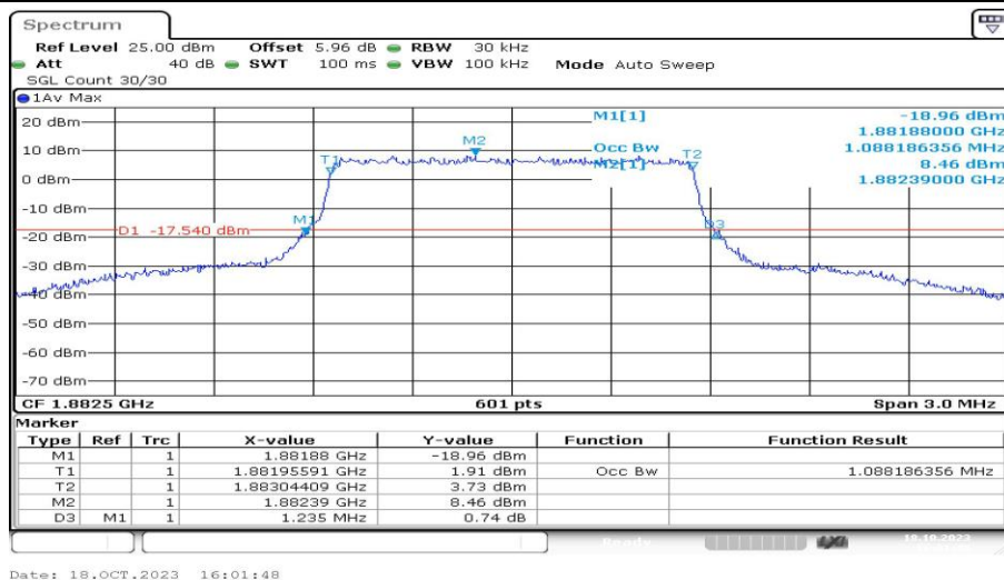
Band25-1.4MHz-16QAM-26365-6RB#0-PASS
