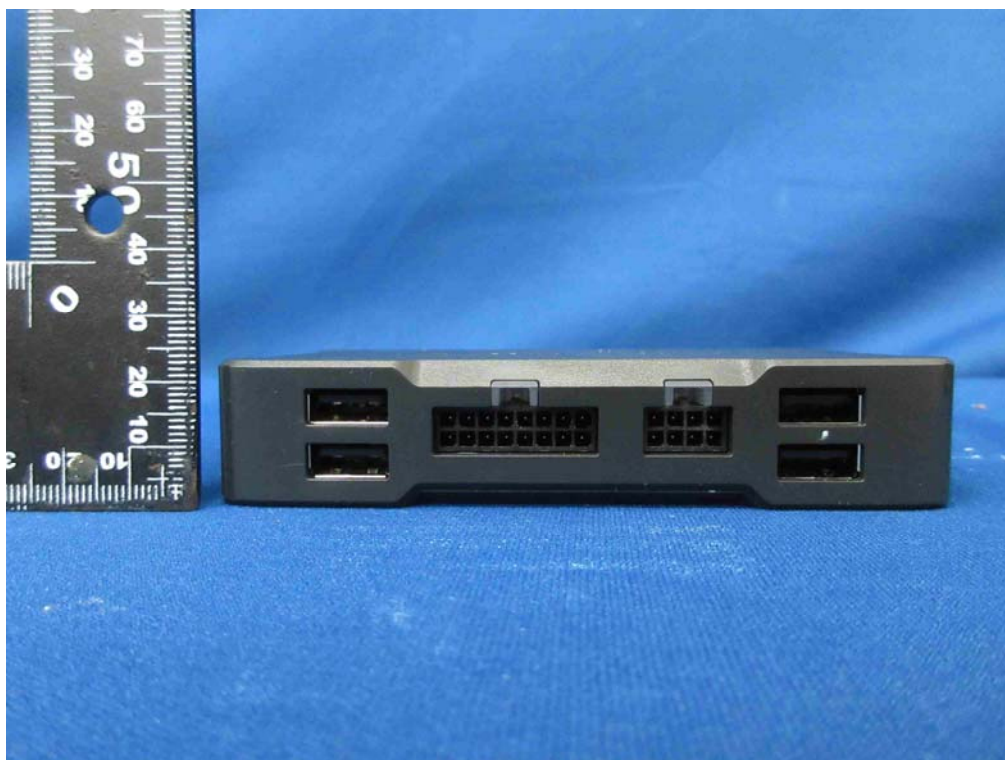
(12) EUT Photo (M/N: VG54-NAE)
